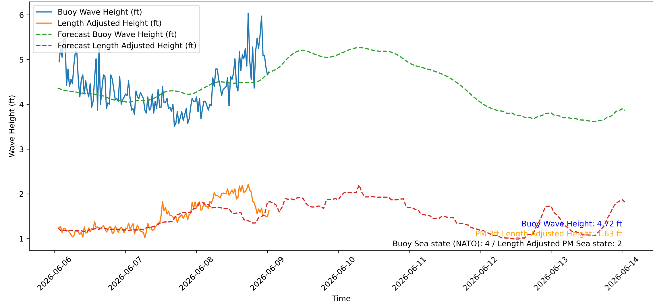
Wave Heights over Time for Oceanside Harbor at 2026-06-09 01:20:26
