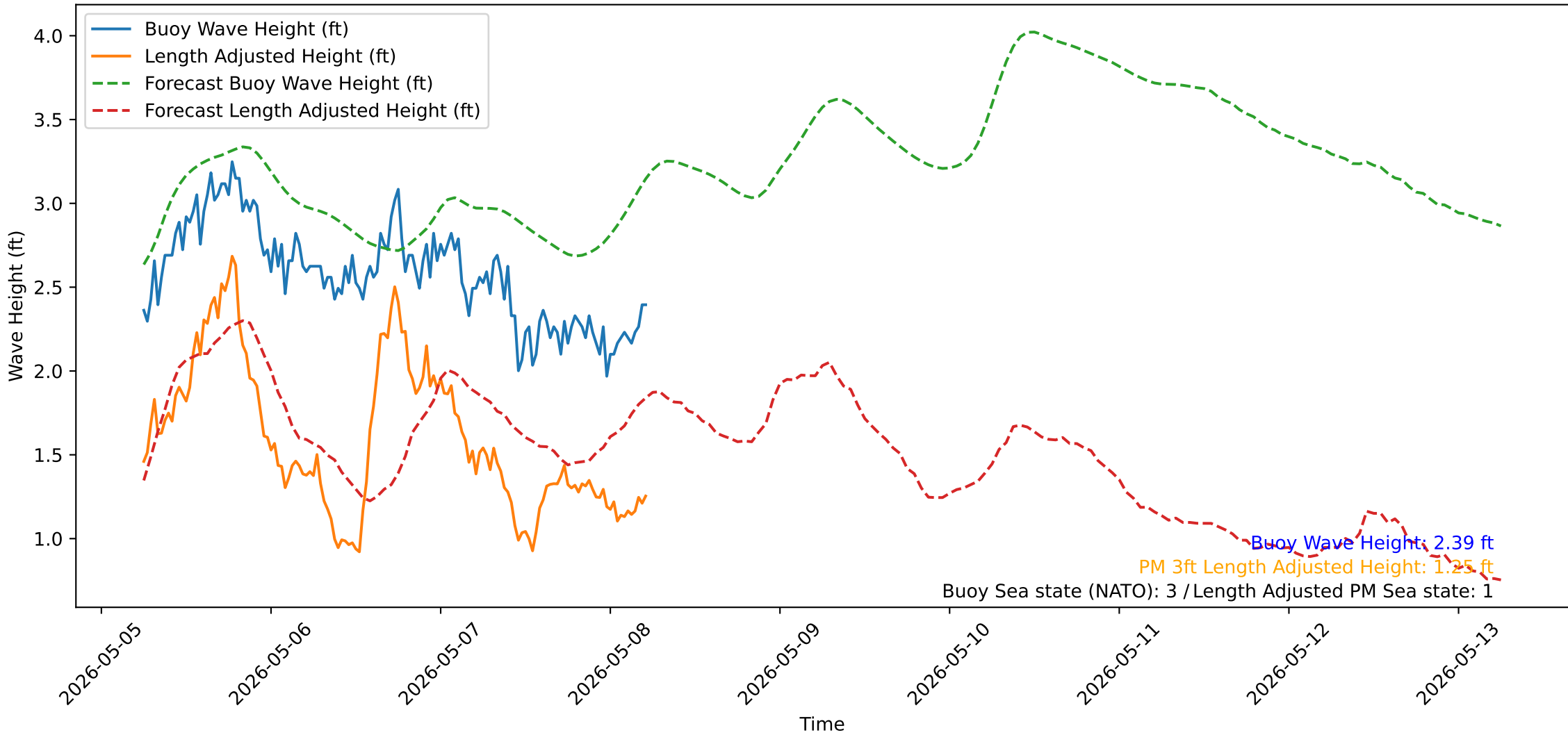
Wave Heights over Time for Oceanside Harbor at 2026-05-08 06:00:31
