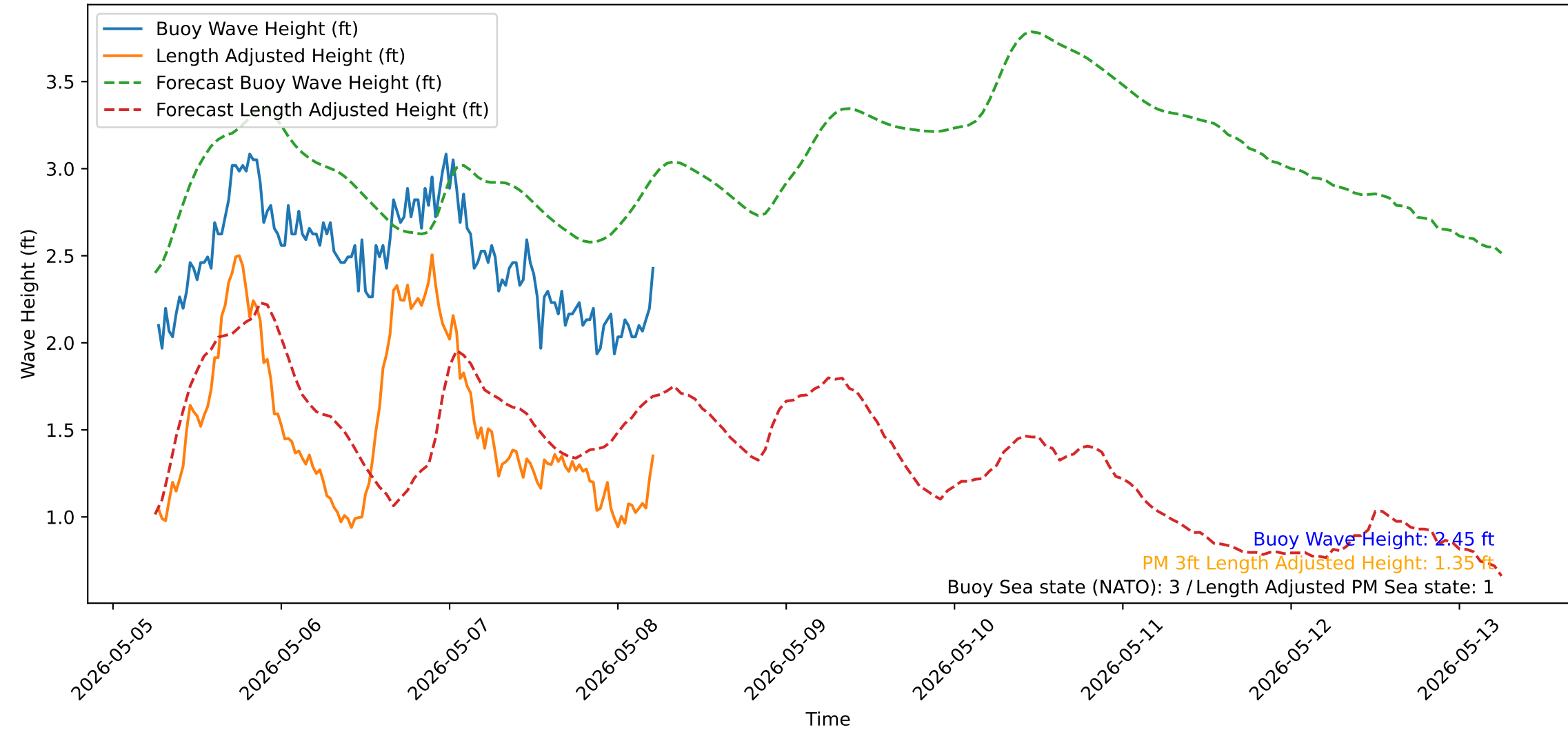
Wave Heights over Time for Red Beach at 2026-05-08 06:00:50
