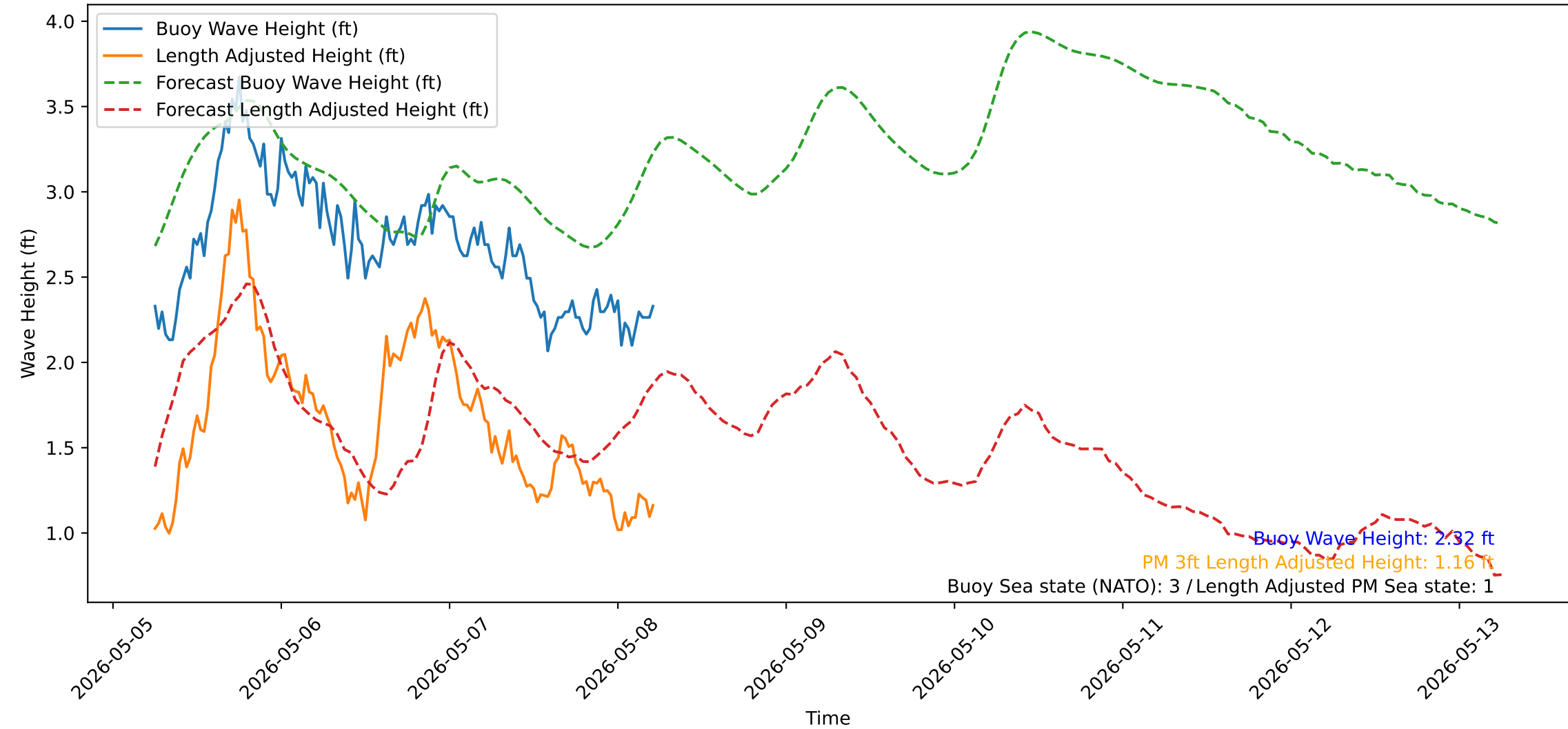
Wave Heights over Time for Green Beach at 2026-05-08 06:01:12
