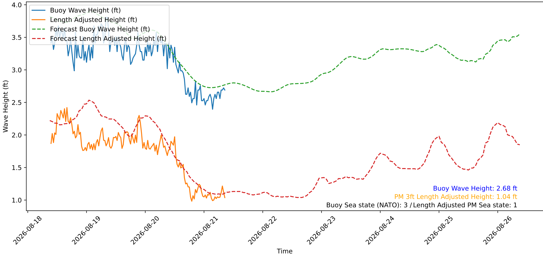
Wave Heights over Time for Oceanside Harbor at 2026-08-21 09:20:26
