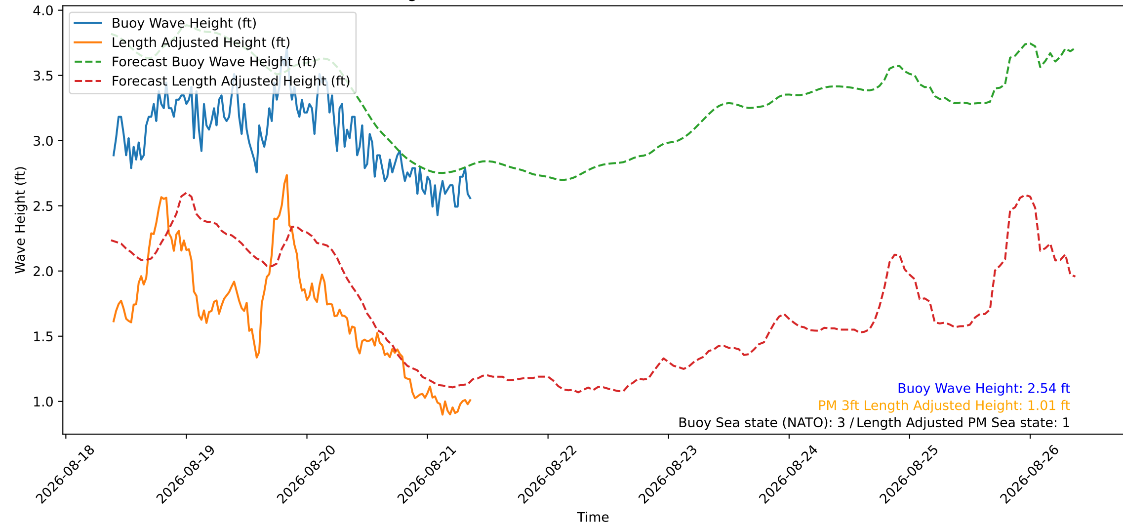
Wave Heights over Time for Green Beach at 2026-08-21 09:21:10
