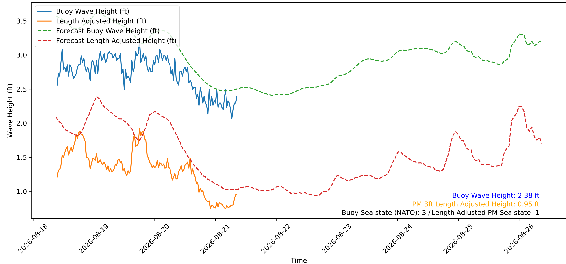
Wave Heights over Time for Red Beach at 2026-08-21 09:20:46
