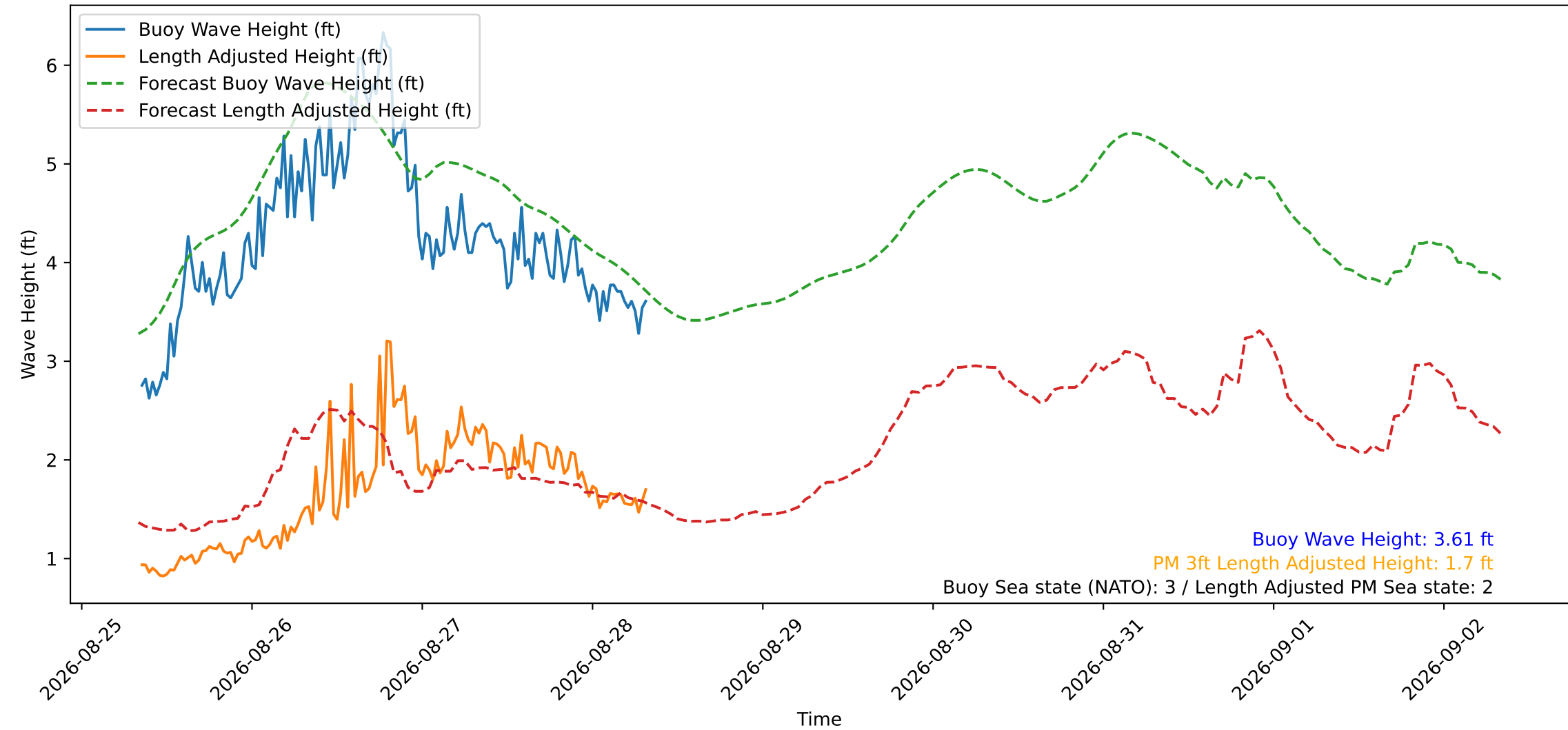
Wave Heights over Time for Green Beach at 2026-08-28 08:21:14
