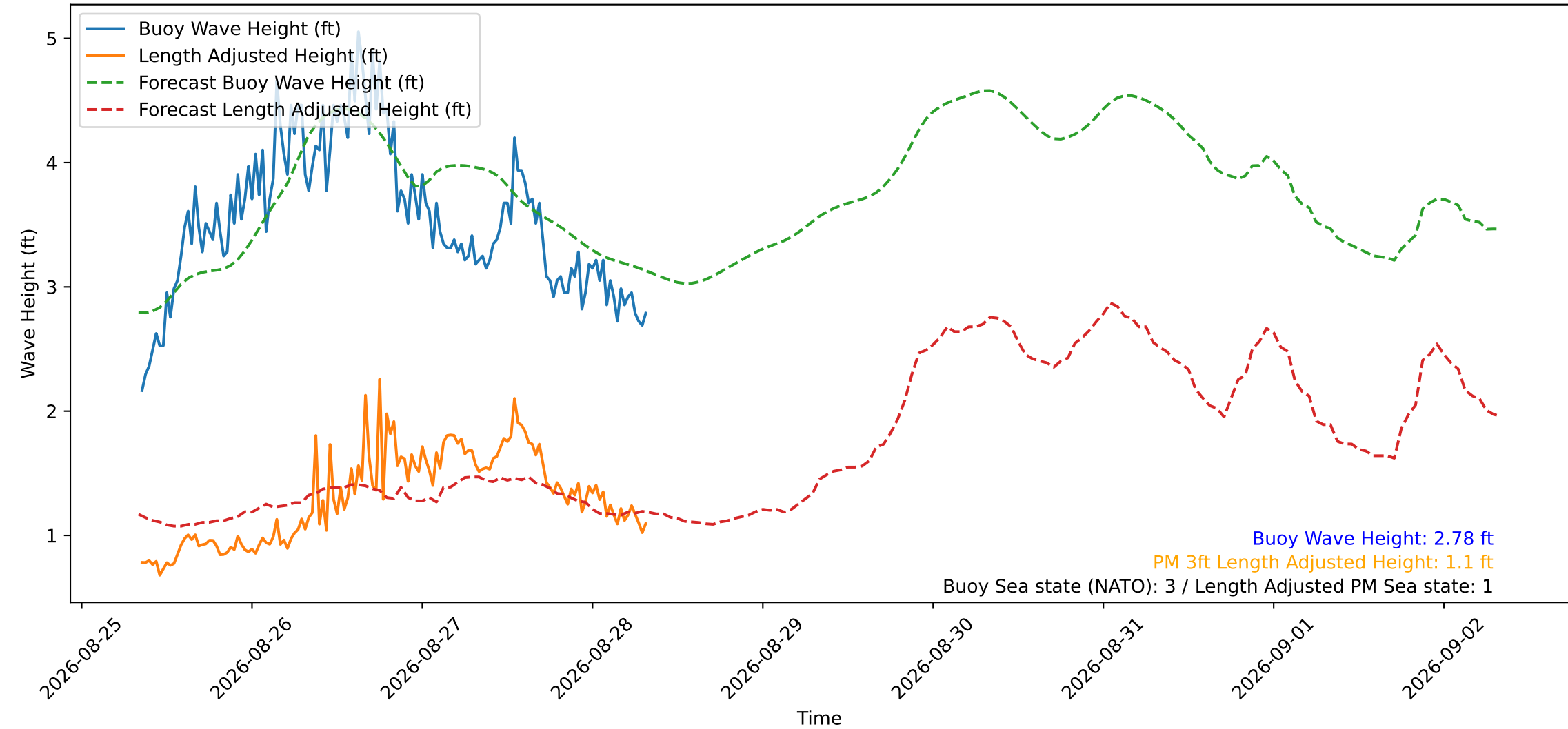
Wave Heights over Time for Red Beach at 2026-08-28 08:20:50
