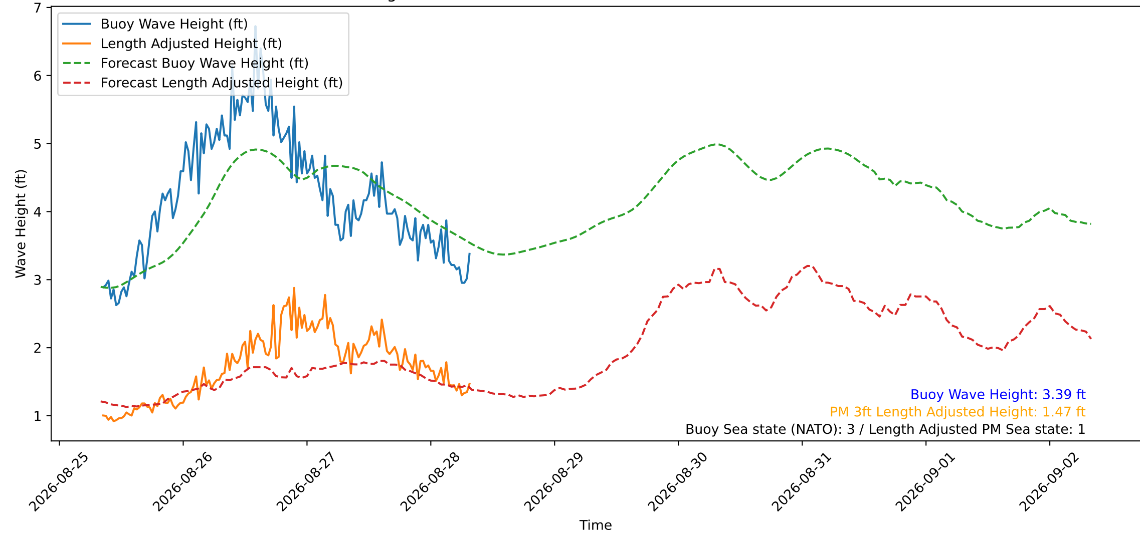
Wave Heights over Time for Oceanside Harbor at 2026-08-28 08:20:29
