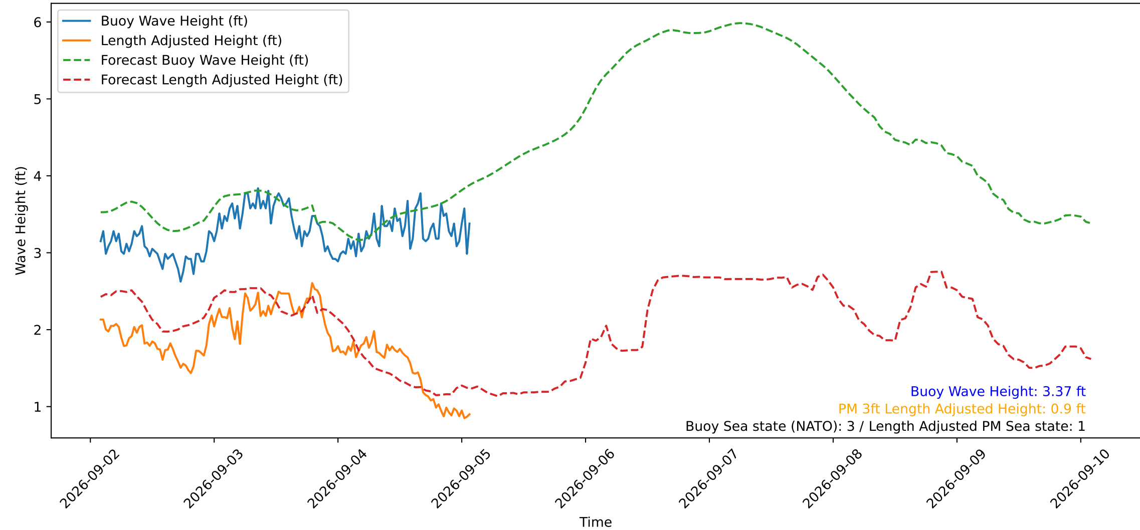
Wave Heights over Time for Oceanside Harbor at 2026-09-05 02:00:30
