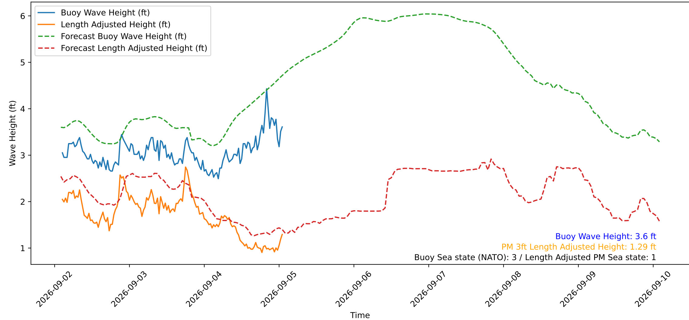
Wave Heights over Time for Green Beach at 2026-09-05 02:01:13
