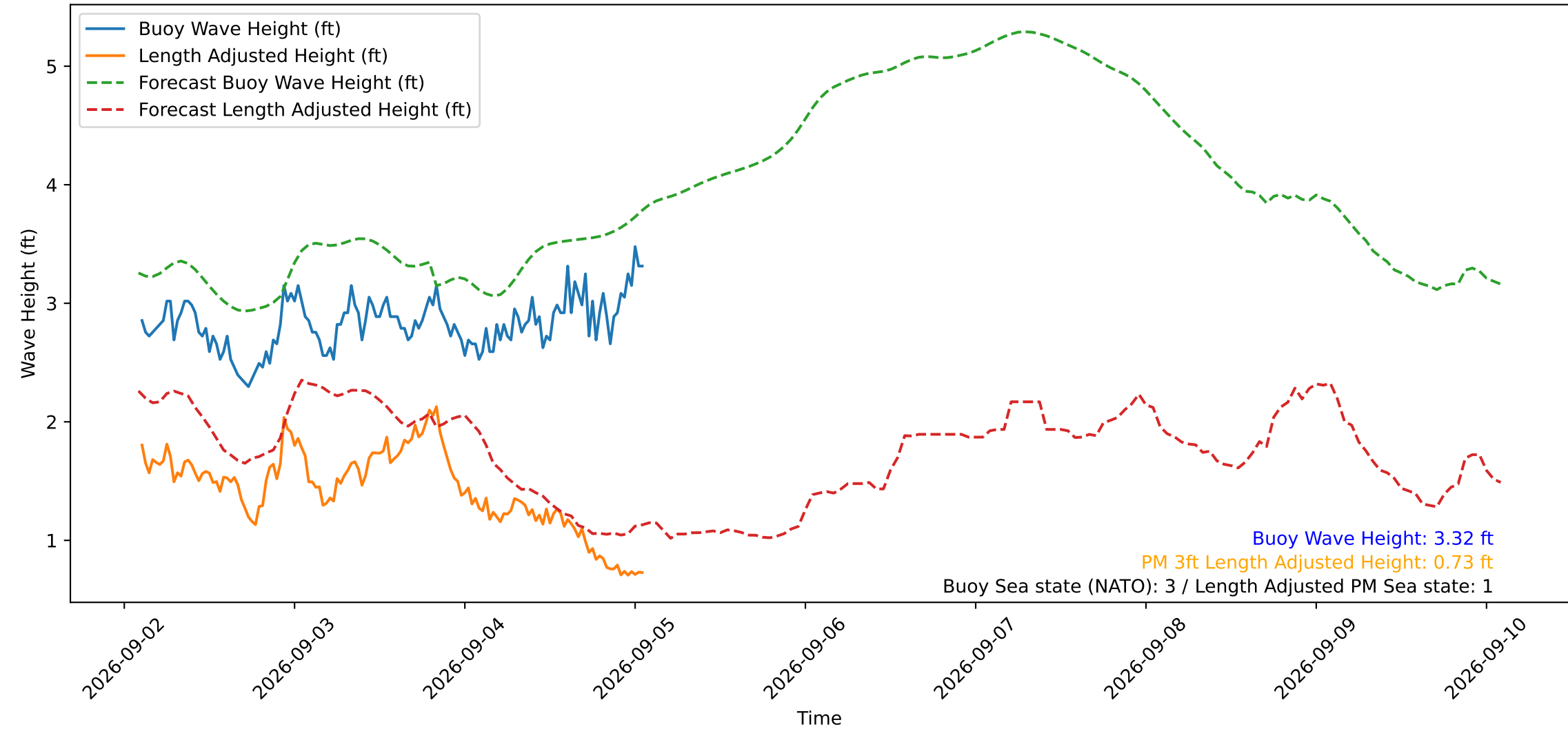
Wave Heights over Time for Red Beach at 2026-09-05 02:00:50
