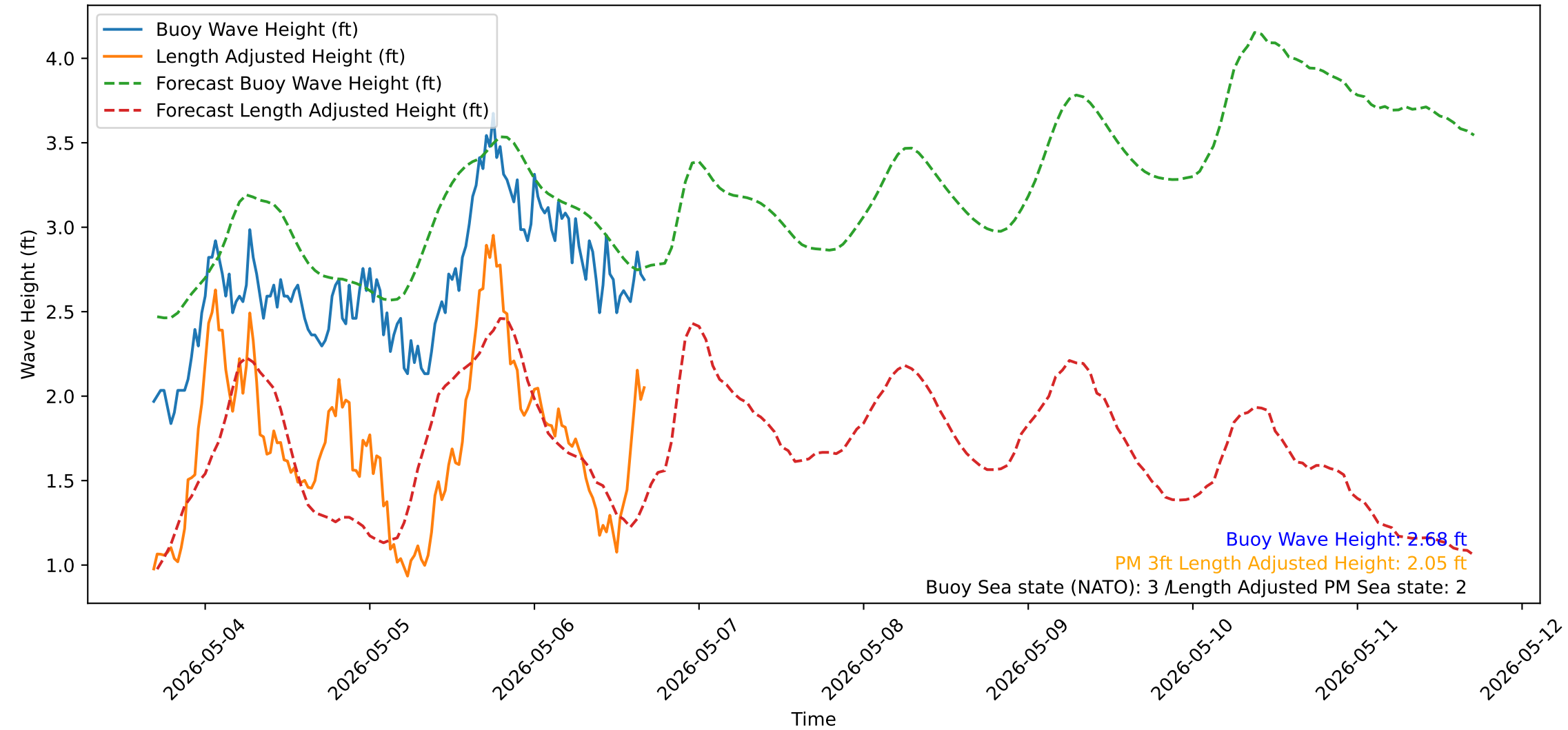
Wave Heights over Time for Green Beach at 2026-05-06 16:41:13
