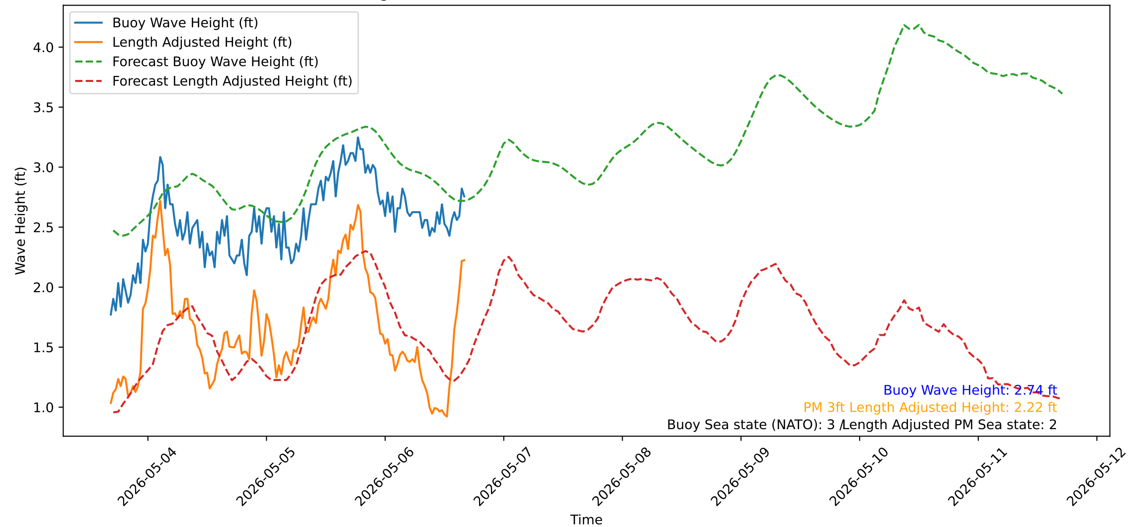
Wave Heights over Time for Oceanside Harbor at 2026-05-06 16:40:31
