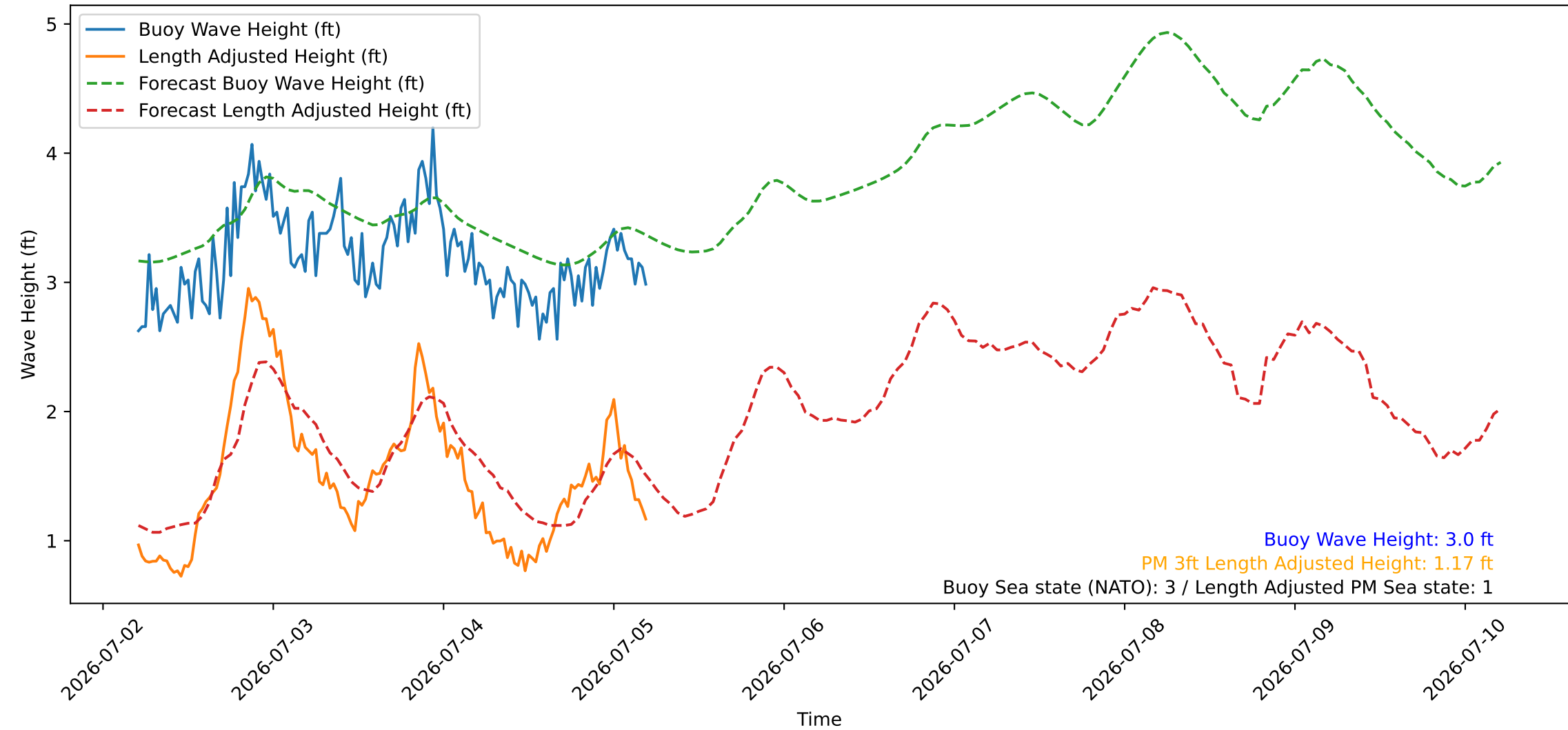
Wave Heights over Time for Green Beach at 2026-07-05 05:11:09
