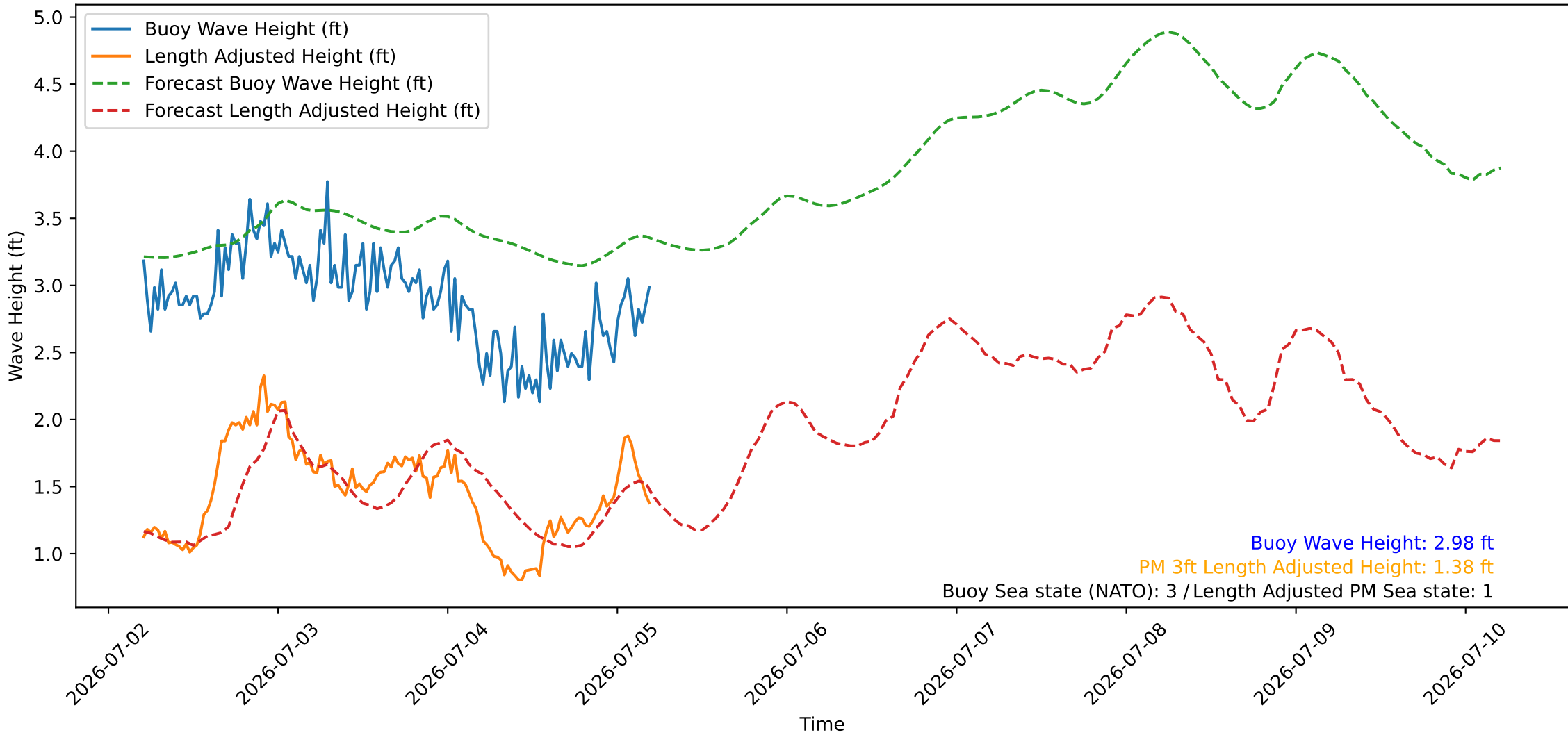
Wave Heights over Time for Oceanside Harbor at 2026-07-05 05:10:27
