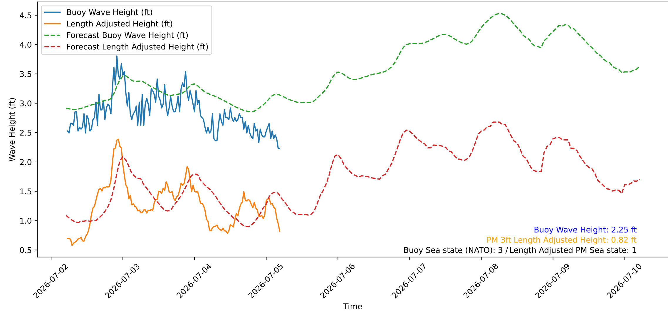
Wave Heights over Time for Red Beach at 2026-07-05 05:10:47
