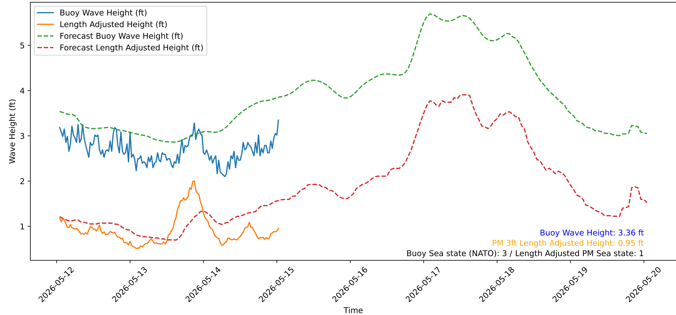
Wave Heights over Time for Green Beach at 2026-05-15 01:11:13
