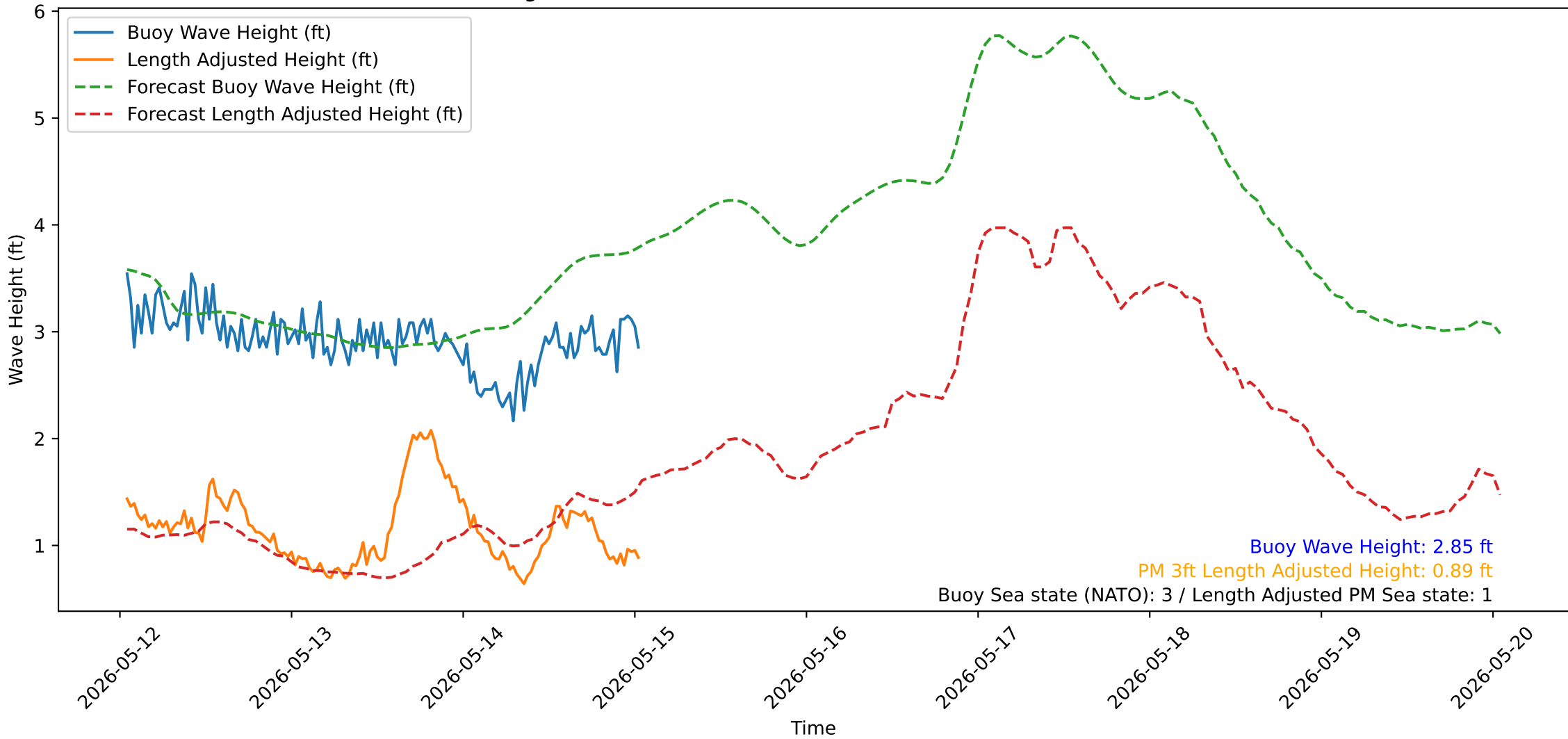
Wave Heights over Time for Oceanside Harbor at 2026-05-15 01:10:31
