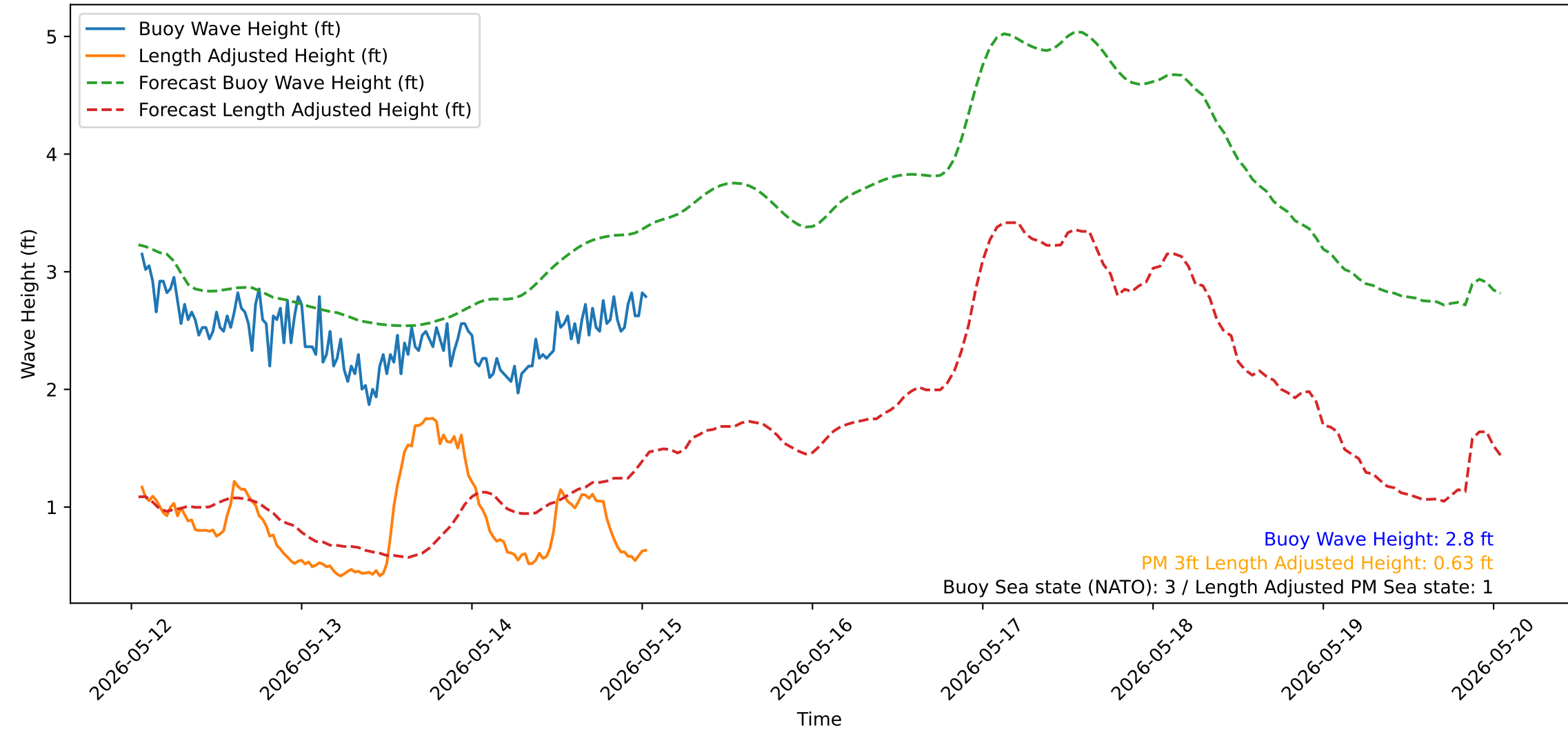
Wave Heights over Time for Red Beach at 2026-05-15 01:10:50
