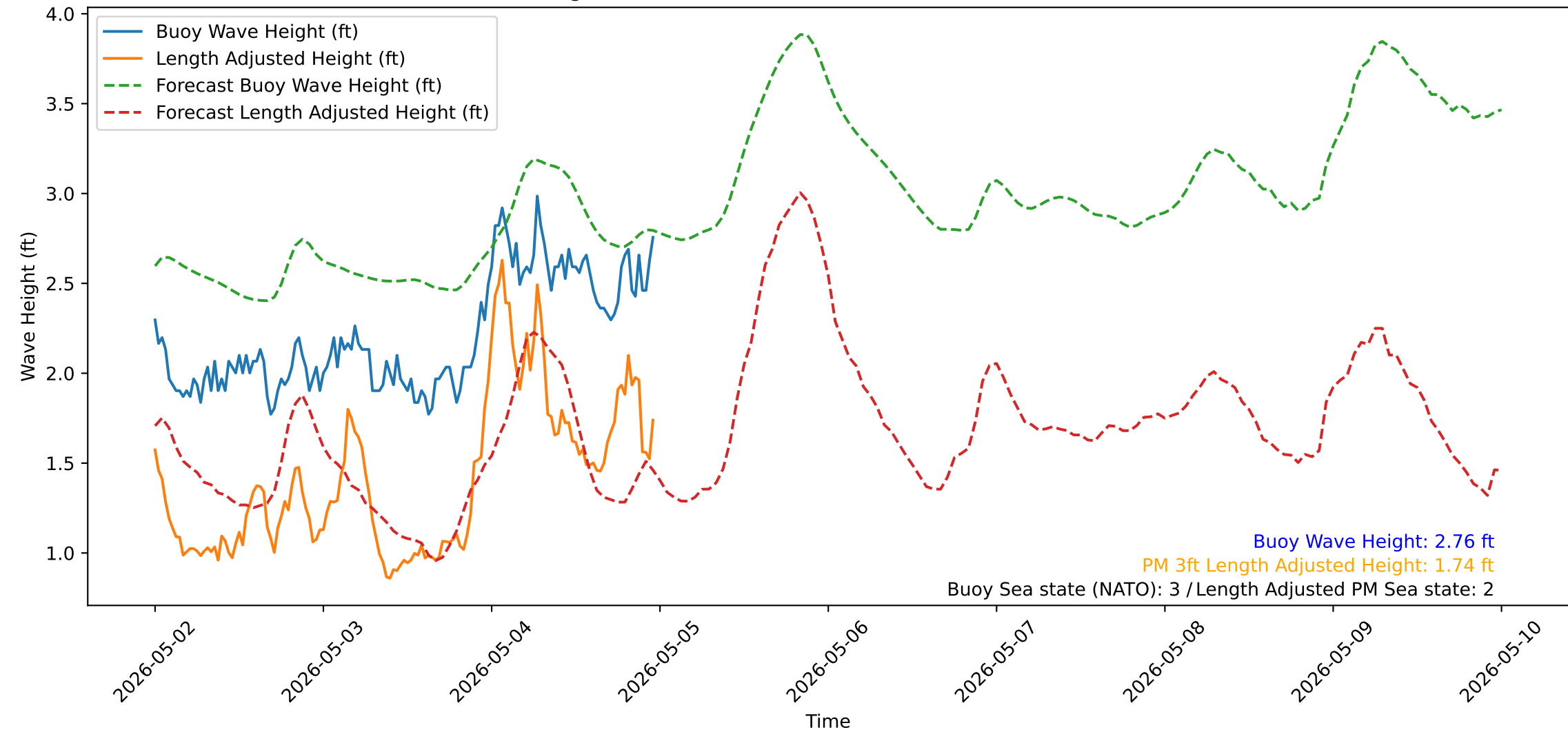
Wave Heights over Time for Green Beach at 2026-05-04 23:51:15
