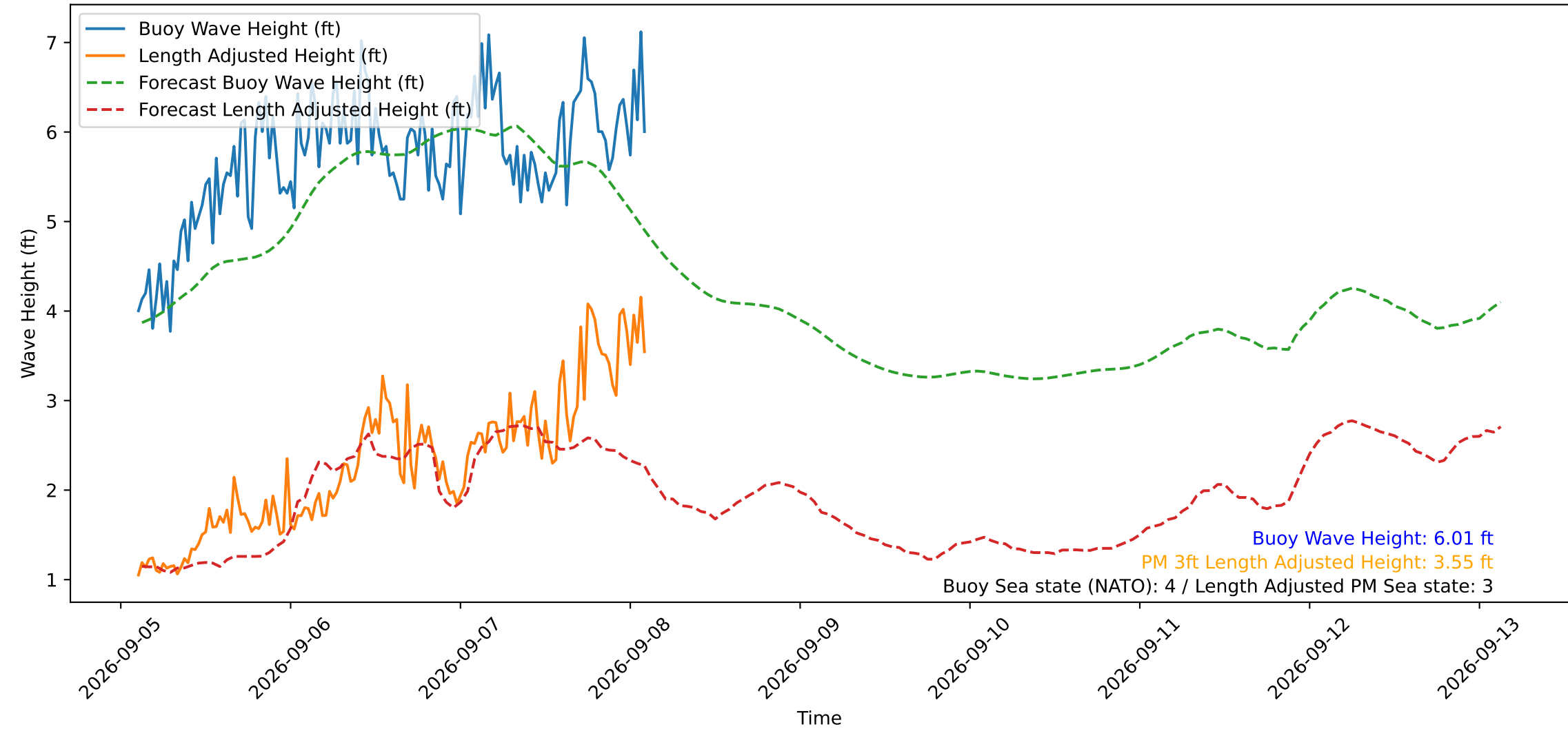
Wave Heights over Time for Oceanside Harbor at 2026-09-08 02:40:29
