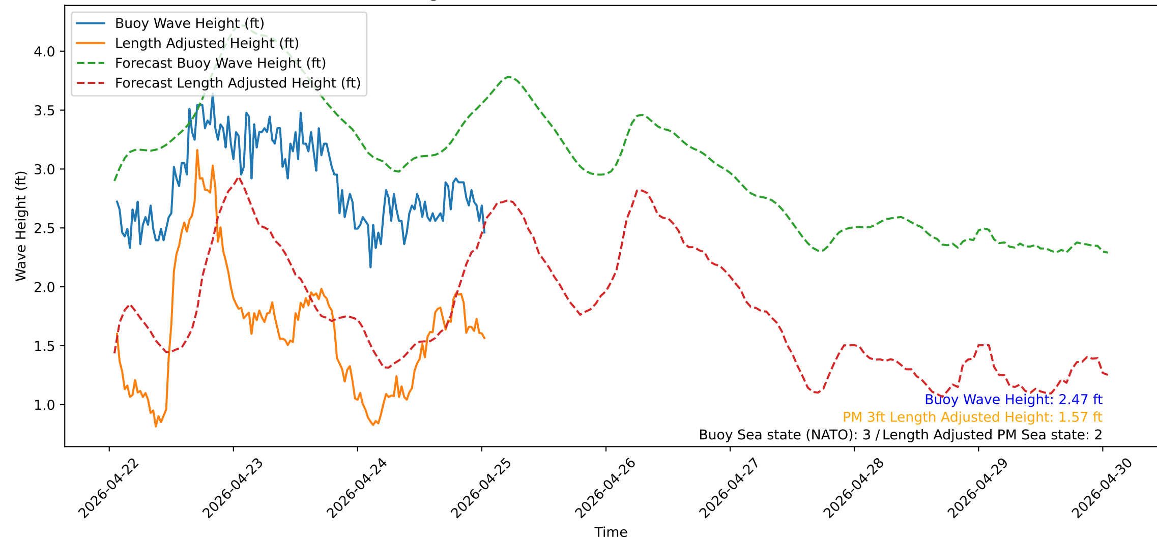
Wave Heights over Time for Red Beach at 2026-04-25 01:10:50
