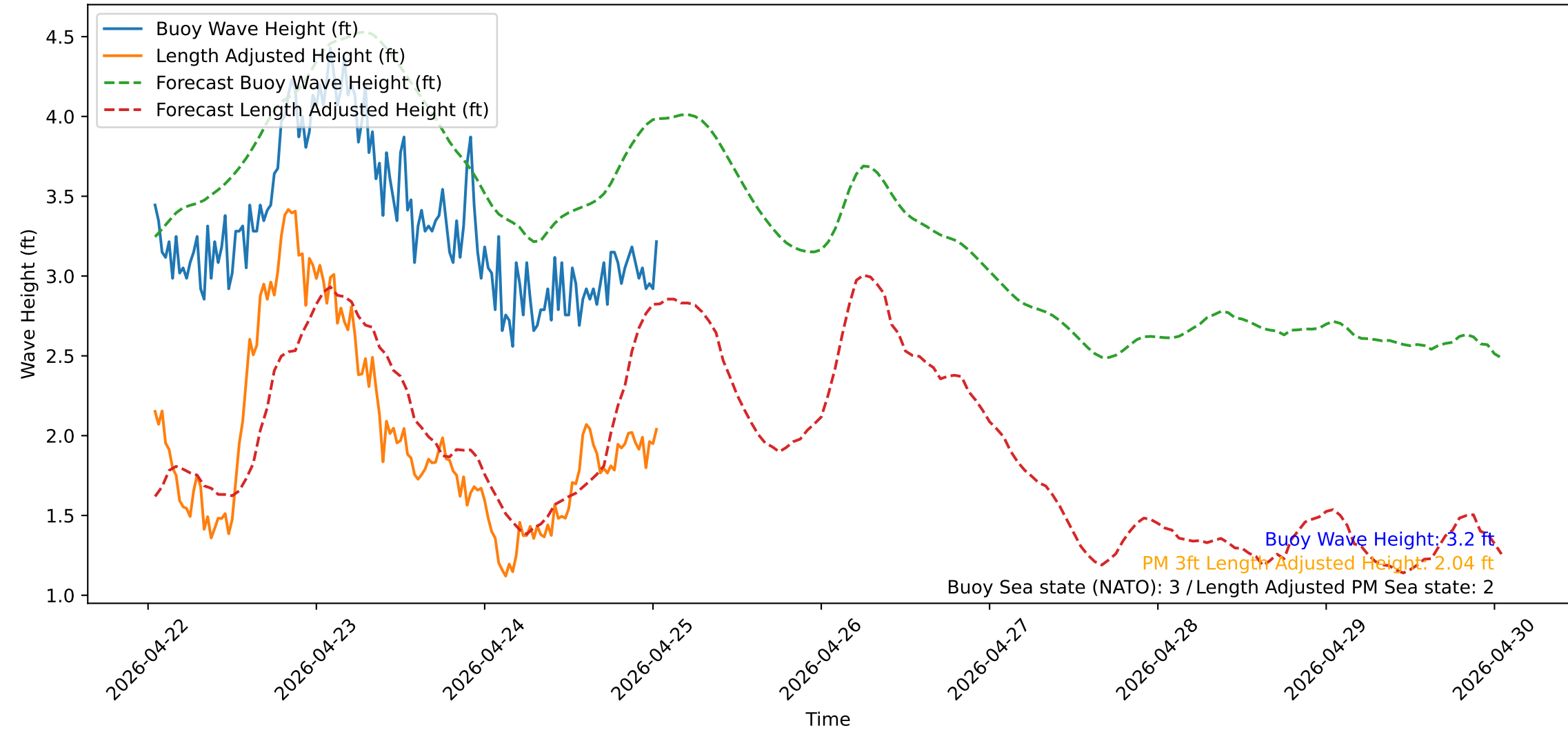
Wave Heights over Time for Oceanside Harbor at 2026-04-25 01:10:31
