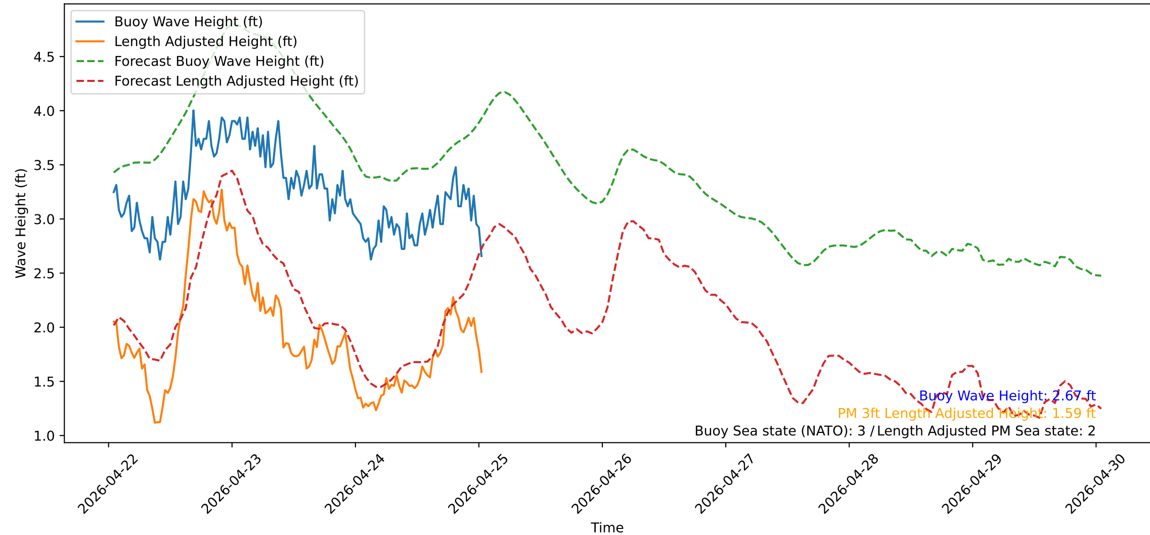
Wave Heights over Time for Green Beach at 2026-04-25 01:11:12
