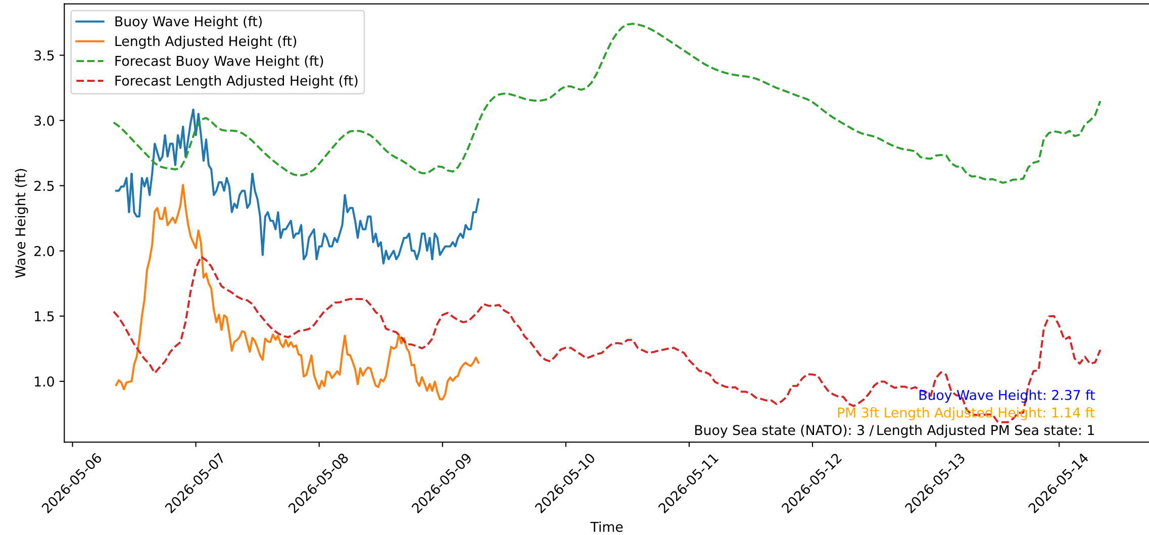
Wave Heights over Time for Red Beach at 2026-05-09 08:00:54
