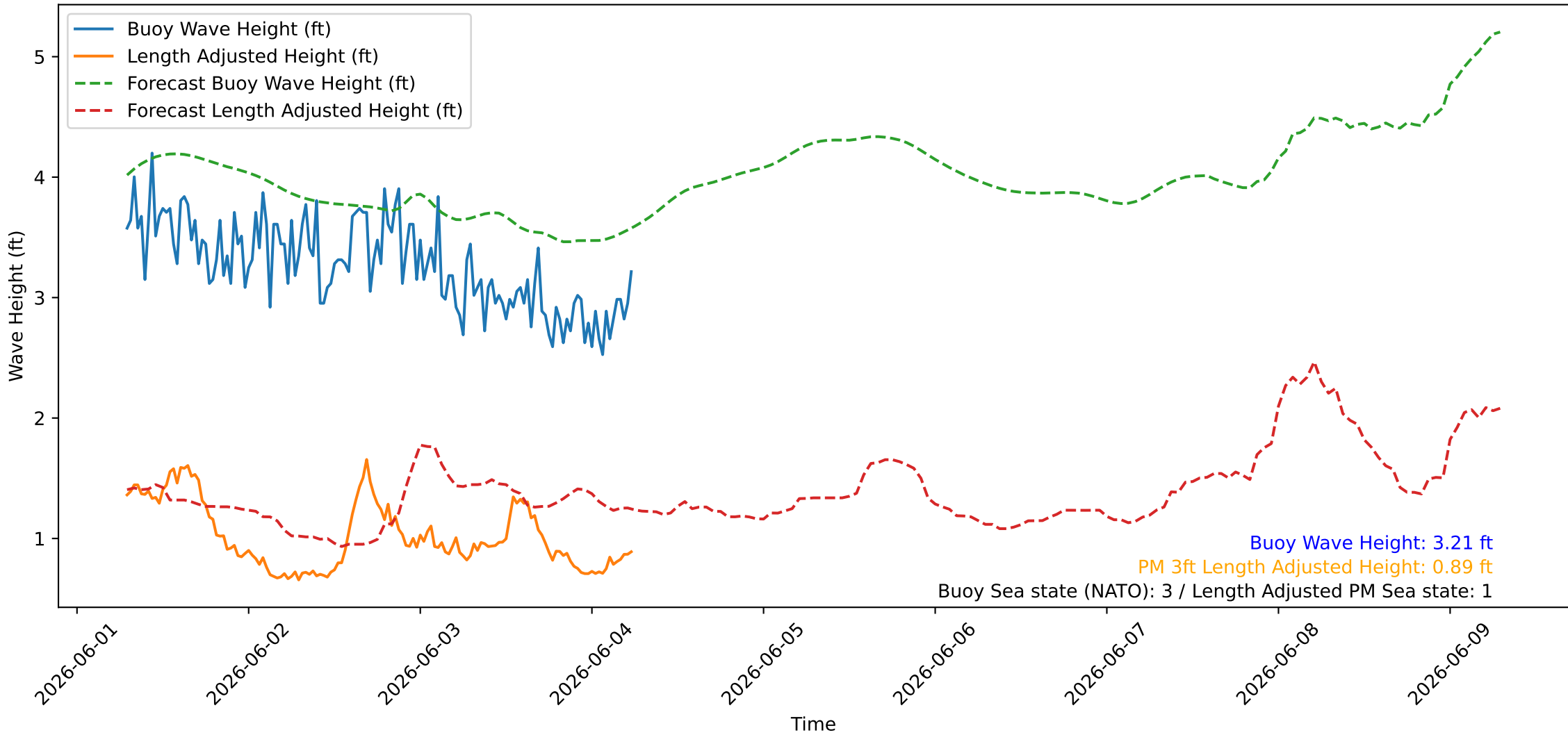
Wave Heights over Time for Red Beach at 2026-06-04 06:30:45
