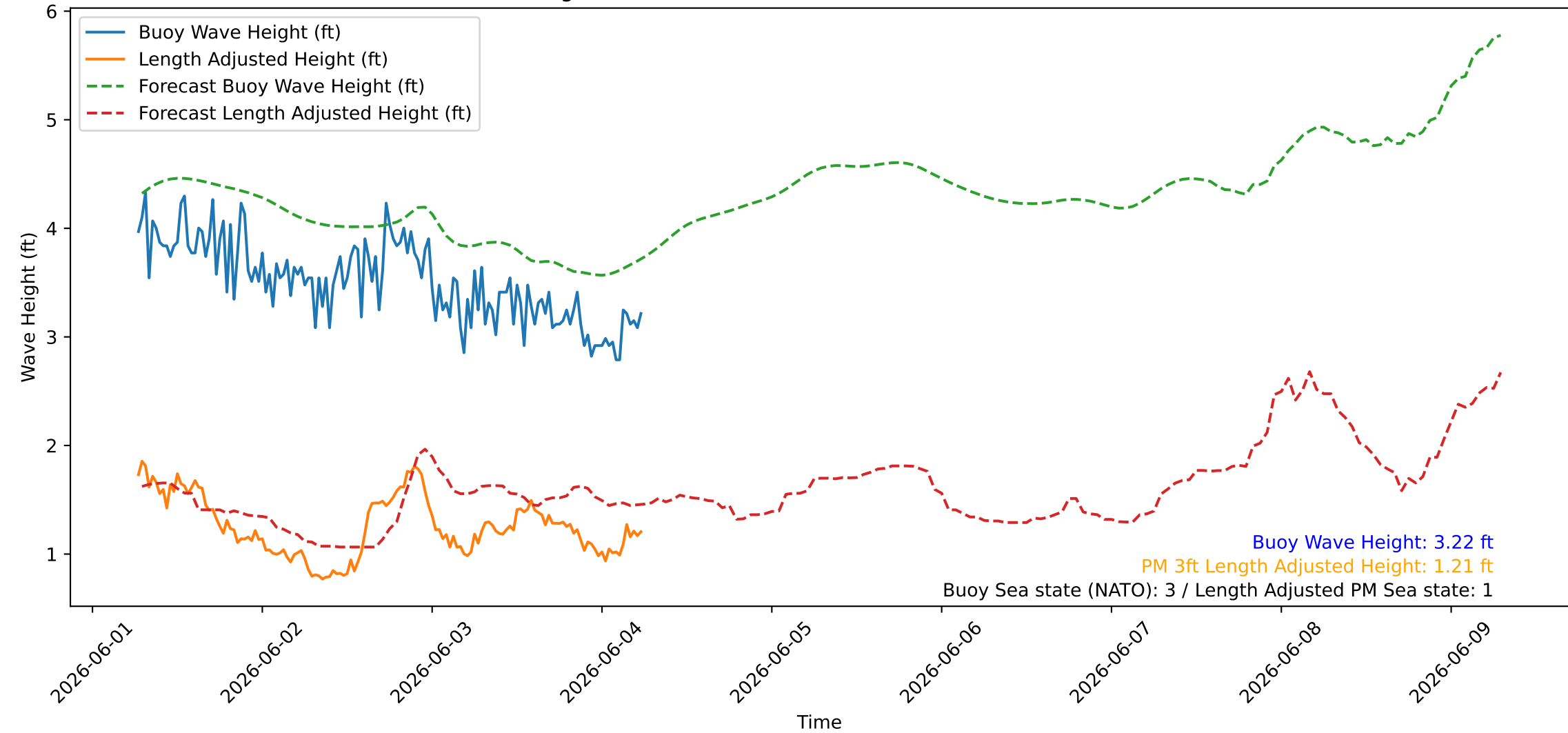
Wave Heights over Time for Green Beach at 2026-06-04 06:31:08
