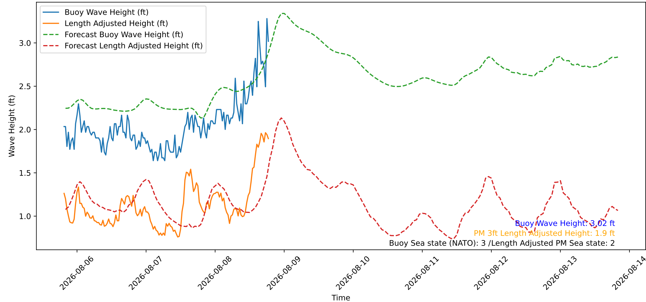
Wave Heights over Time for Oceanside Harbor at 2026-08-08 19:30:26
