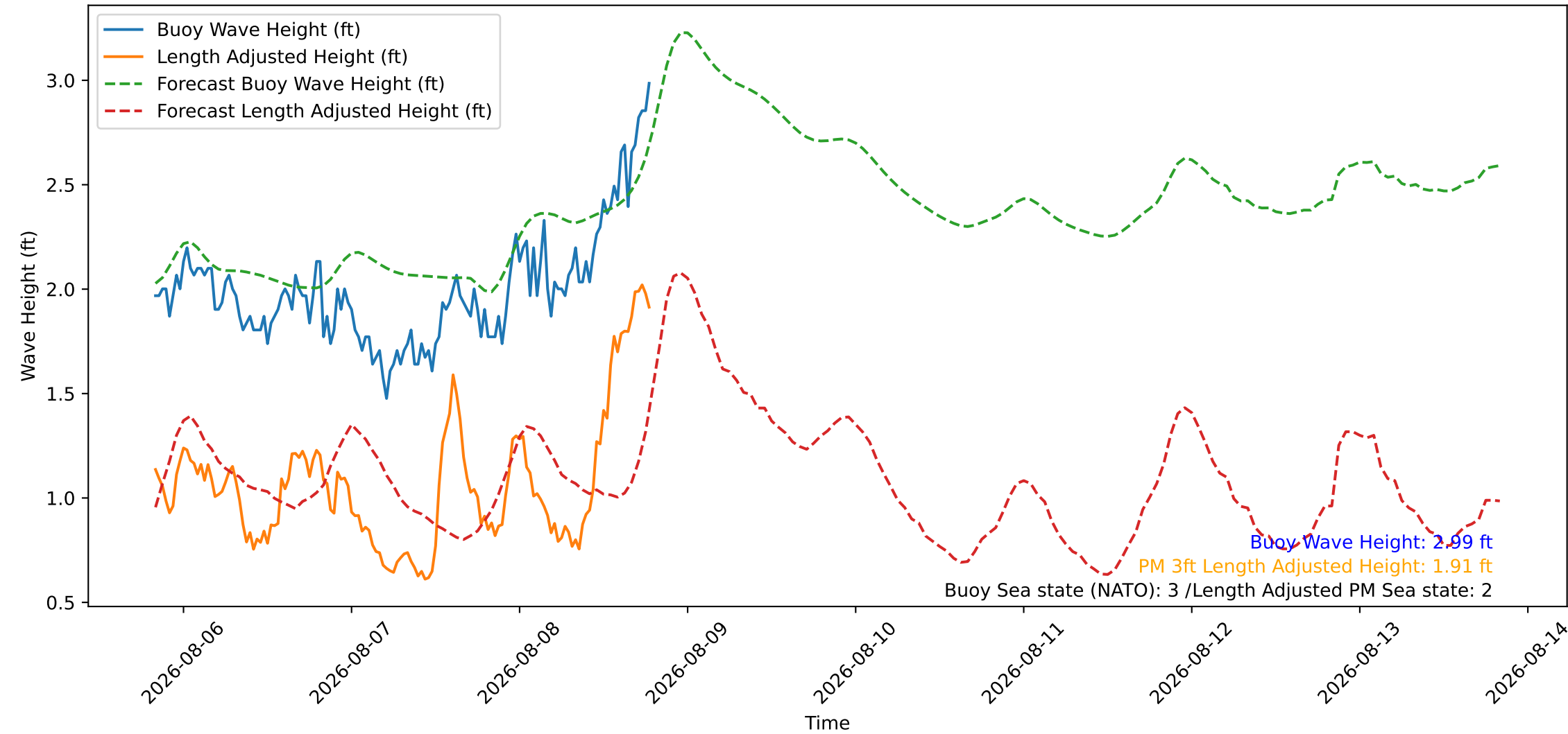
Wave Heights over Time for Red Beach at 2026-08-08 19:30:46
