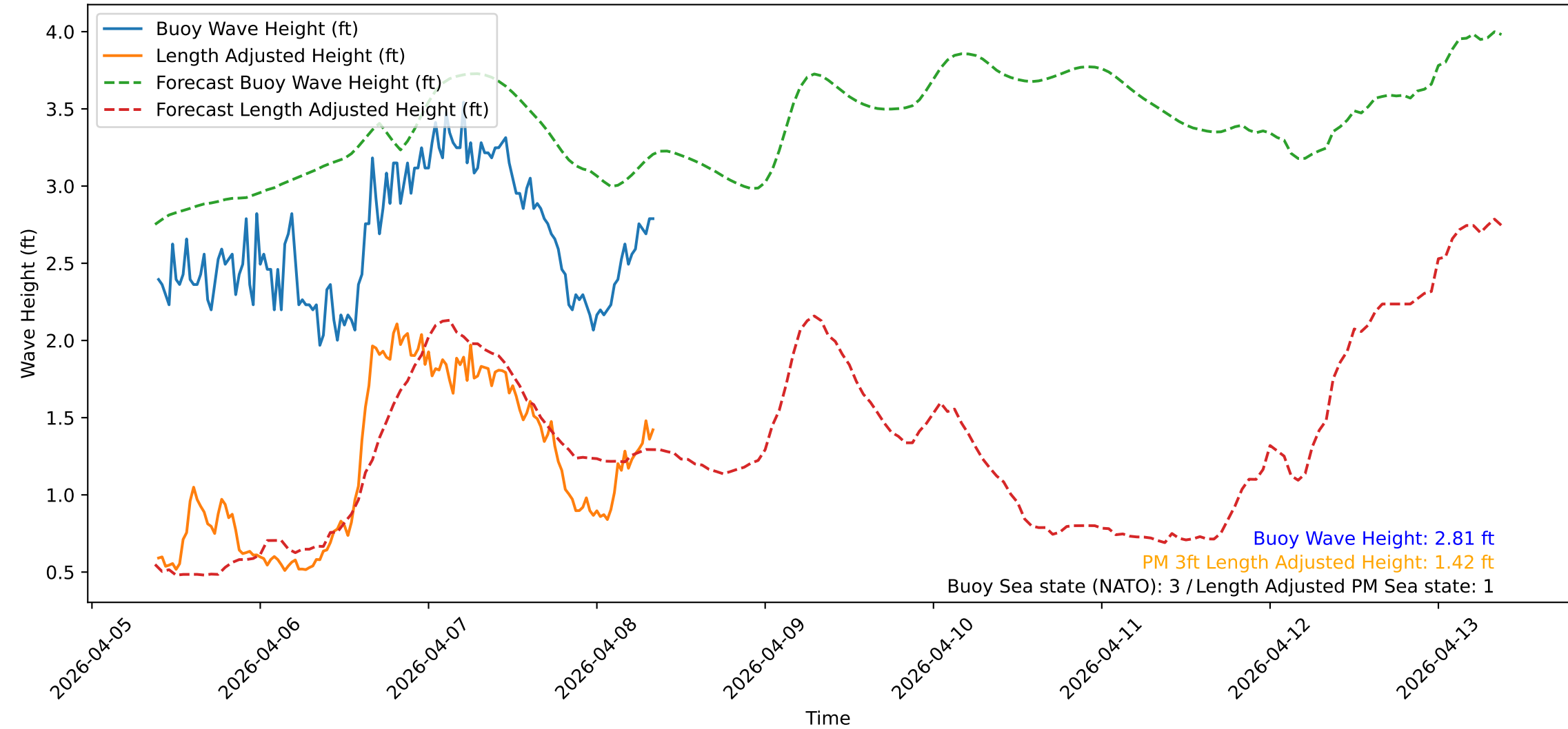
Wave Heights over Time for Red Beach at 2026-04-08 09:00:47
