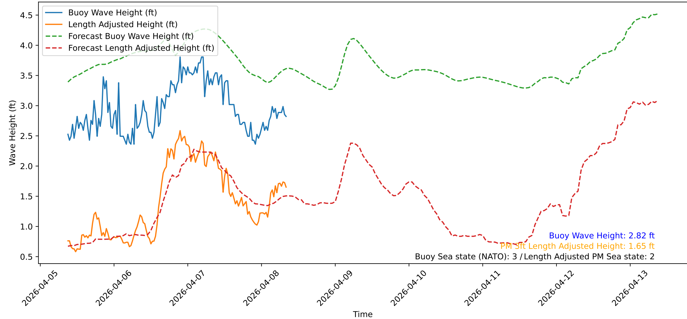
Wave Heights over Time for Green Beach at 2026-04-08 09:01:09
