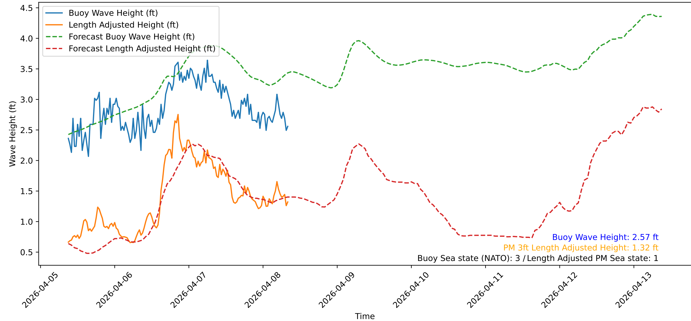
Wave Heights over Time for Oceanside Harbor at 2026-04-08 09:00:31
