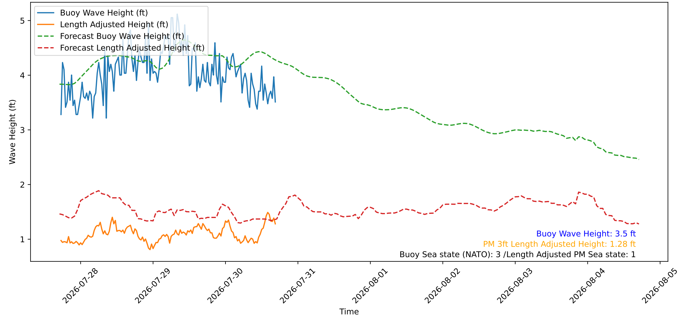
Wave Heights over Time for Red Beach at 2026-07-30 17:10:49
