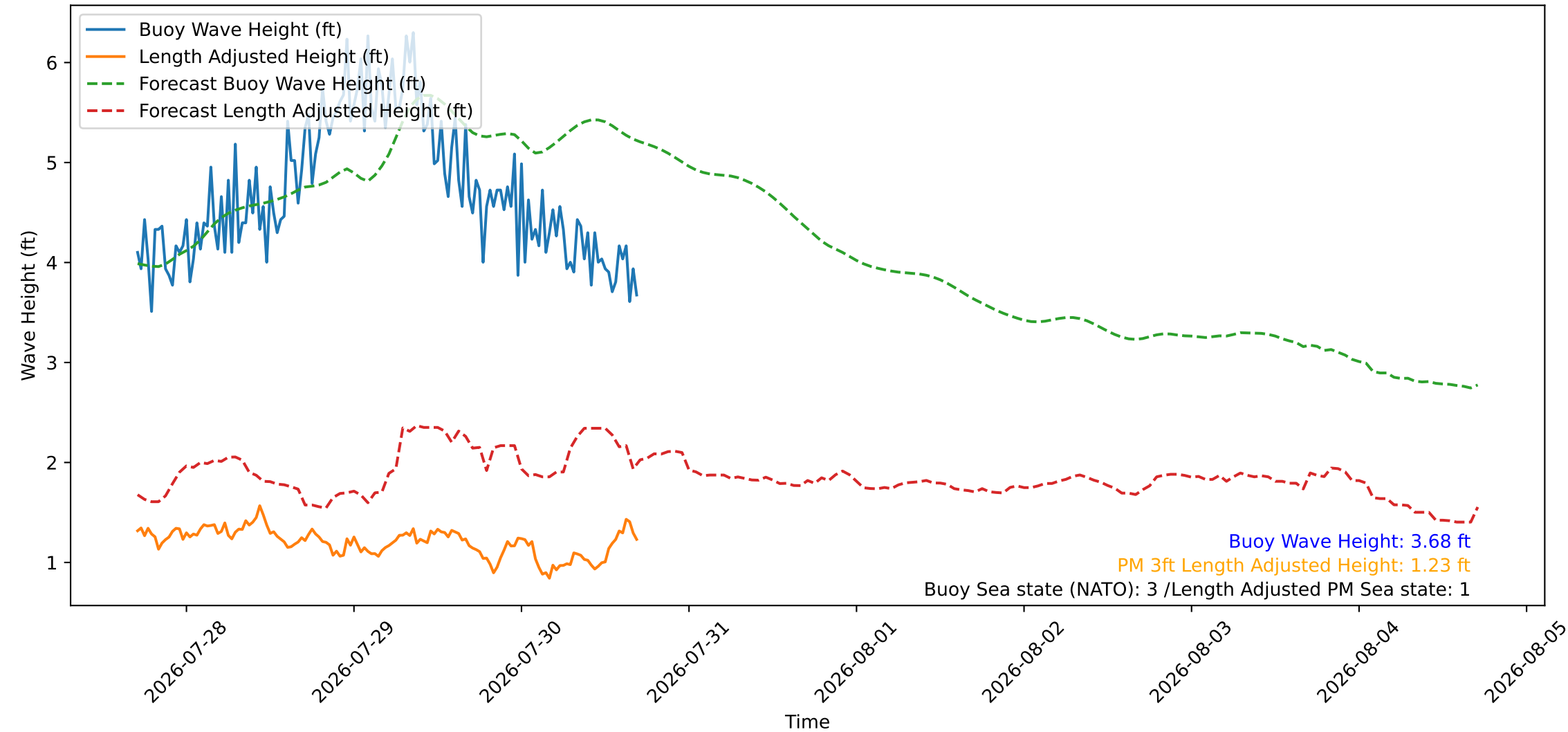
Wave Heights over Time for Green Beach at 2026-07-30 17:11:15
