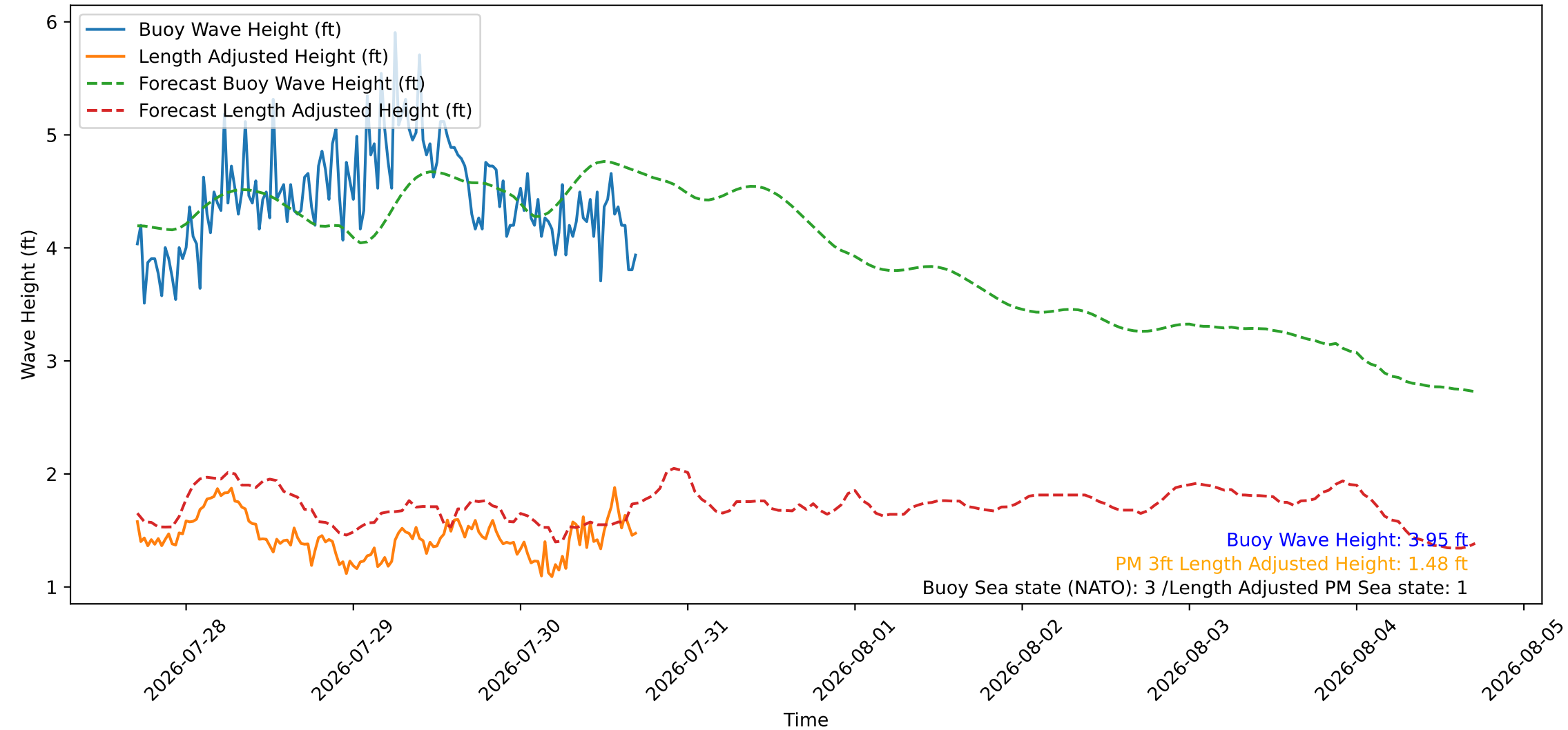
Wave Heights over Time for Oceanside Harbor at 2026-07-30 17:10:28
