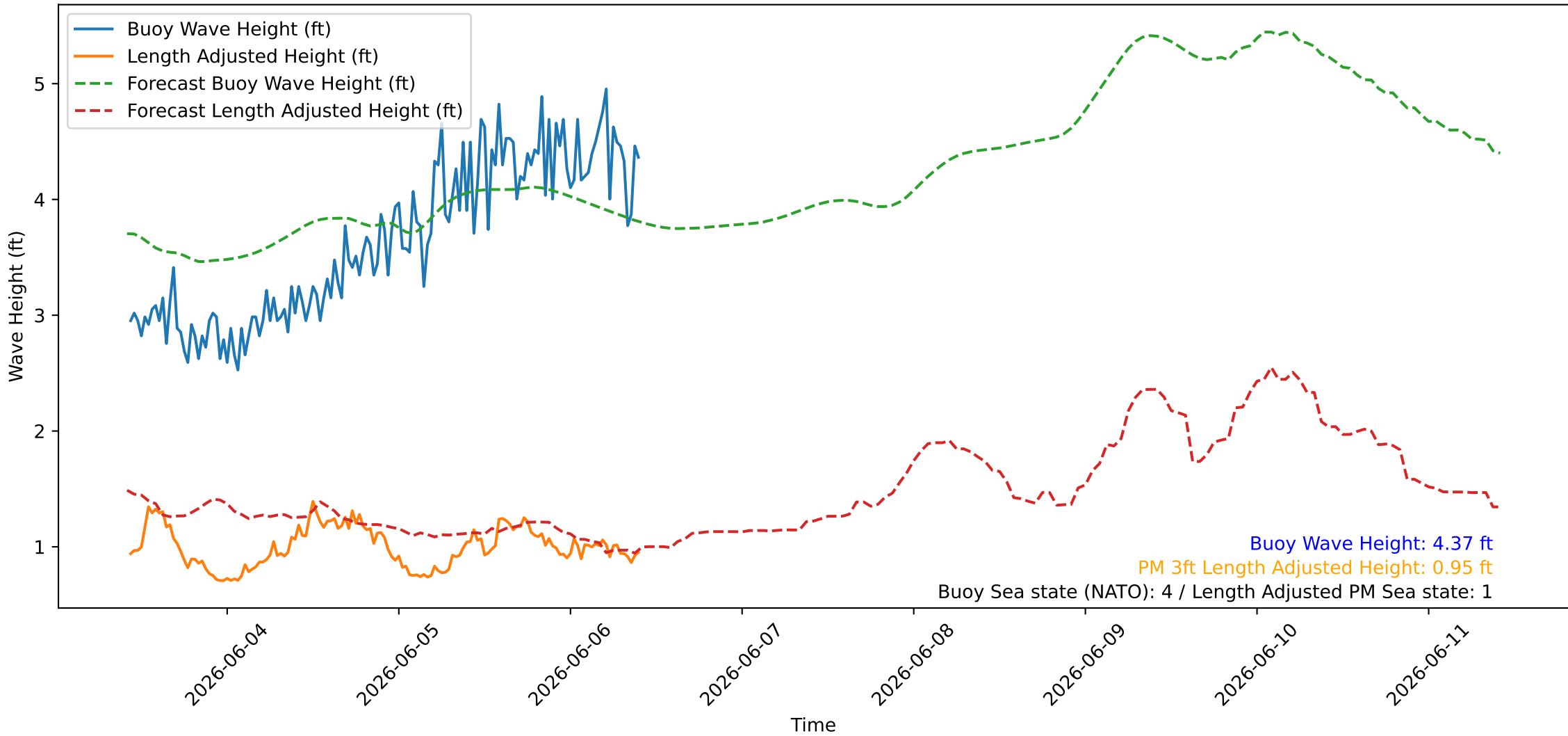
Wave Heights over Time for Red Beach at 2026-06-06 10:10:46
