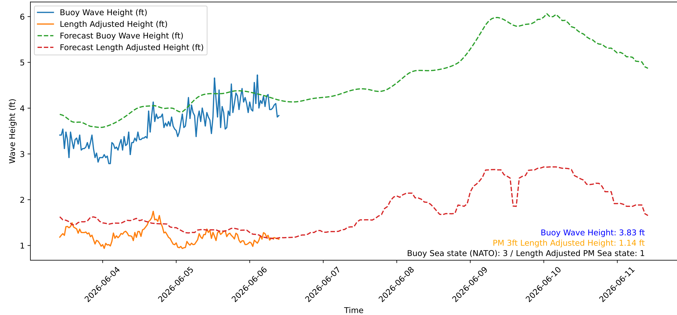
Wave Heights over Time for Green Beach at 2026-06-06 10:11:08
