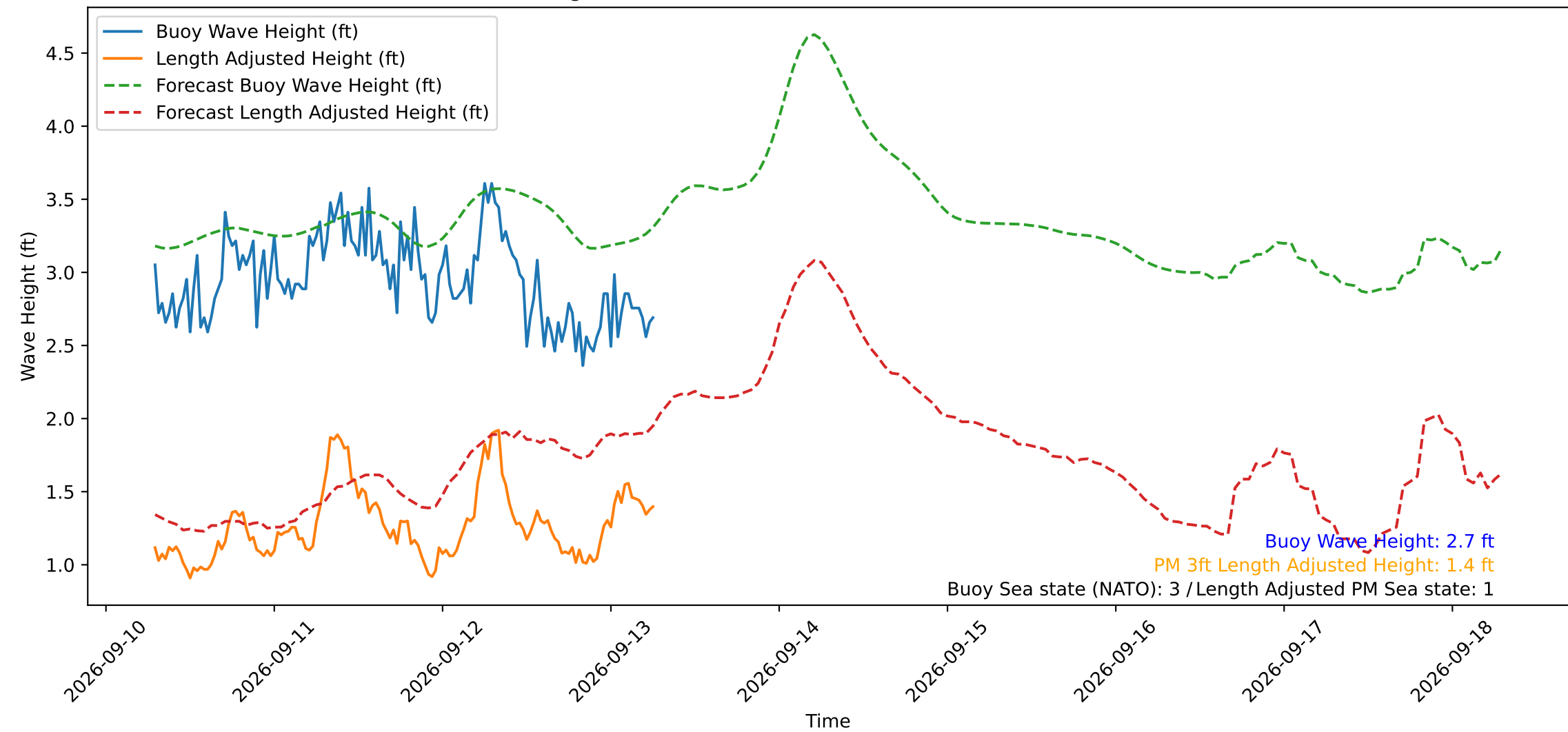
Wave Heights over Time for Green Beach at 2026-09-13 06:41:11
