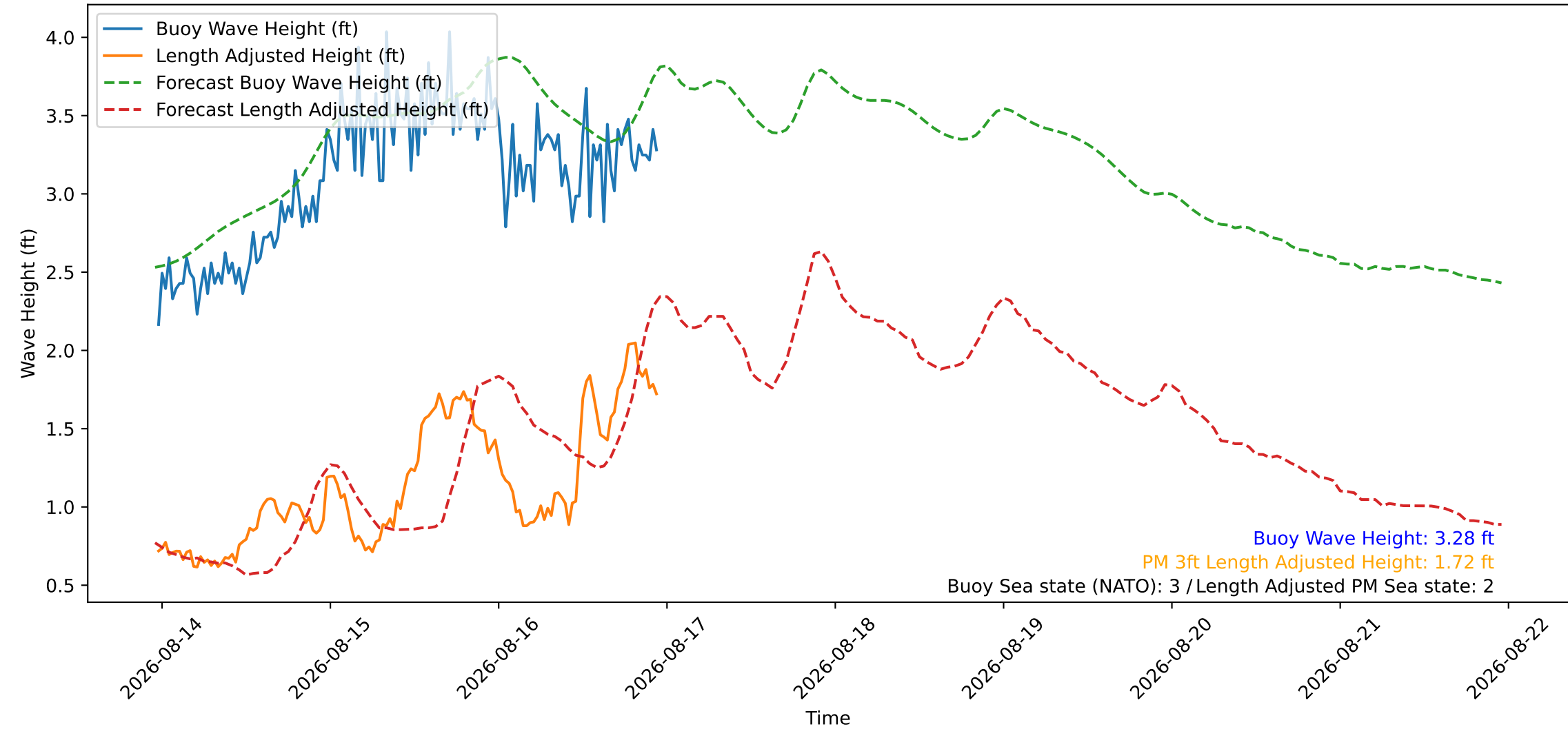
Wave Heights over Time for Red Beach at 2026-08-16 23:20:47
