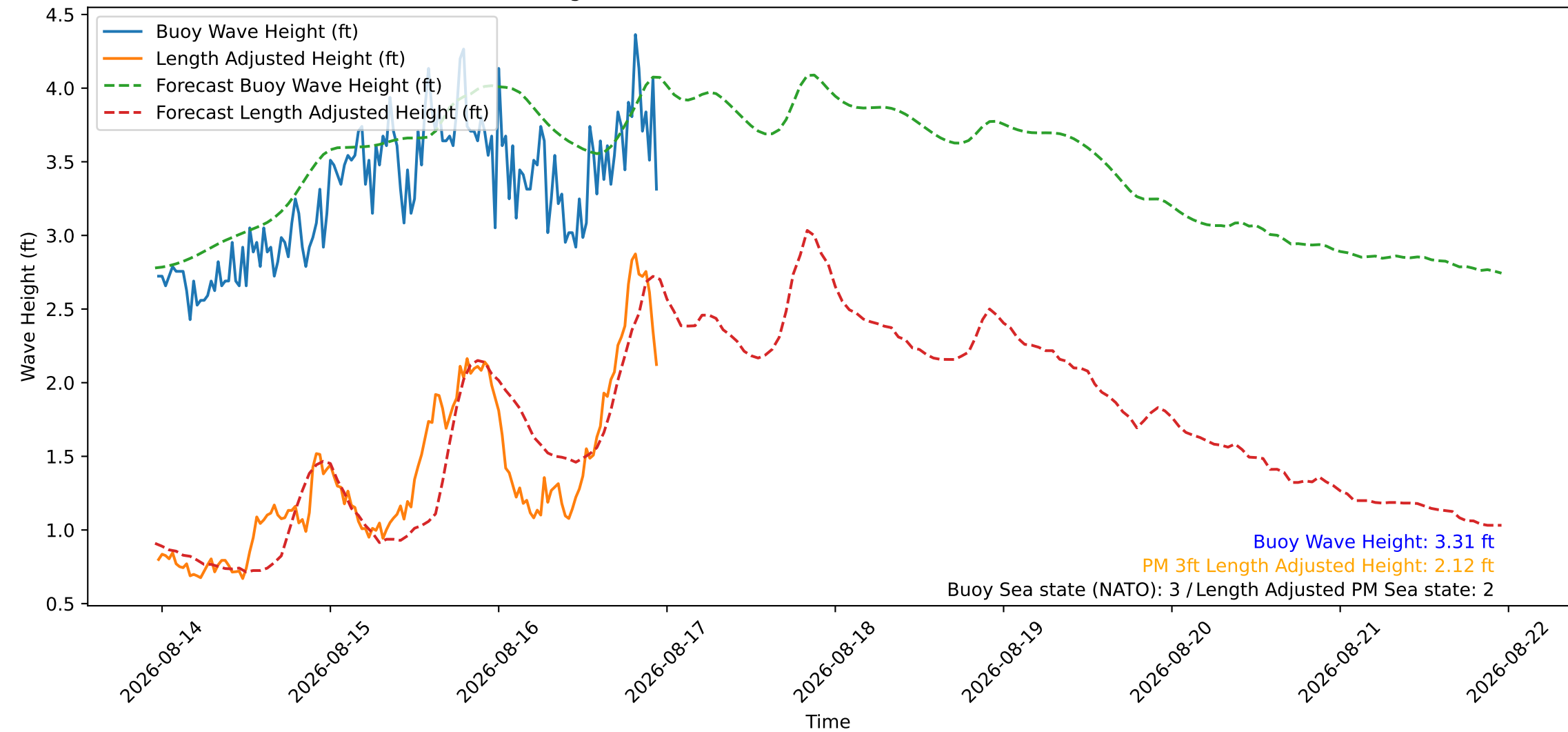
Wave Heights over Time for Green Beach at 2026-08-16 23:21:10
