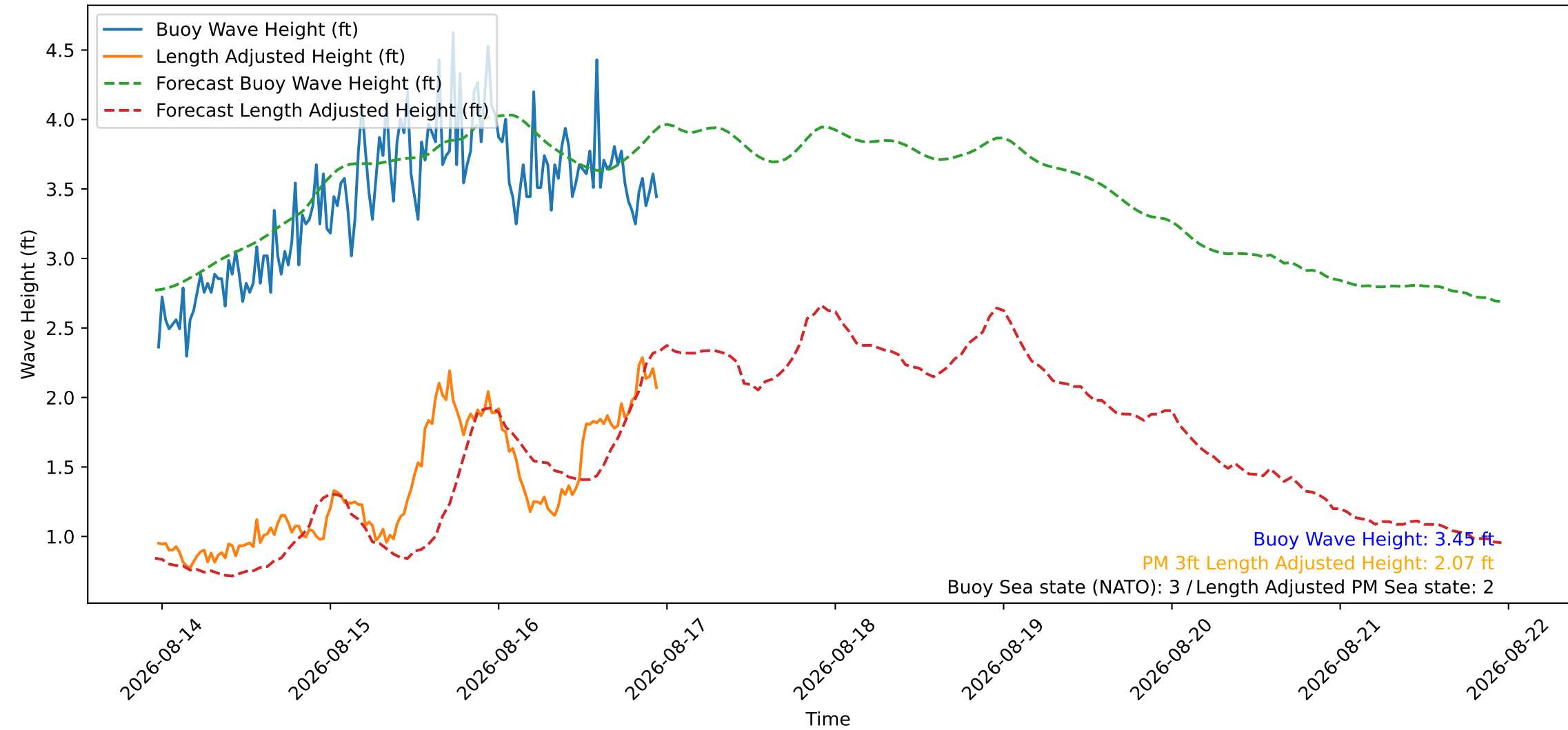
Wave Heights over Time for Oceanside Harbor at 2026-08-16 23:20:26
