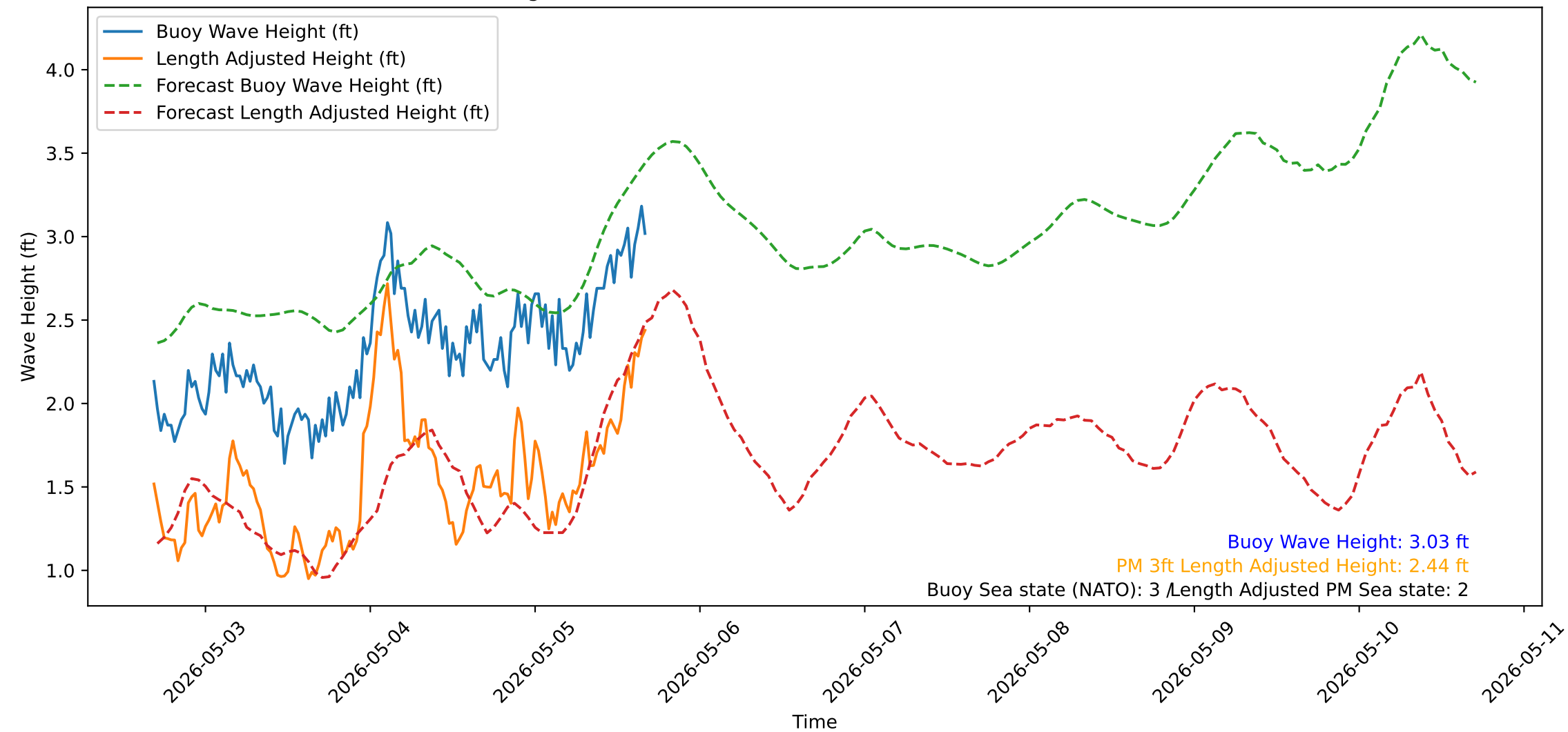
Wave Heights over Time for Oceanside Harbor at 2026-05-05 16:30:31
