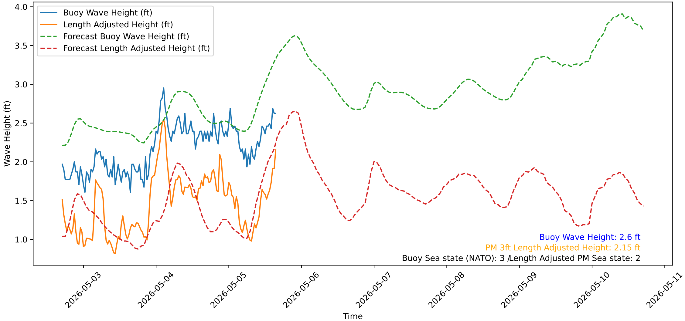
Wave Heights over Time for Red Beach at 2026-05-05 16:30:51
