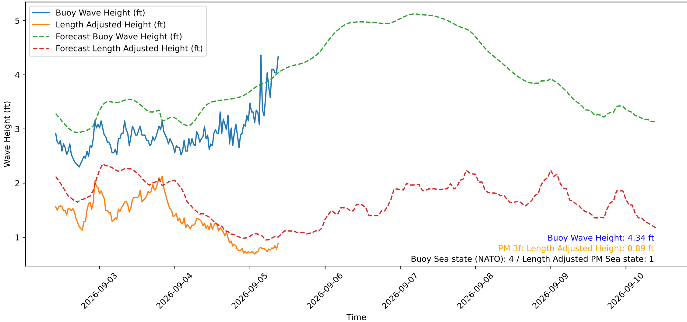
Wave Heights over Time for Red Beach at 2026-09-05 09:50:51
