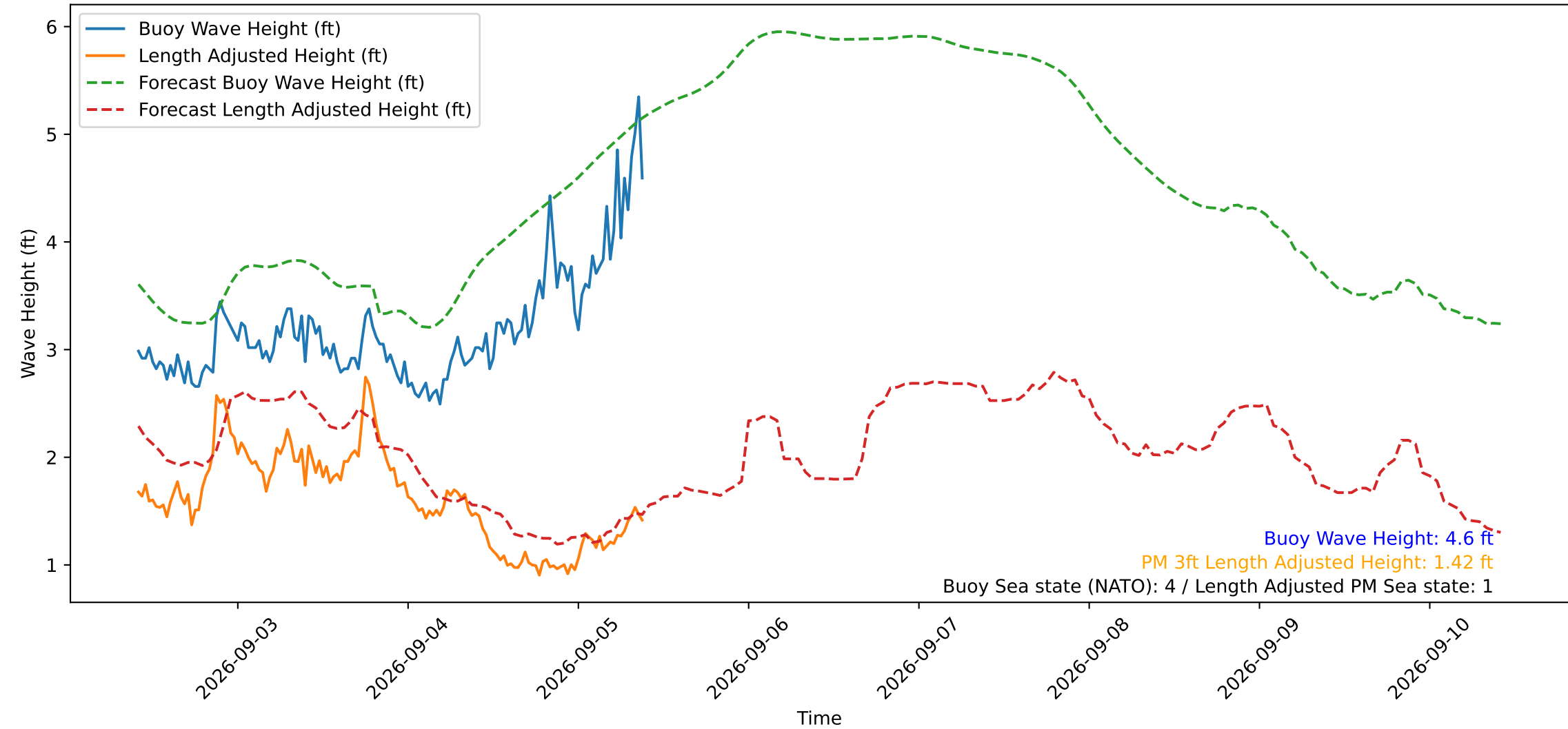
Wave Heights over Time for Green Beach at 2026-09-05 09:51:15
