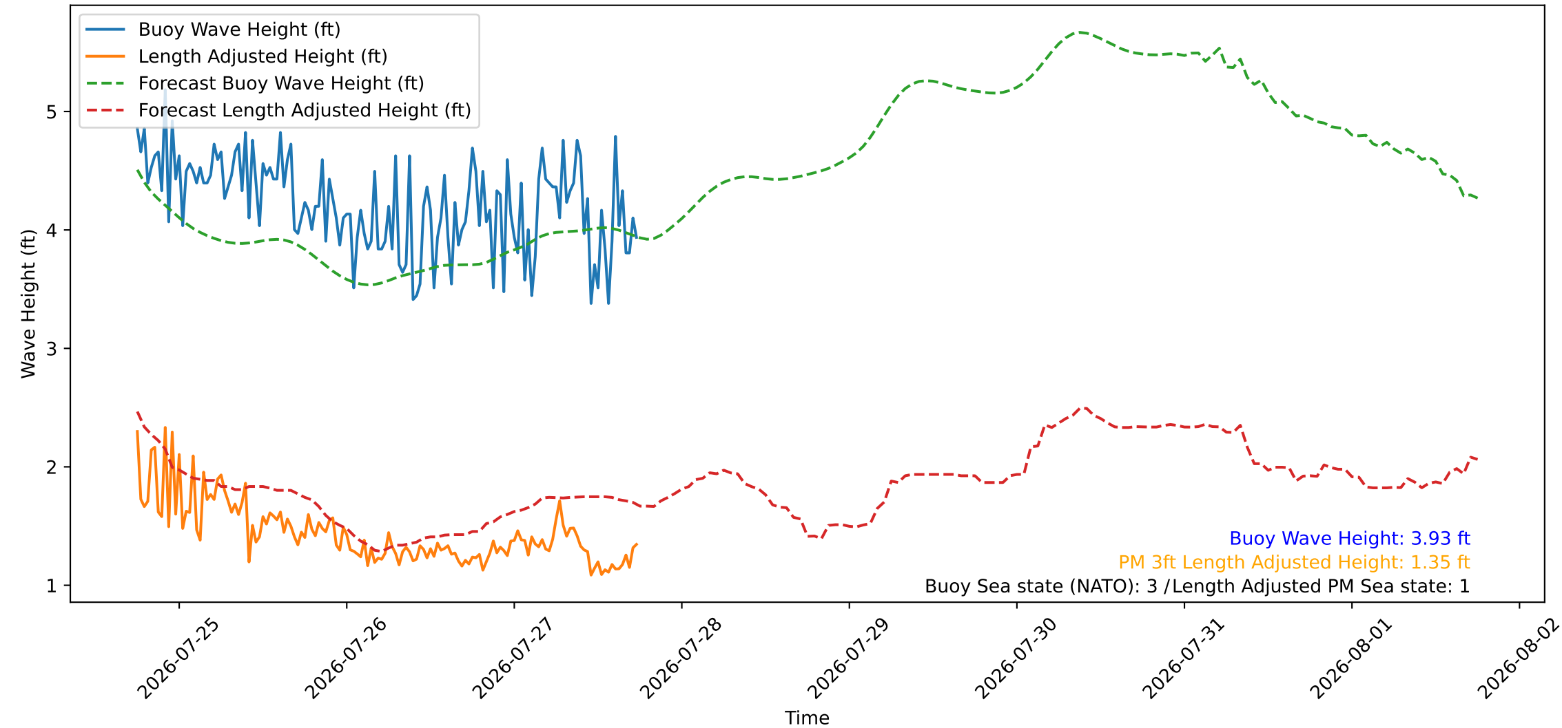
Wave Heights over Time for Green Beach at 2026-07-27 18:11:09
