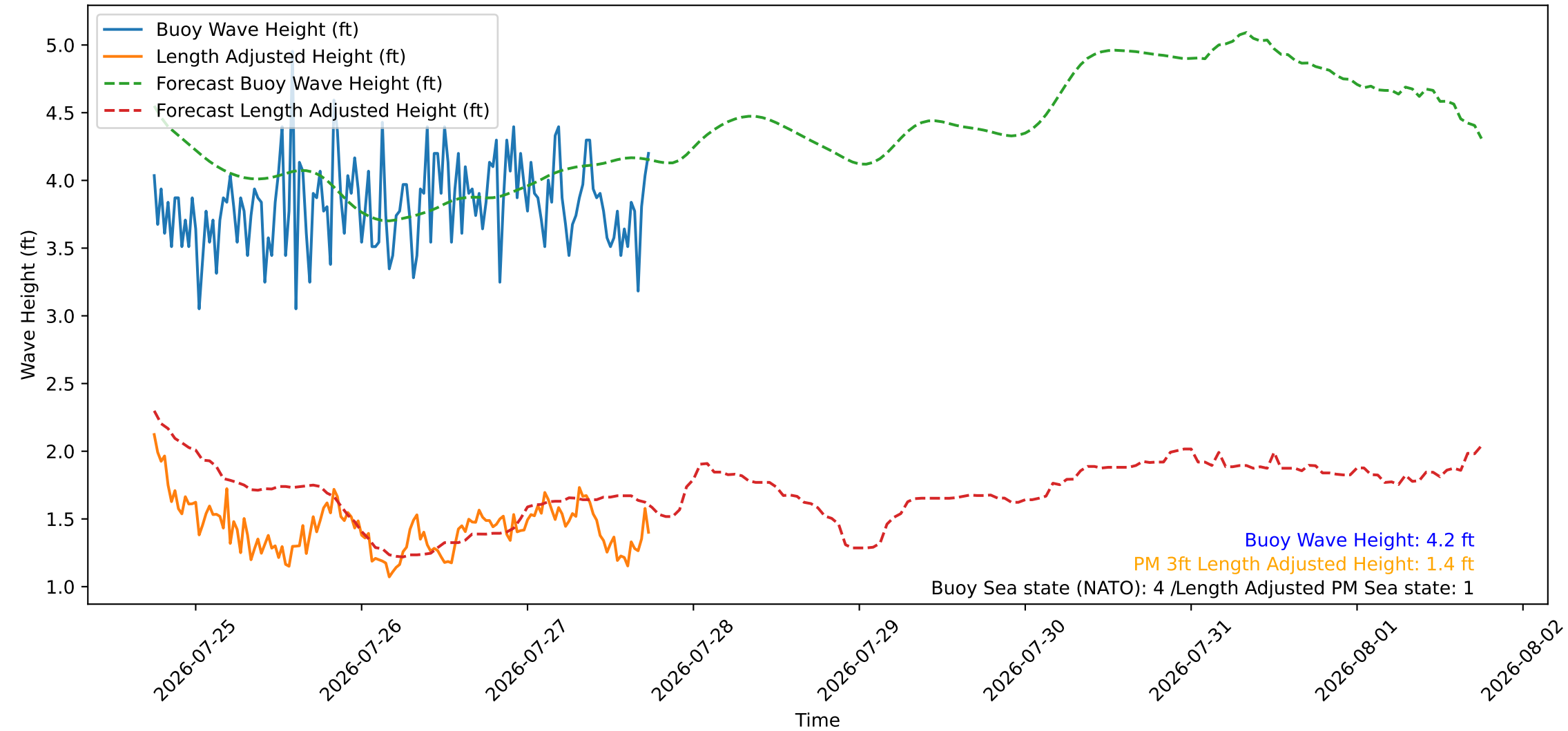
Wave Heights over Time for Oceanside Harbor at 2026-07-27 18:10:26
