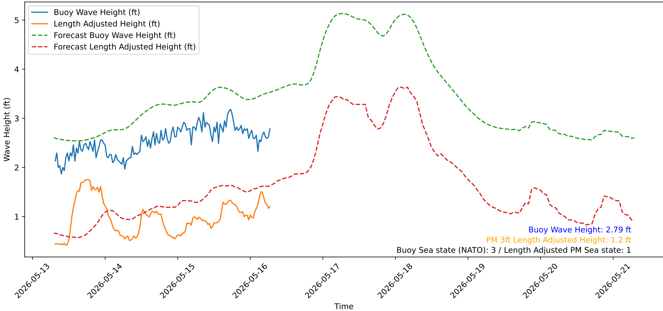
Wave Heights over Time for Red Beach at 2026-05-16 07:20:52
