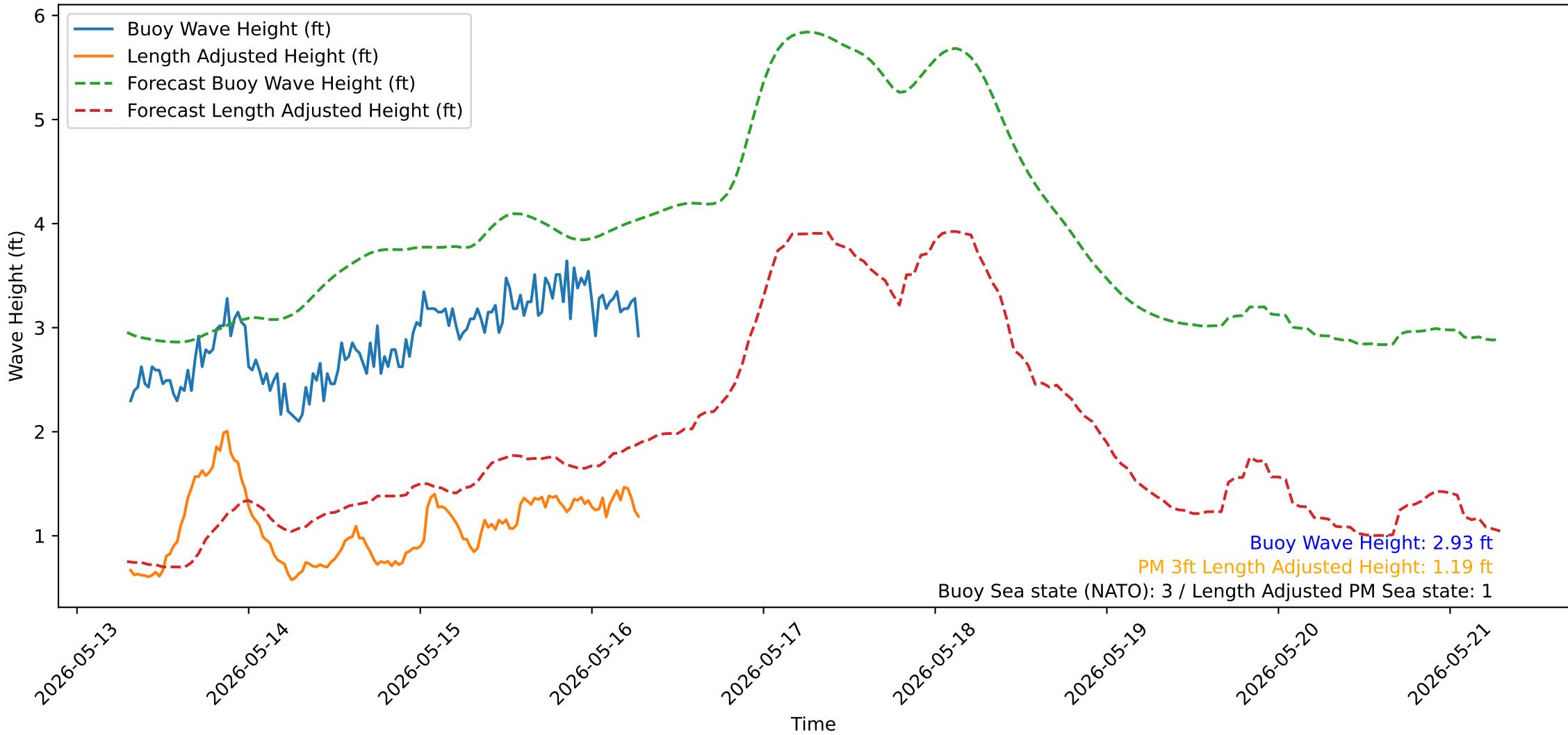
Wave Heights over Time for Green Beach at 2026-05-16 07:21:15
