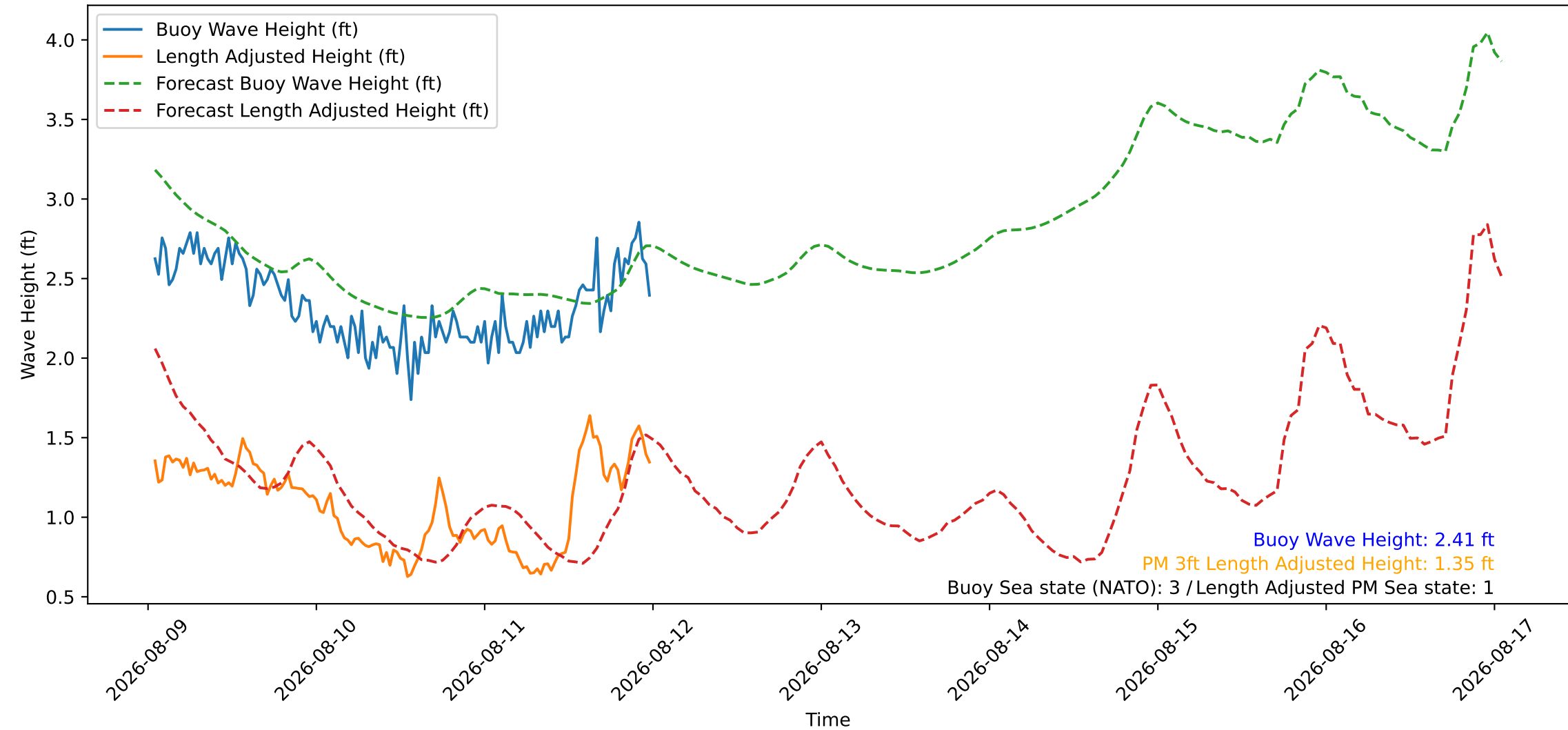
Wave Heights over Time for Red Beach at 2026-08-12 00:40:46
