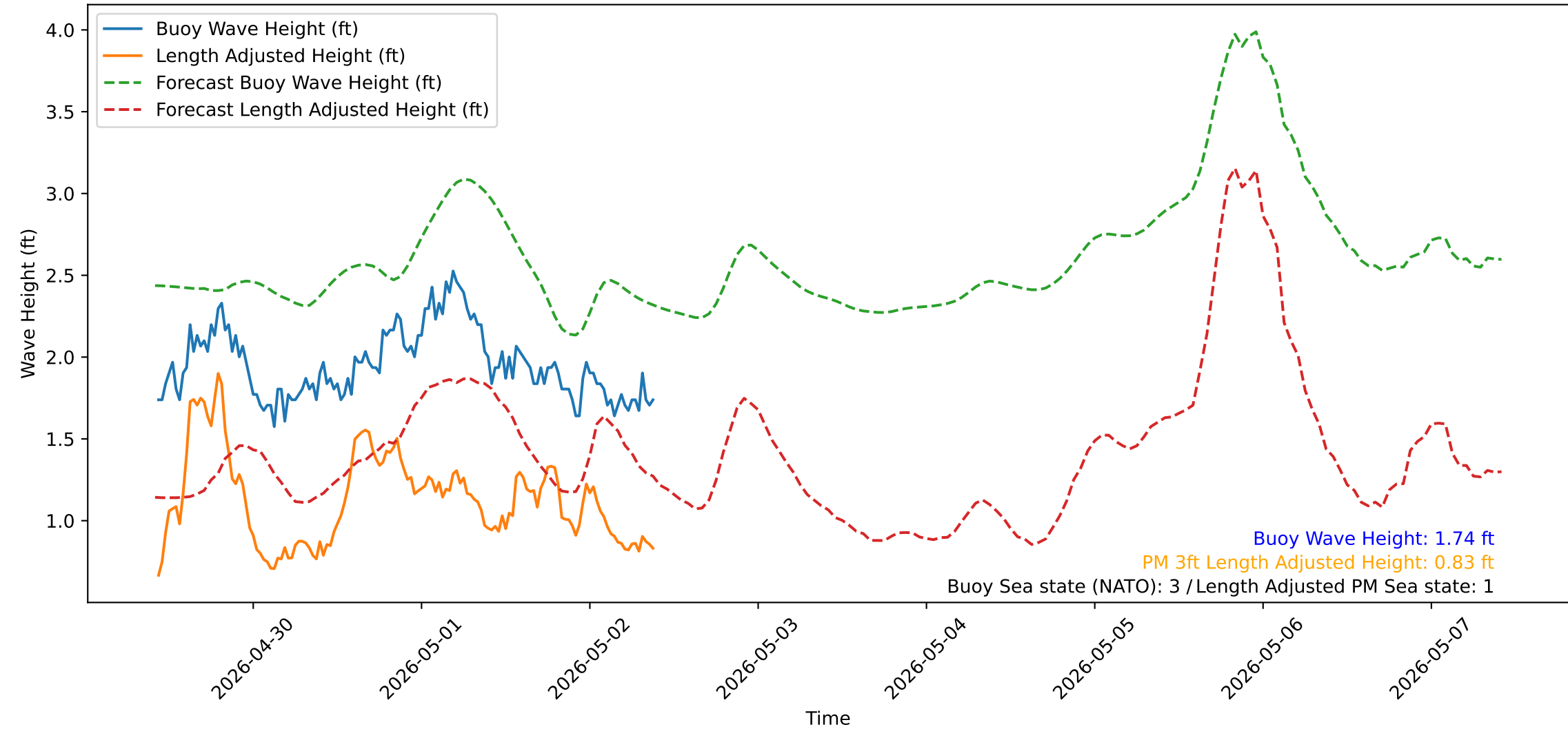
Wave Heights over Time for Red Beach at 2026-05-02 10:00:50
