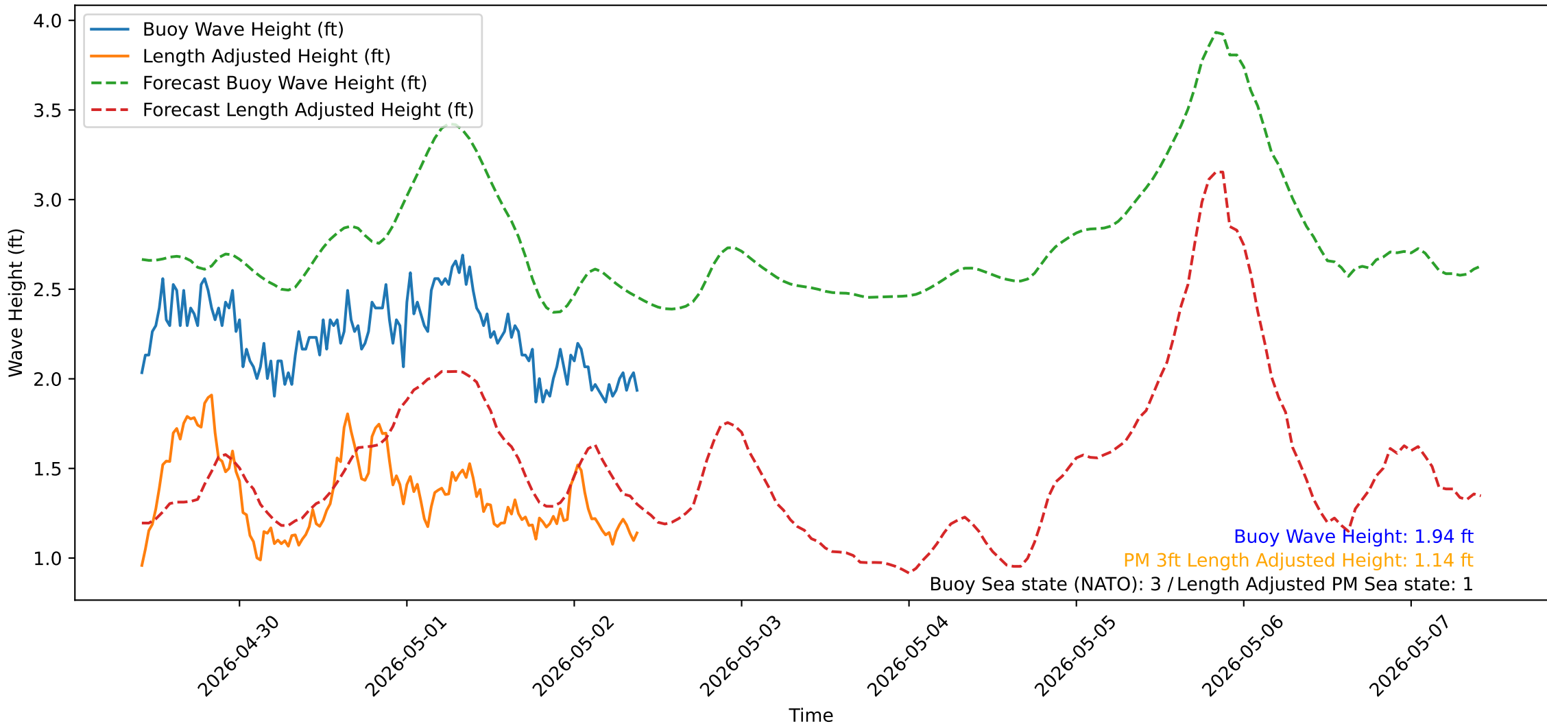
Wave Heights over Time for Oceanside Harbor at 2026-05-02 10:00:31
