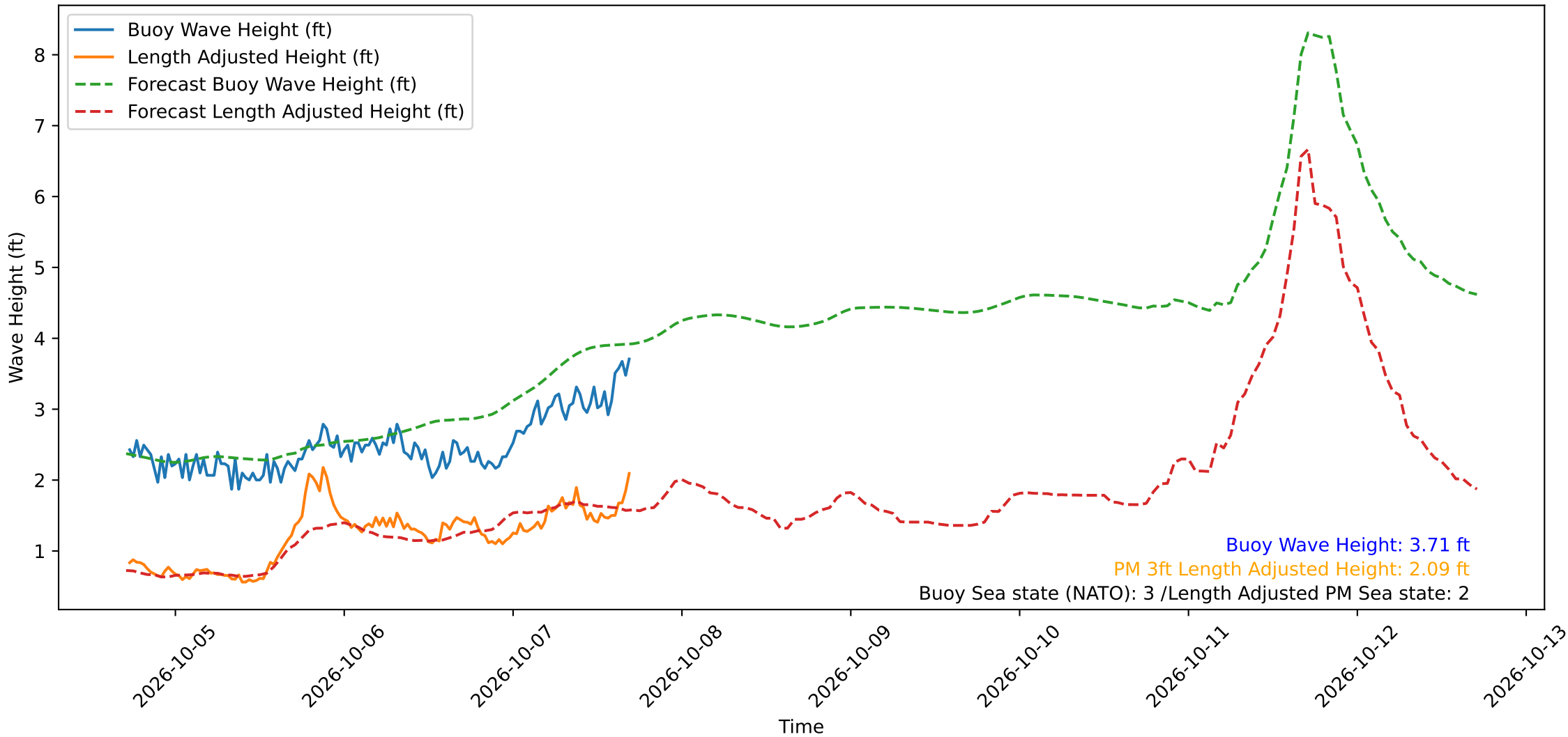
Wave Heights over Time for Oceanside Harbor at 2026-10-07 17:20:29
