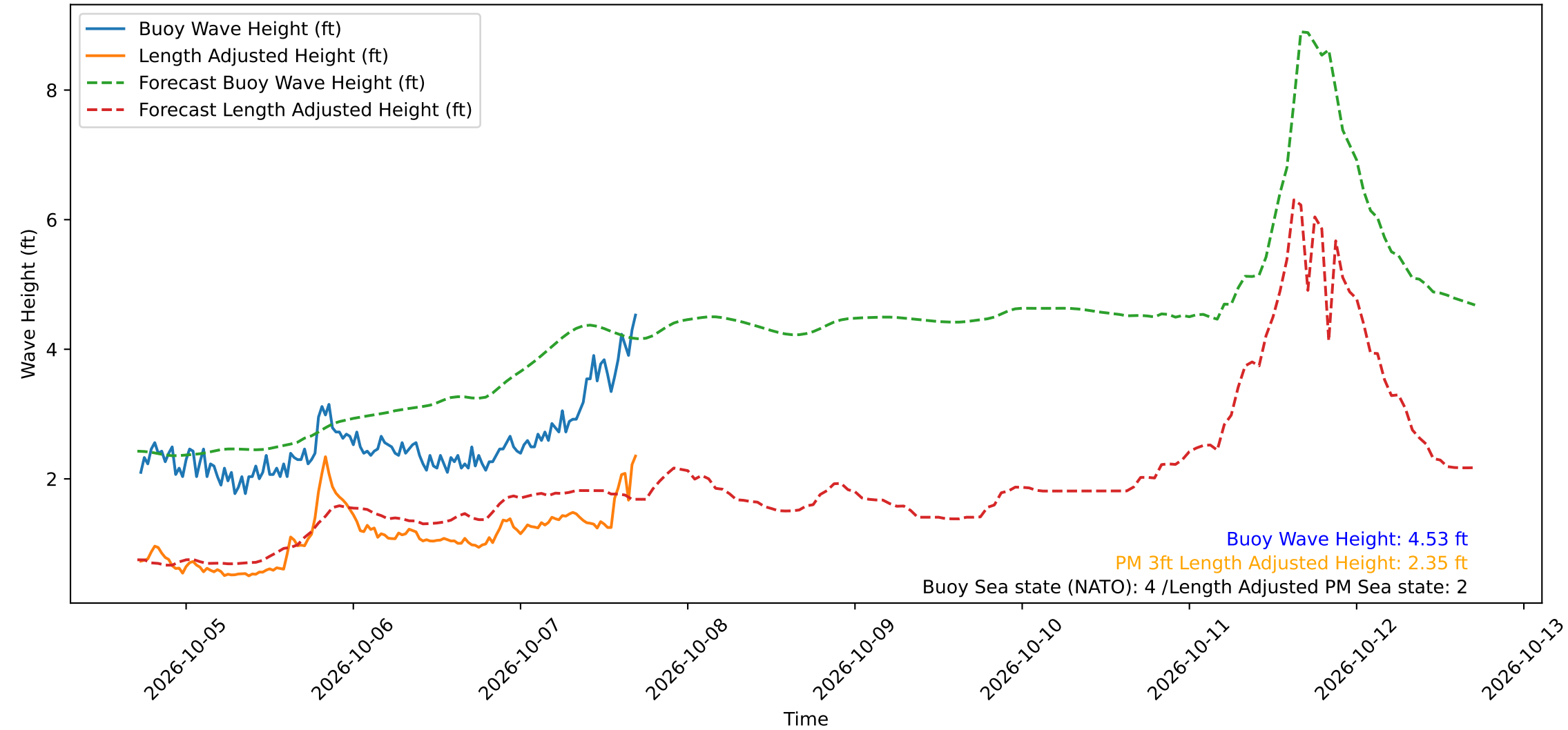
Wave Heights over Time for Green Beach at 2026-10-07 17:21:14
