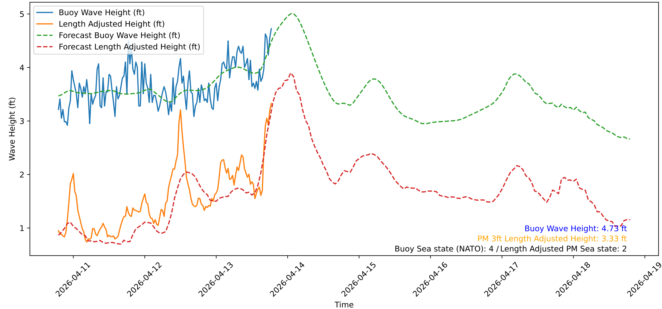
Wave Heights over Time for Green Beach at 2026-04-13 19:11:12
