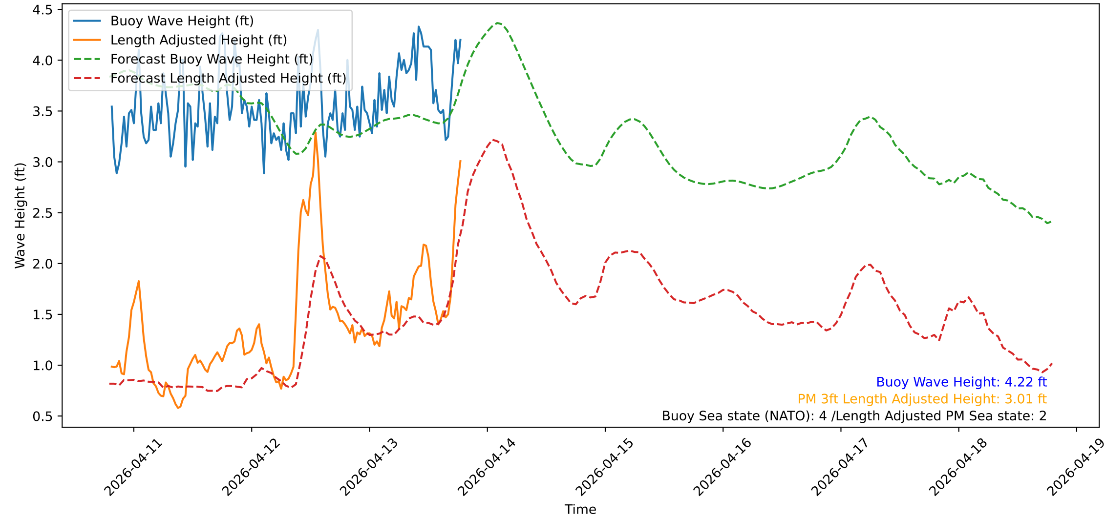
Wave Heights over Time for Red Beach at 2026-04-13 19:10:50
