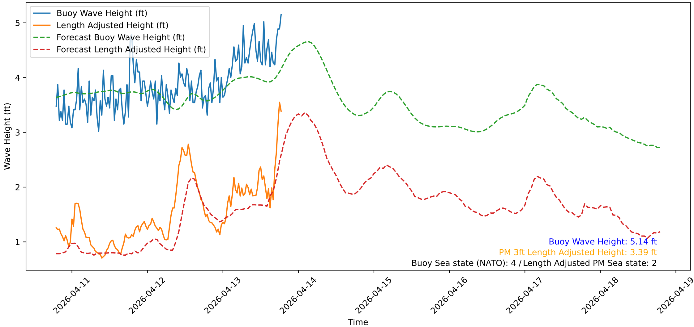
Wave Heights over Time for Oceanside Harbor at 2026-04-13 19:10:31
