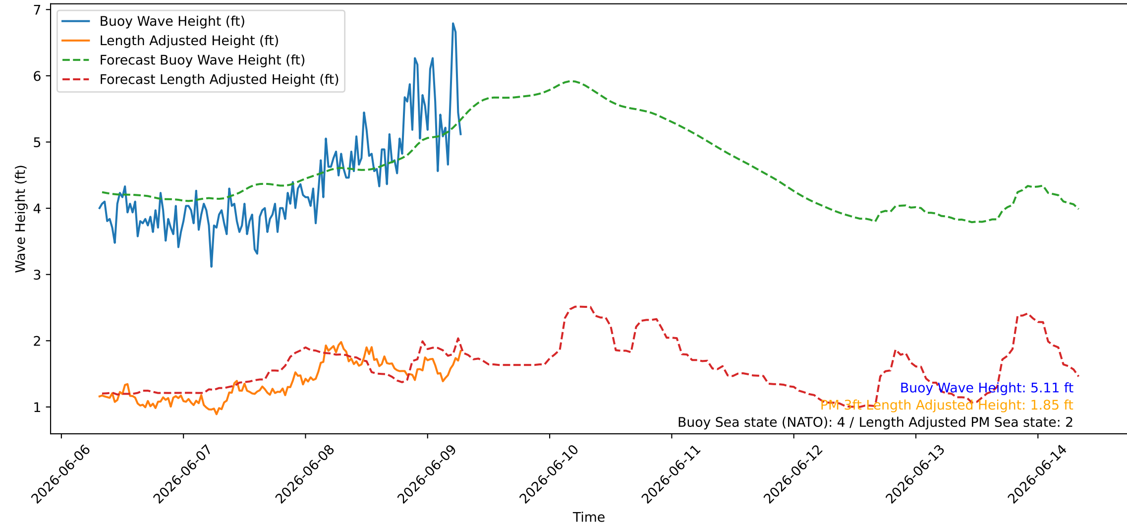
Wave Heights over Time for Green Beach at 2026-06-09 07:31:08
