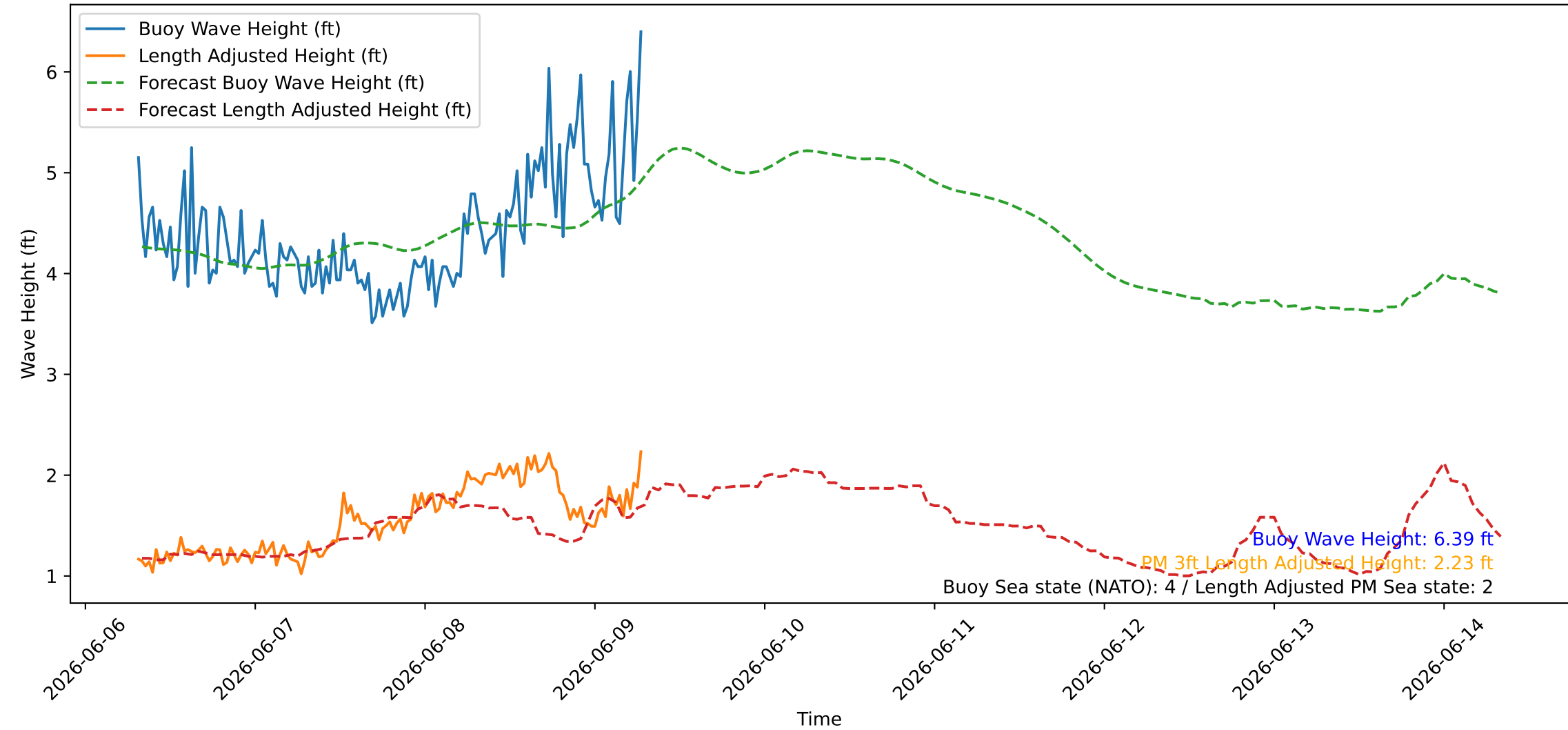
Wave Heights over Time for Oceanside Harbor at 2026-06-09 07:30:26
