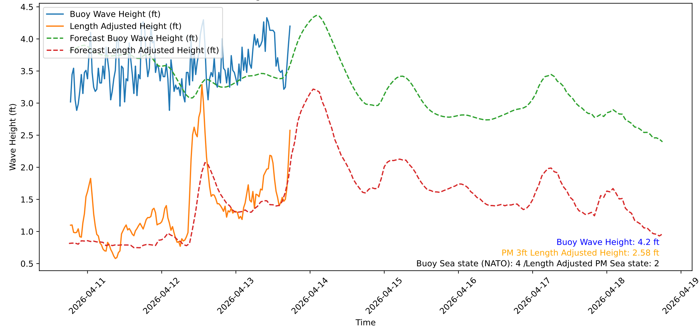
Wave Heights over Time for Red Beach at 2026-04-13 18:20:51
