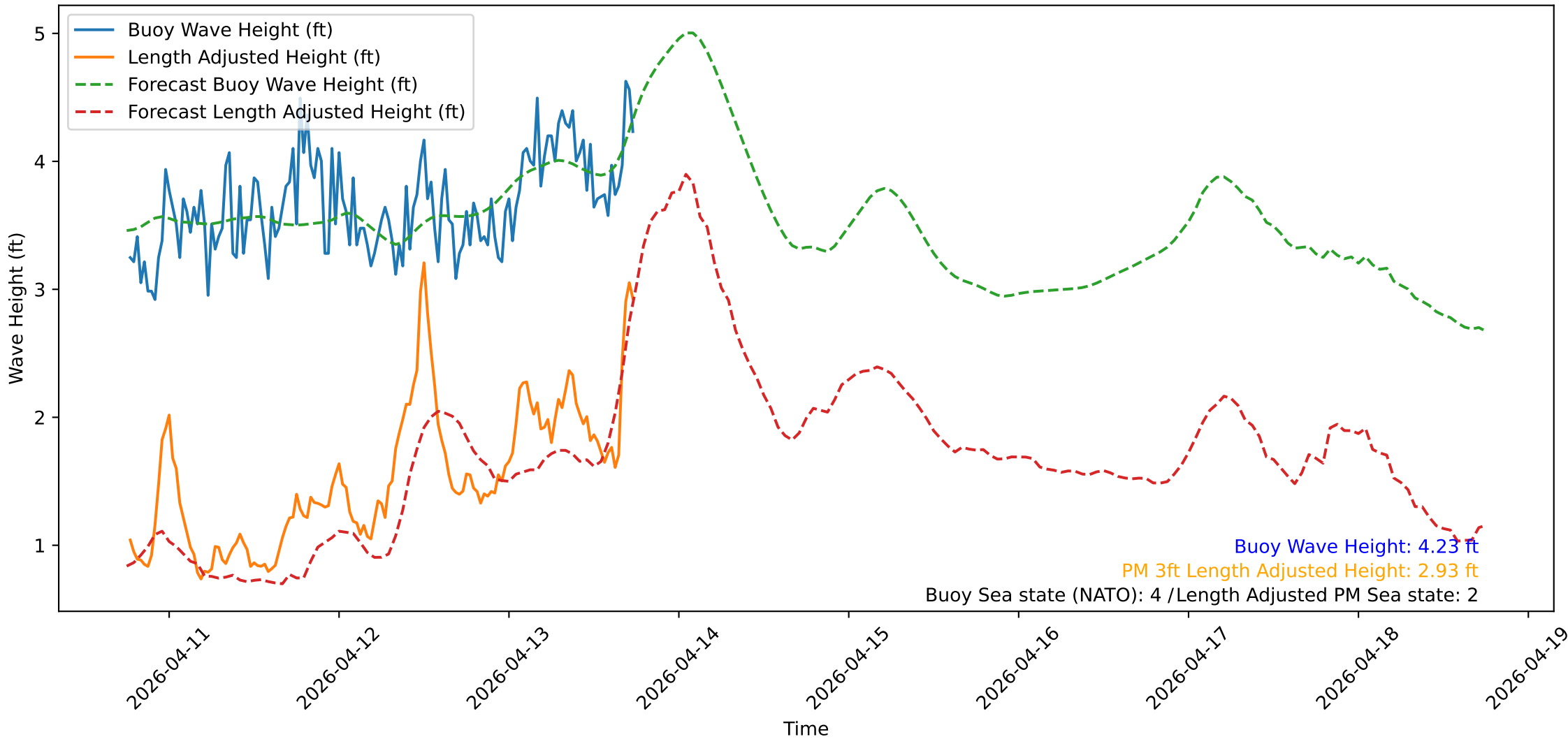
Wave Heights over Time for Green Beach at 2026-04-13 18:21:13
