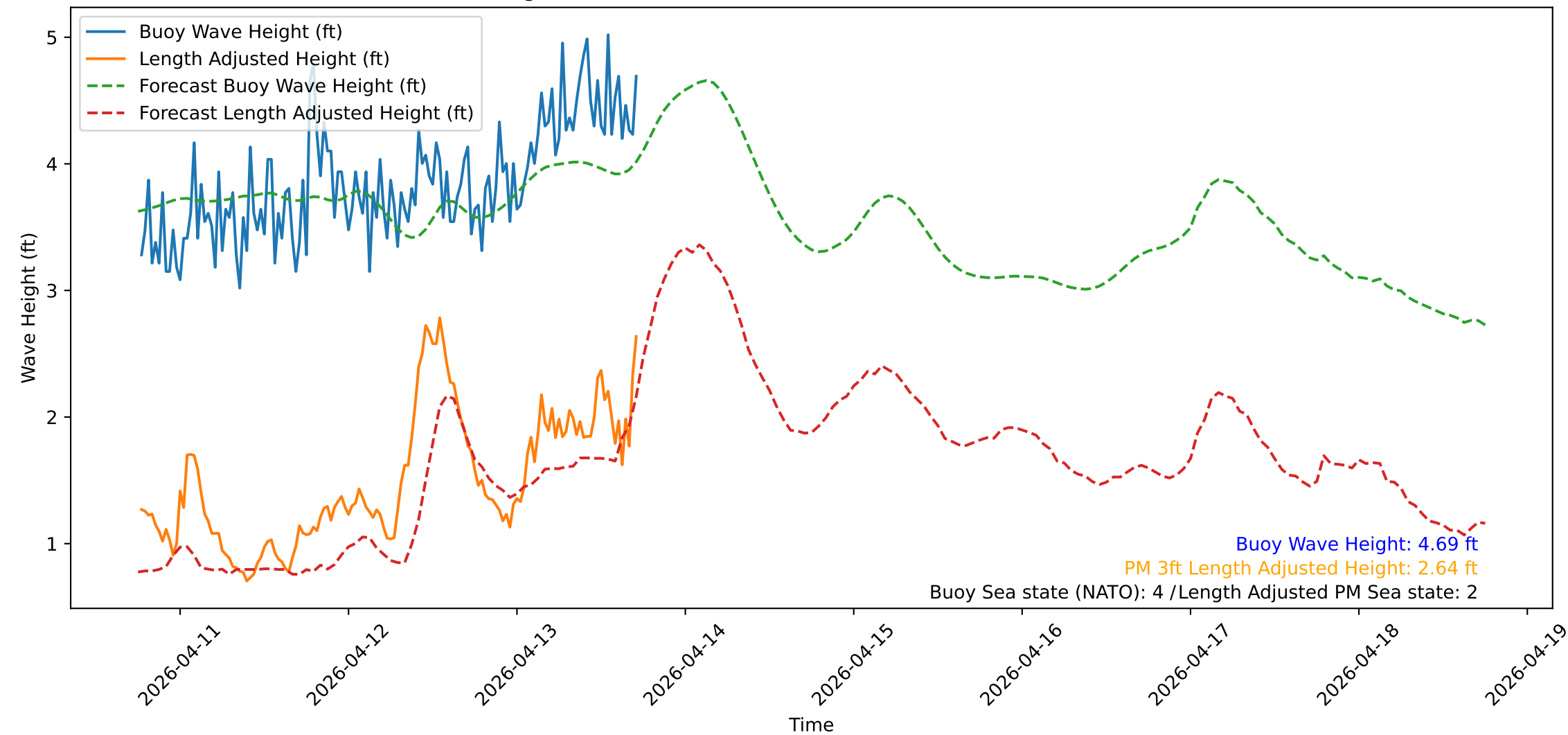
Wave Heights over Time for Oceanside Harbor at 2026-04-13 18:20:31
