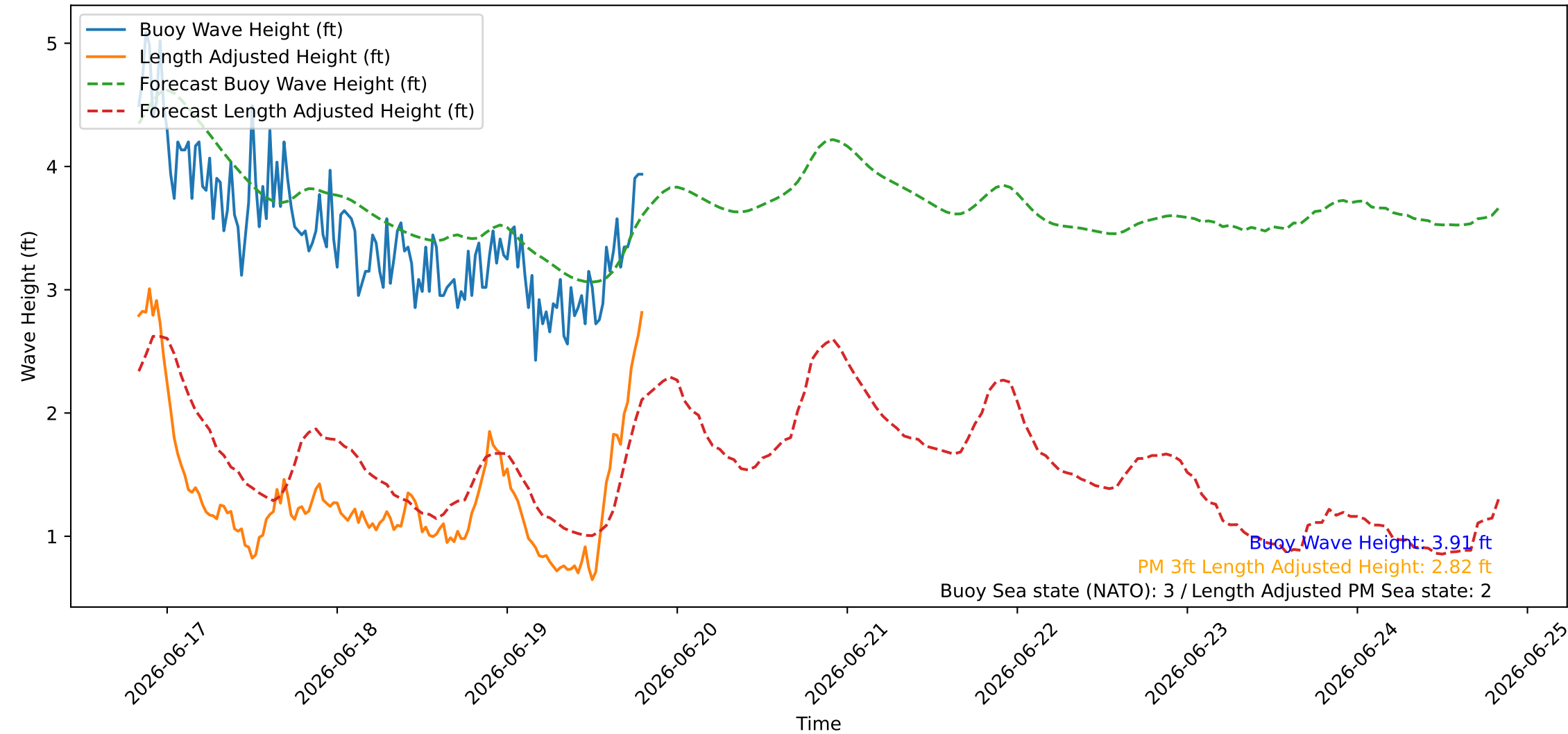
Wave Heights over Time for Green Beach at 2026-06-19 20:01:07
