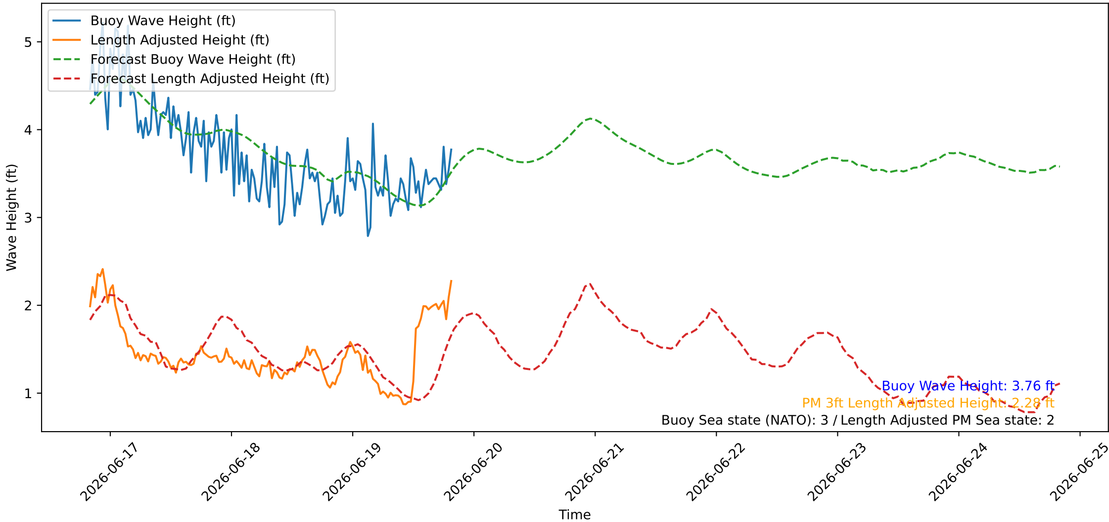
Wave Heights over Time for Oceanside Harbor at 2026-06-19 20:00:26
