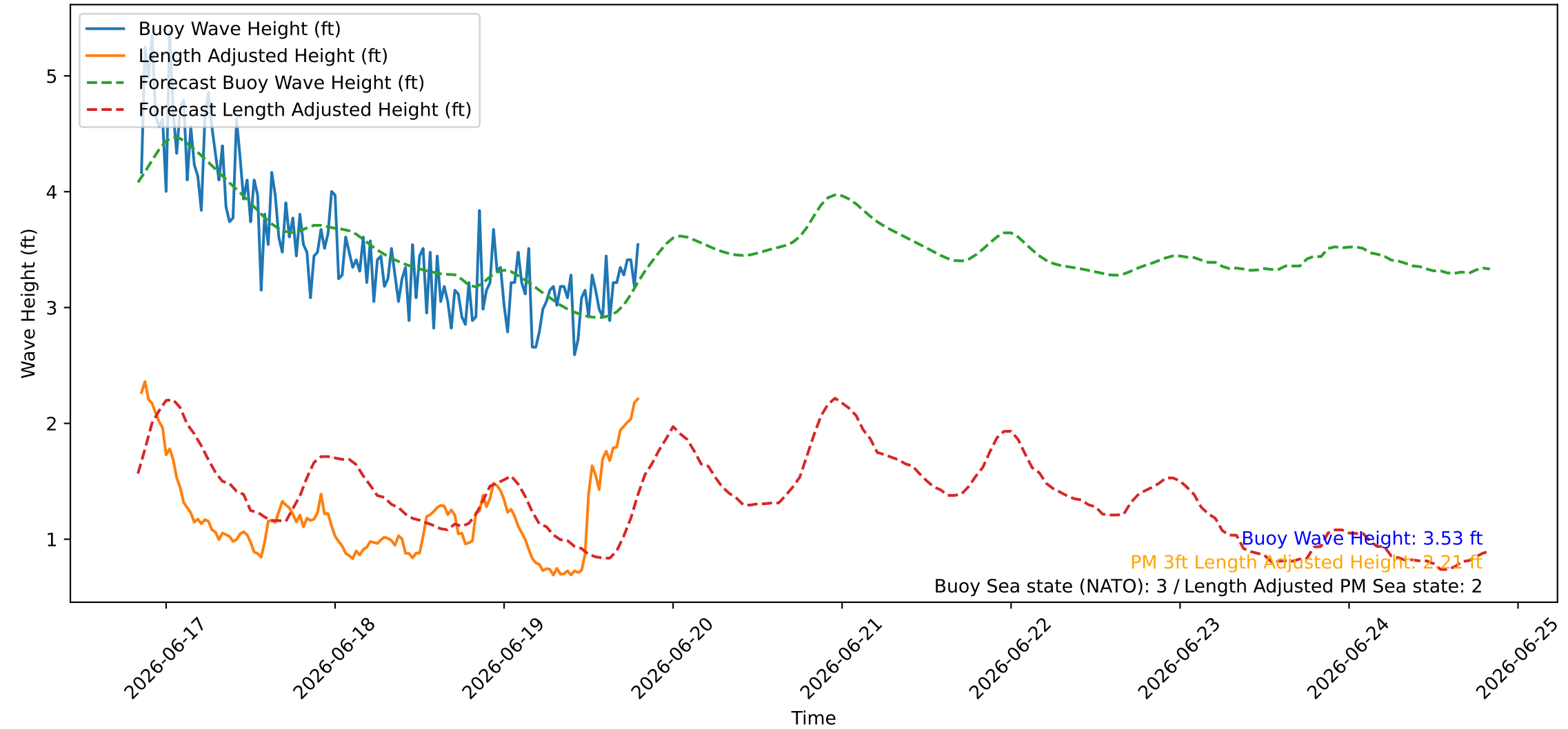
Wave Heights over Time for Red Beach at 2026-06-19 20:00:45
