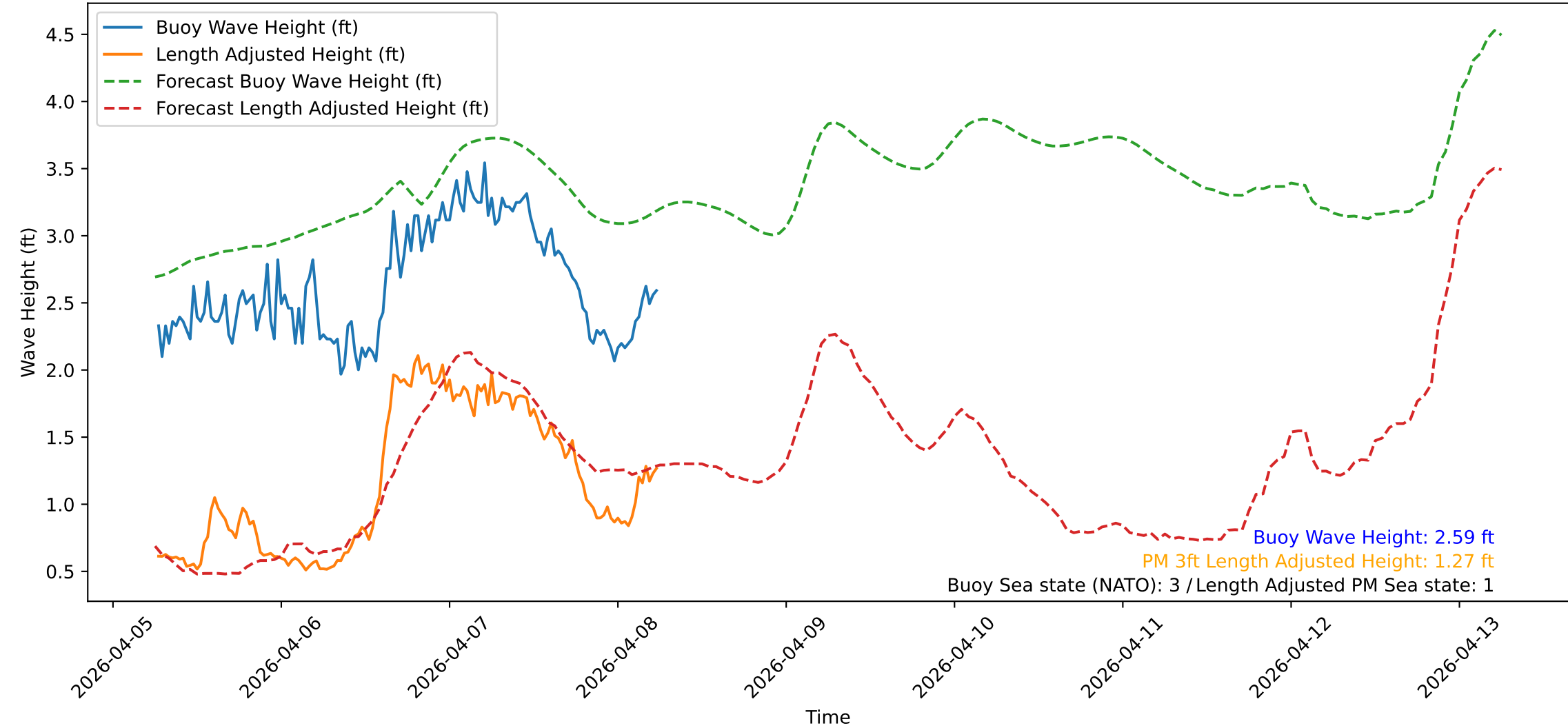
Wave Heights over Time for Red Beach at 2026-04-08 06:20:48
