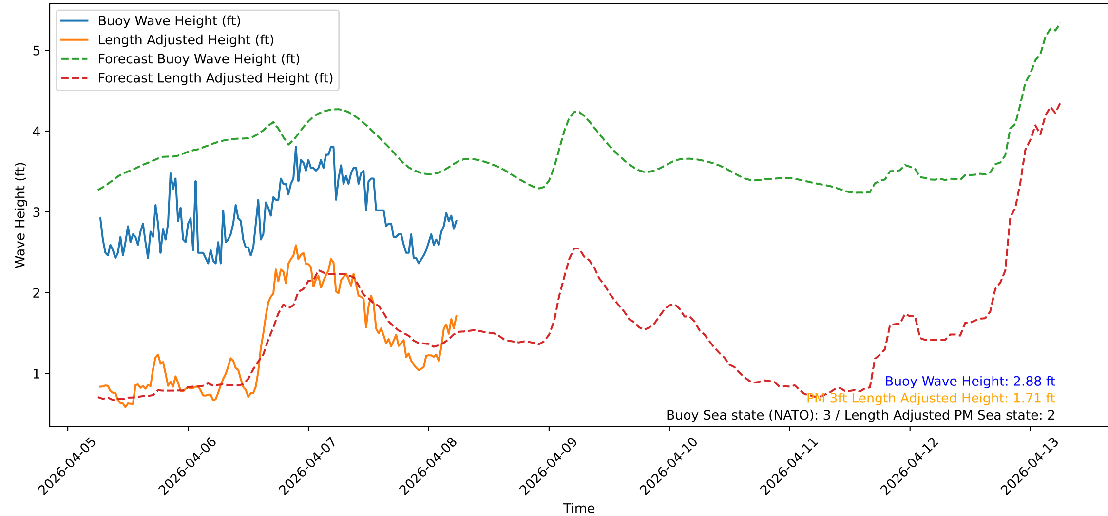
Wave Heights over Time for Green Beach at 2026-04-08 06:21:10
