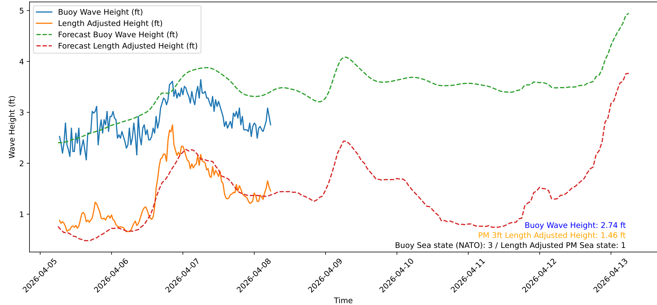
Wave Heights over Time for Oceanside Harbor at 2026-04-08 06:20:32
