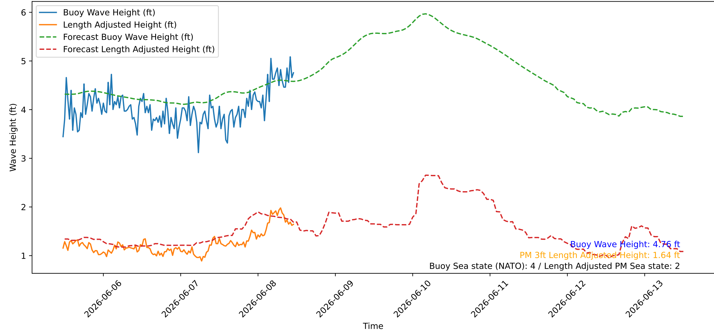
Wave Heights over Time for Green Beach at 2026-06-08 11:41:08
