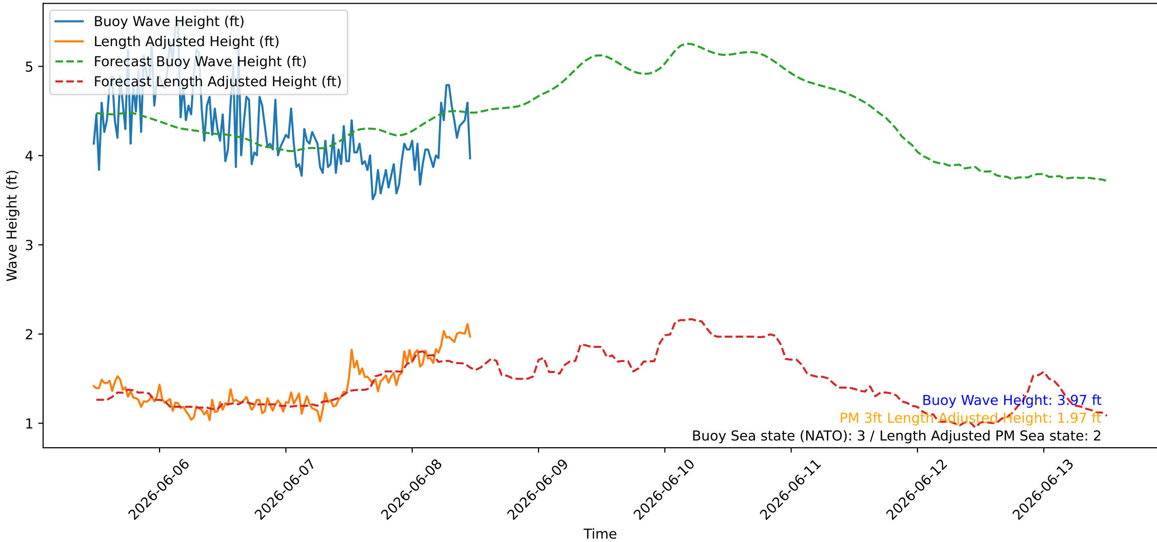
Wave Heights over Time for Oceanside Harbor at 2026-06-08 11:40:26
