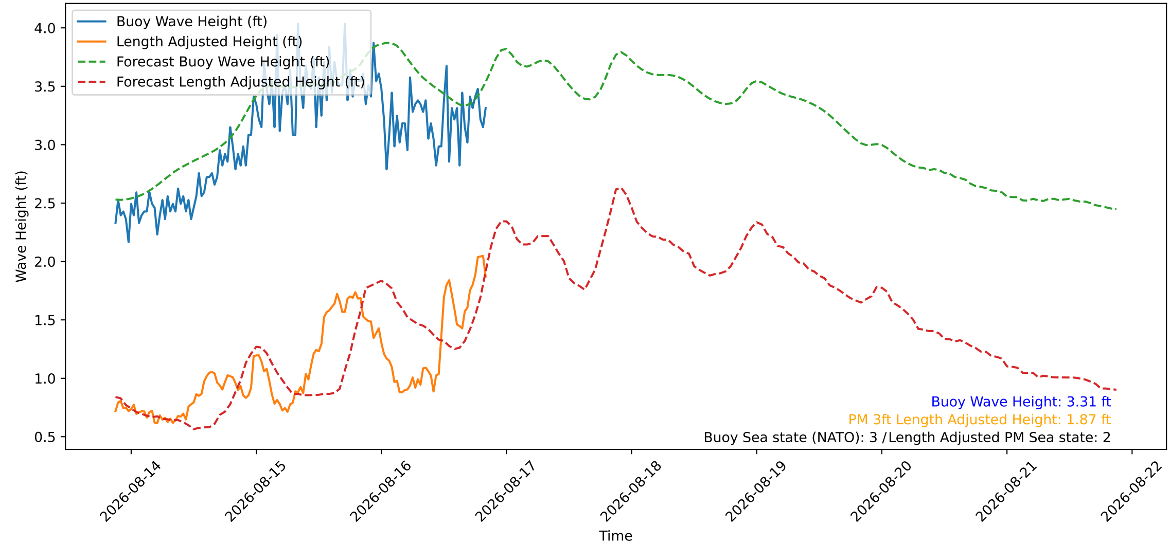
Wave Heights over Time for Red Beach at 2026-08-16 20:50:47
