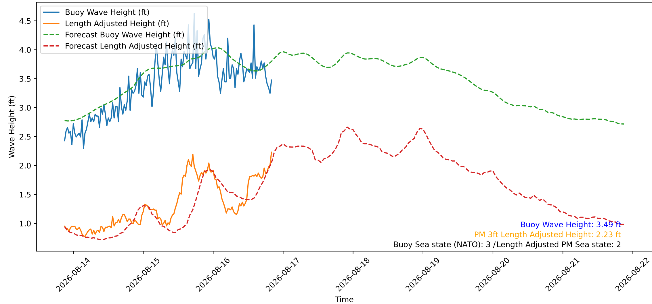
Wave Heights over Time for Oceanside Harbor at 2026-08-16 20:50:26
