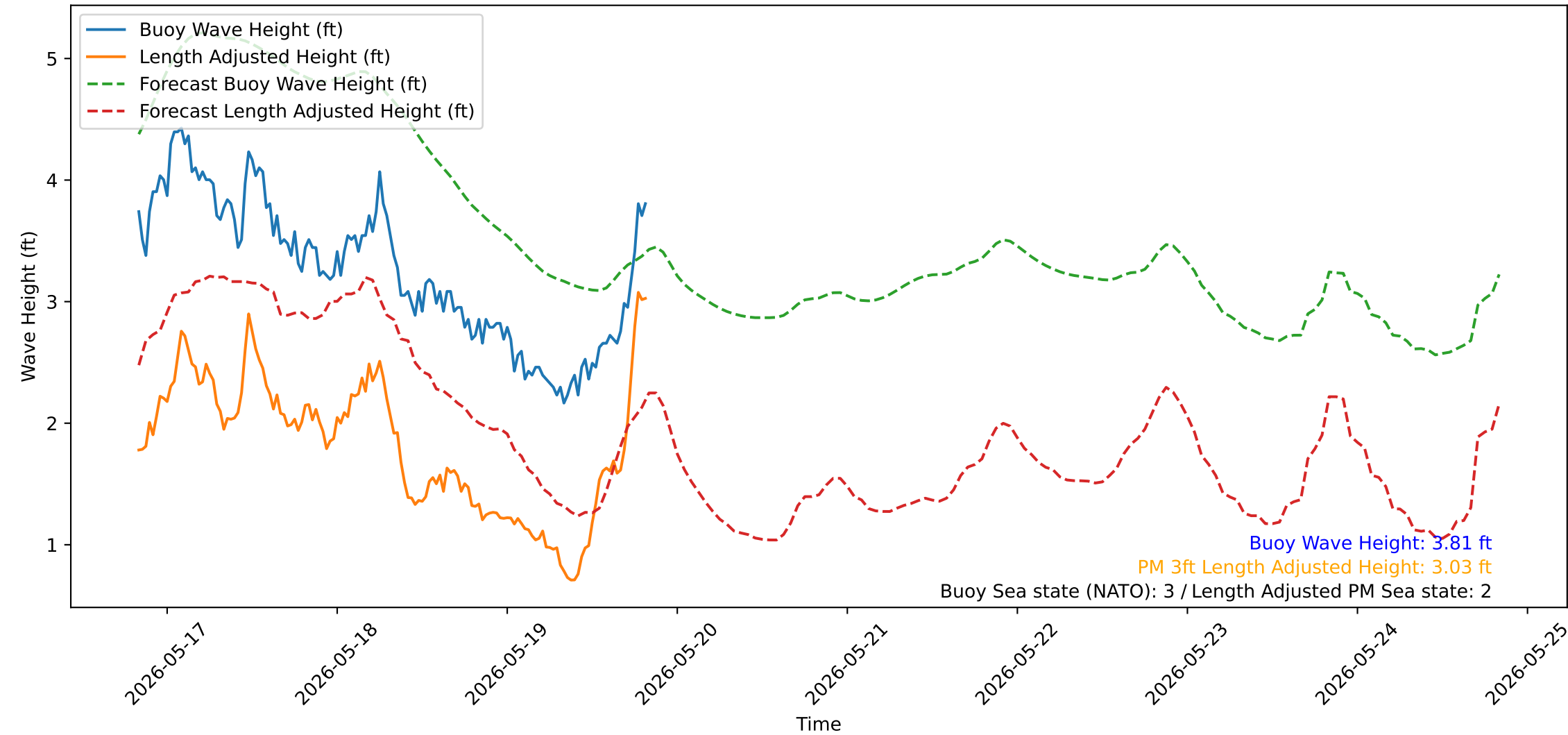
Wave Heights over Time for Green Beach at 2026-05-19 20:11:15
