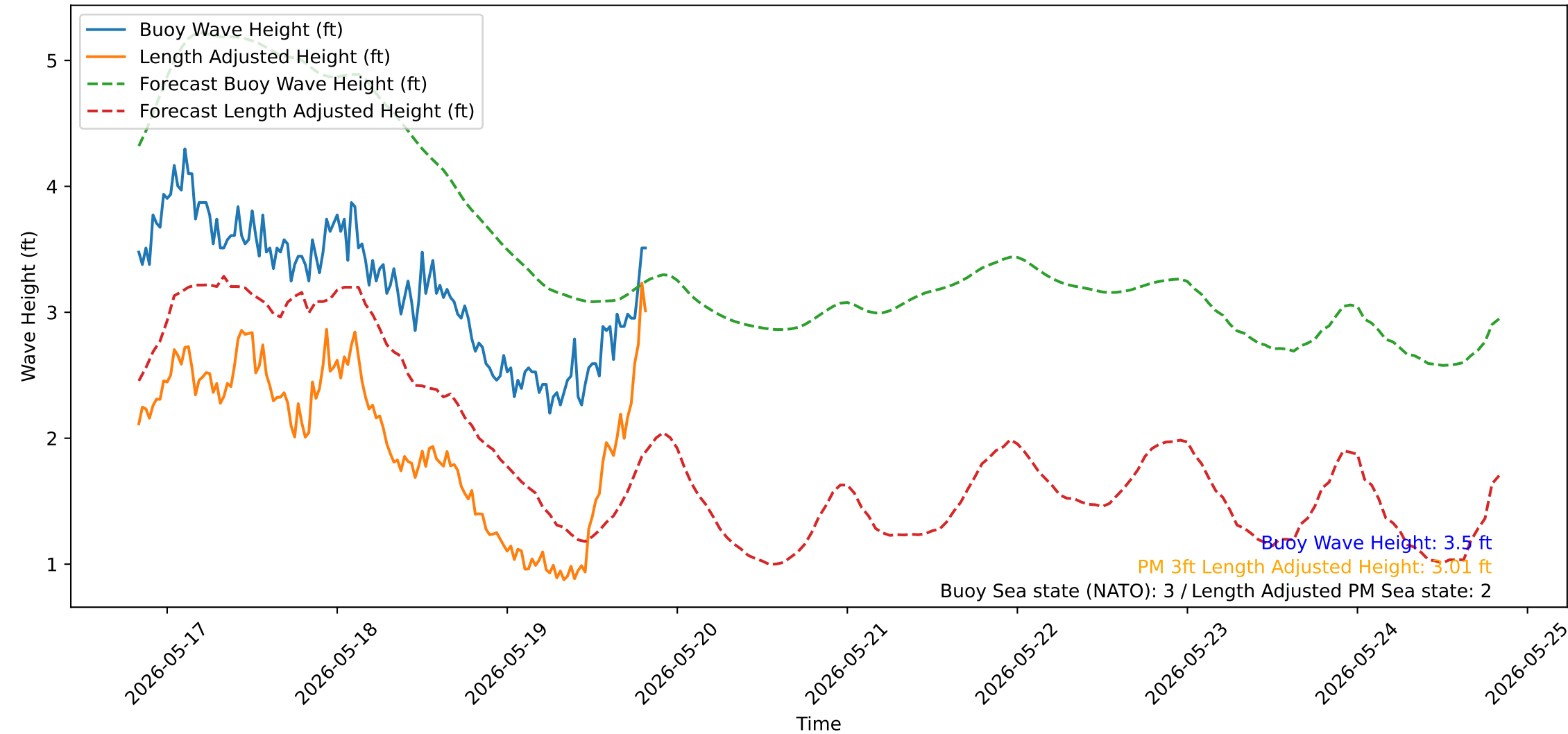
Wave Heights over Time for Oceanside Harbor at 2026-05-19 20:10:32
