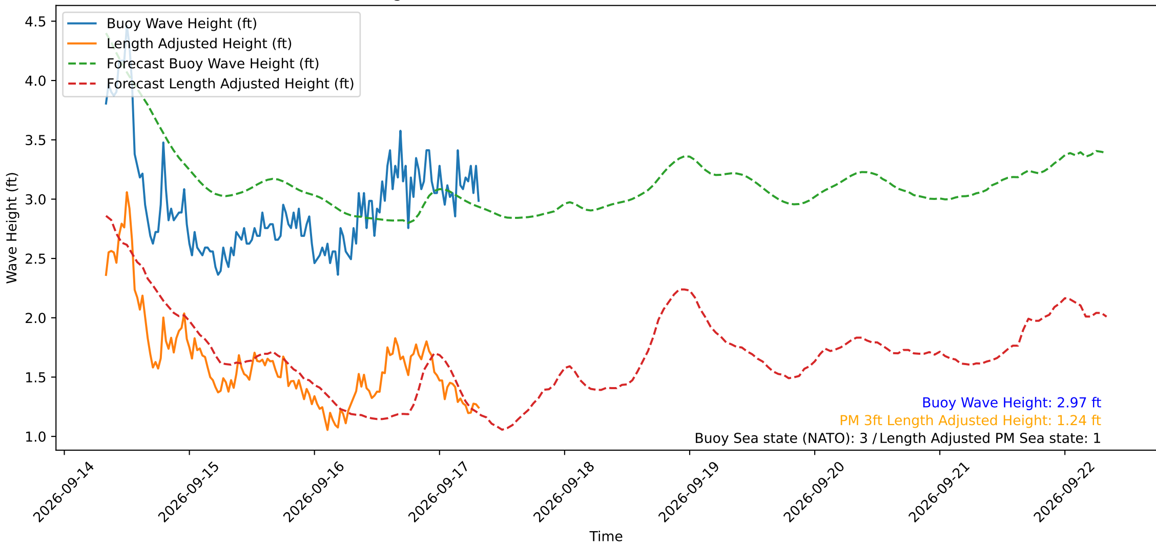
Wave Heights over Time for Oceanside Harbor at 2026-09-17 08:00:30
