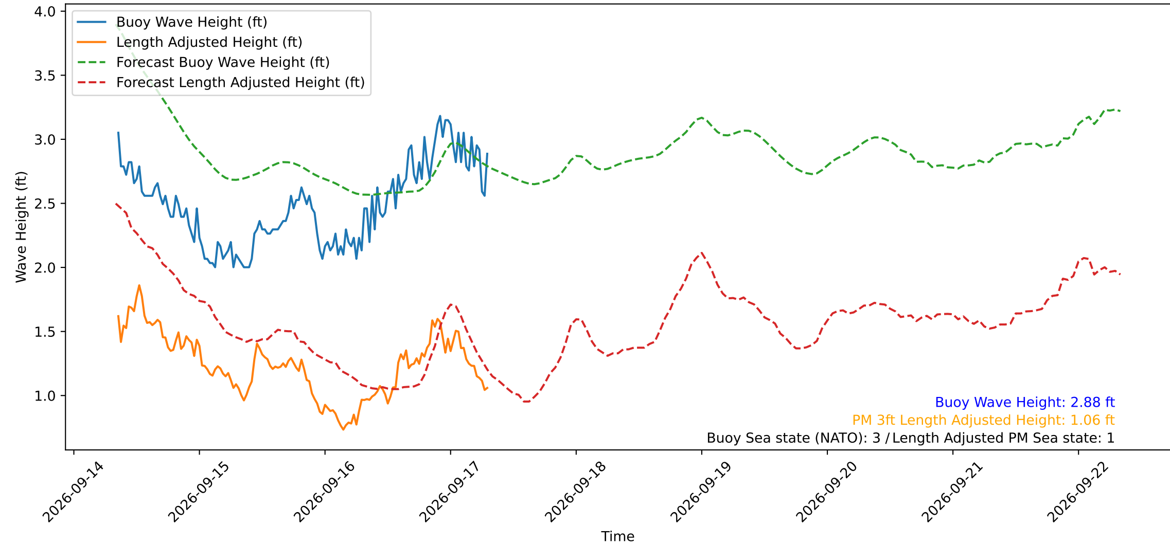
Wave Heights over Time for Red Beach at 2026-09-17 08:00:50
