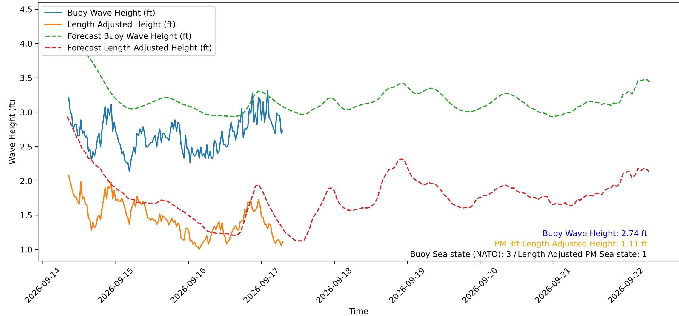
Wave Heights over Time for Green Beach at 2026-09-17 08:01:12
