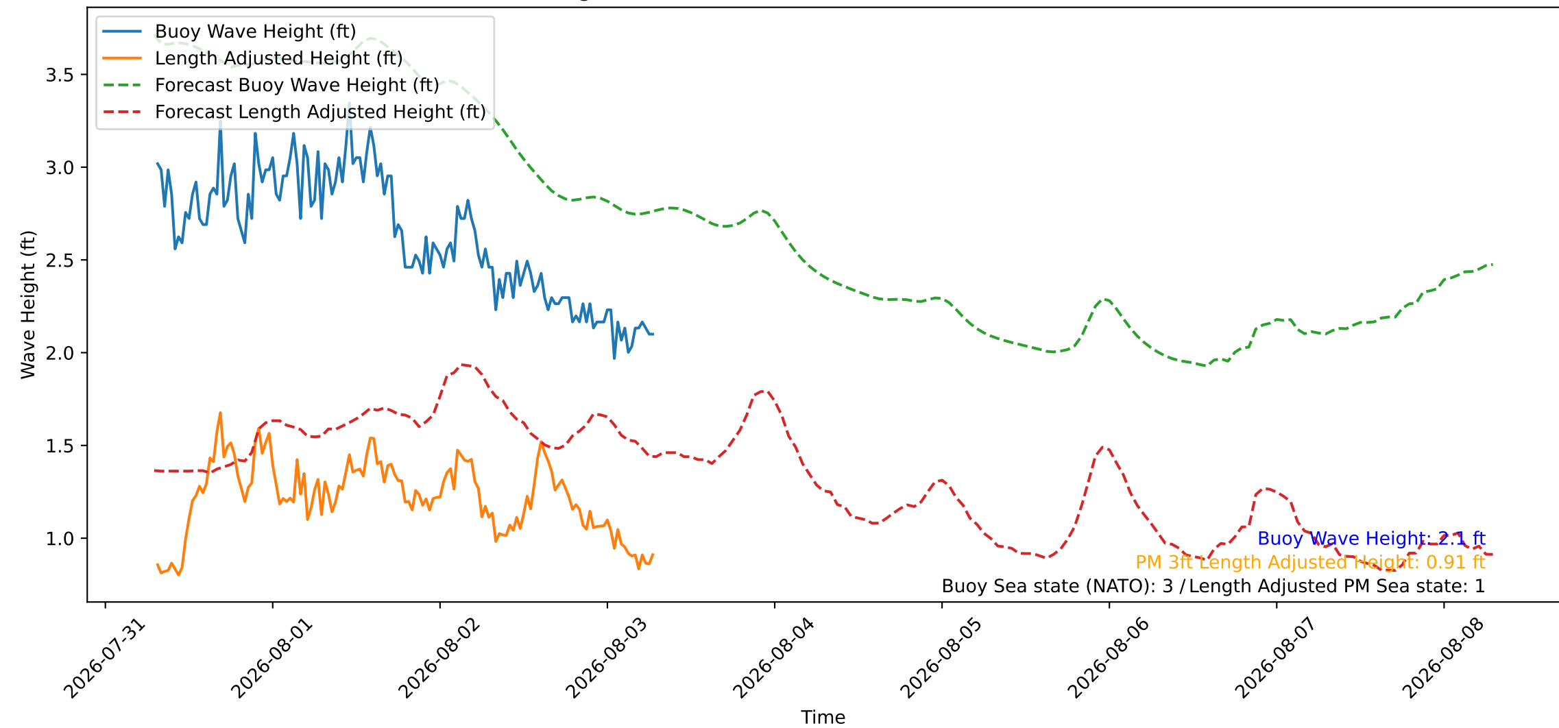
Wave Heights over Time for Red Beach at 2026-08-03 07:10:46
