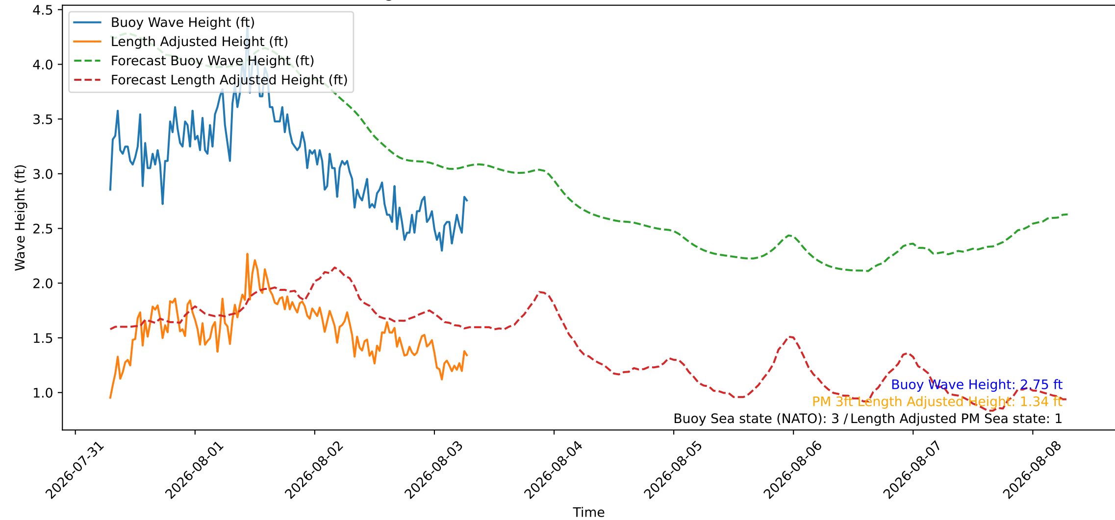
Wave Heights over Time for Oceanside Harbor at 2026-08-03 07:10:26
