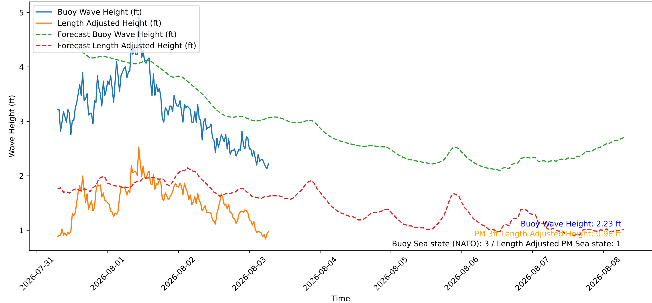
Wave Heights over Time for Green Beach at 2026-08-03 07:11:08
