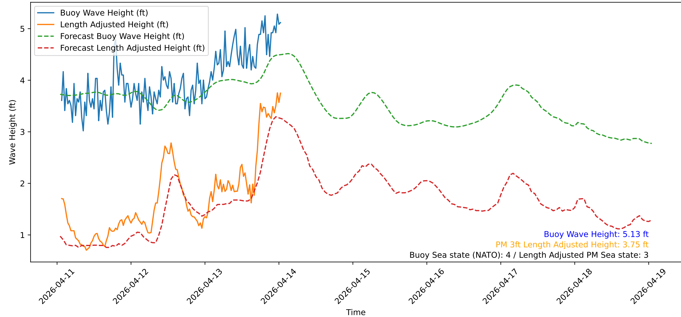
Wave Heights over Time for Oceanside Harbor at 2026-04-14 01:20:31
