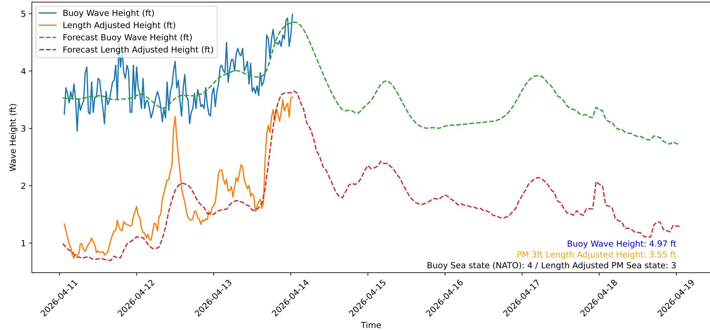
Wave Heights over Time for Green Beach at 2026-04-14 01:21:15
