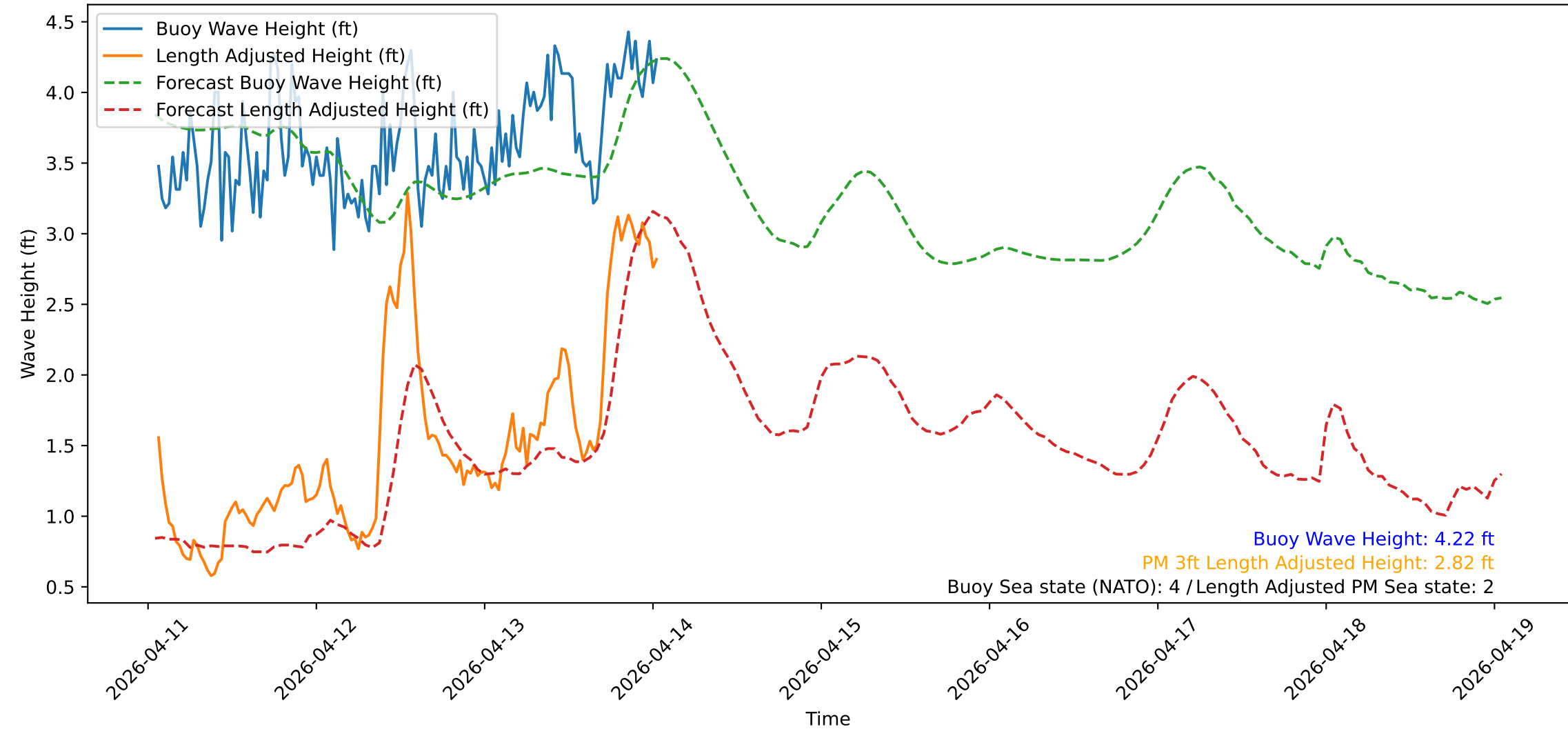
Wave Heights over Time for Red Beach at 2026-04-14 01:20:52
