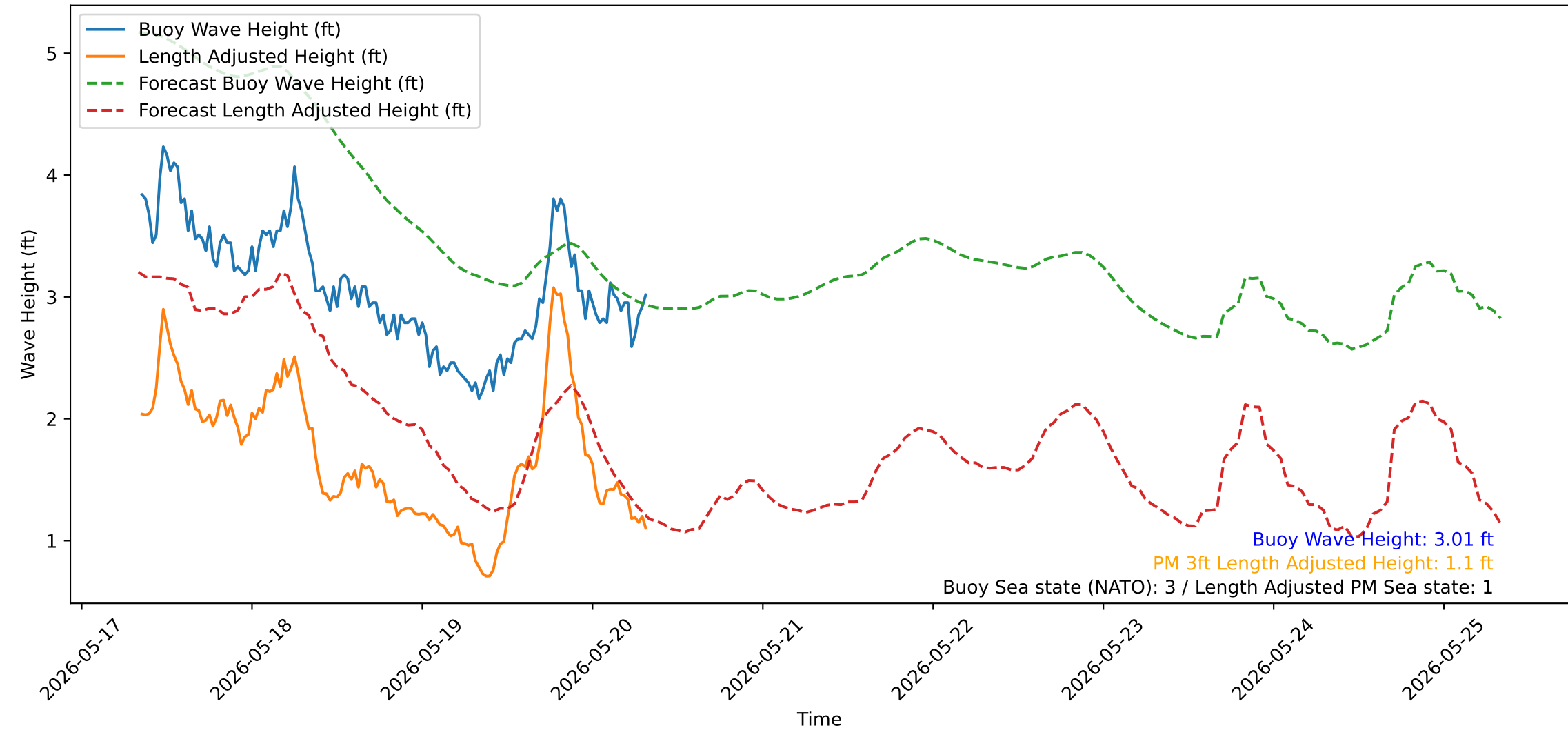
Wave Heights over Time for Green Beach at 2026-05-20 08:21:14
