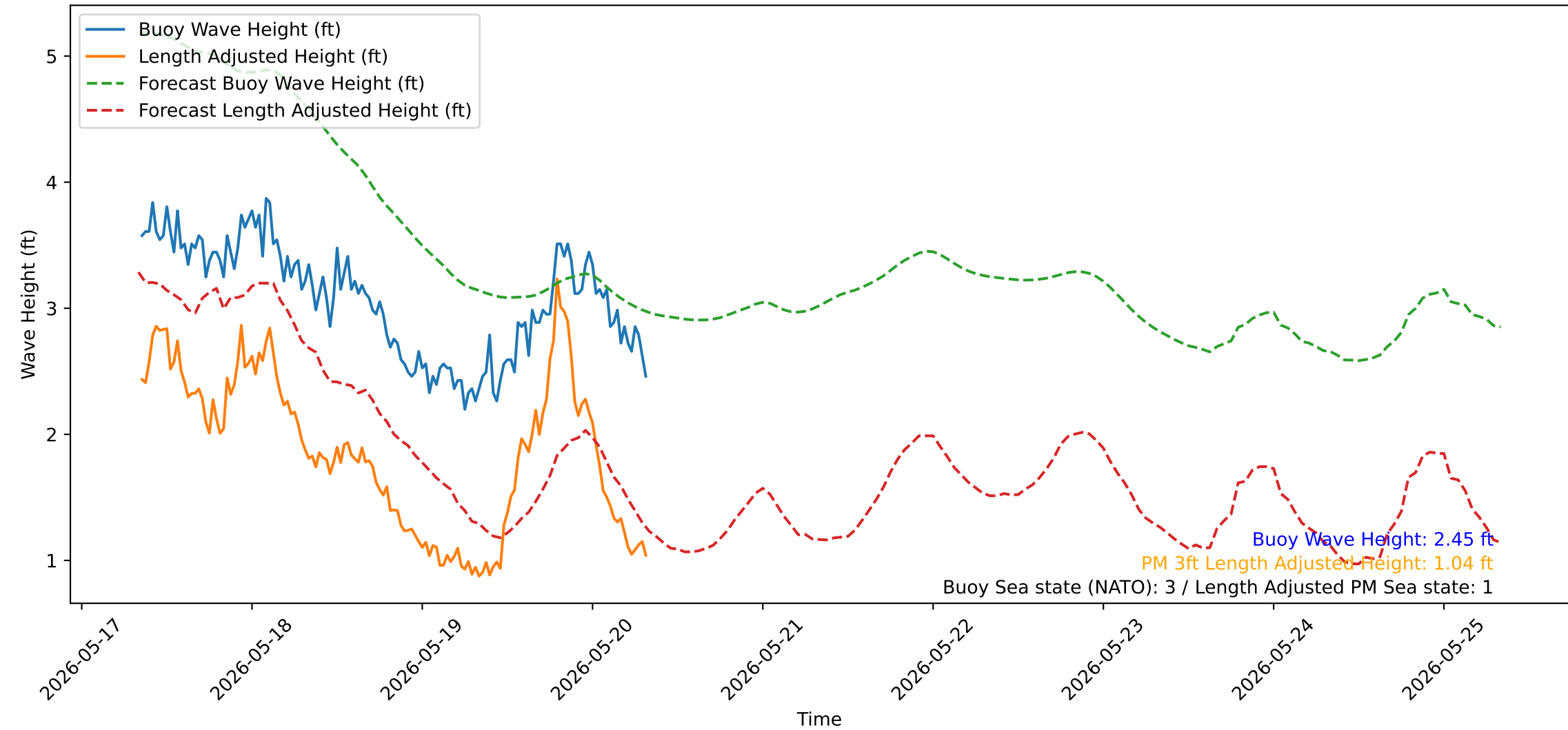
Wave Heights over Time for Oceanside Harbor at 2026-05-20 08:20:31
