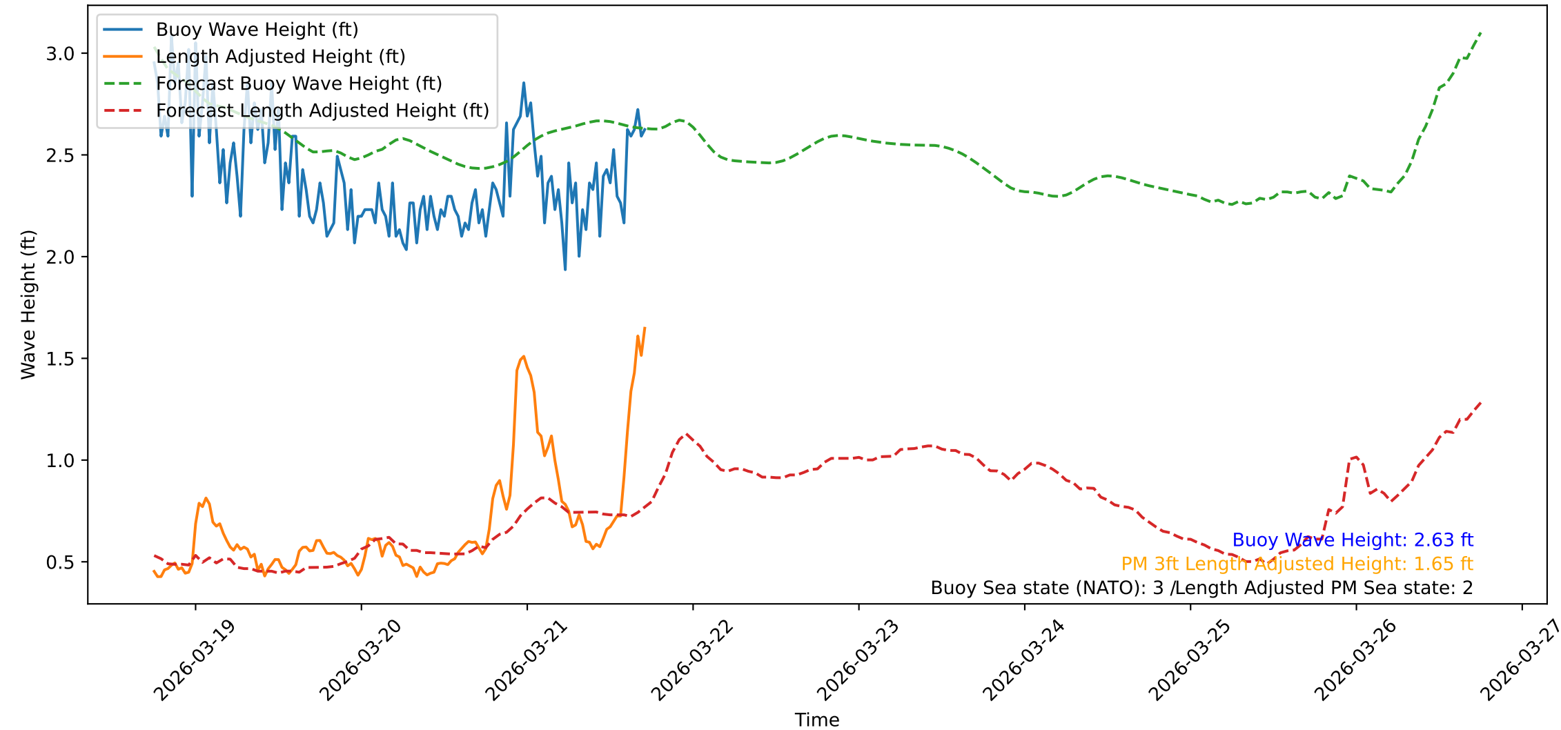
Wave Heights over Time for Green Beach at 2026-03-21 17:51:10
