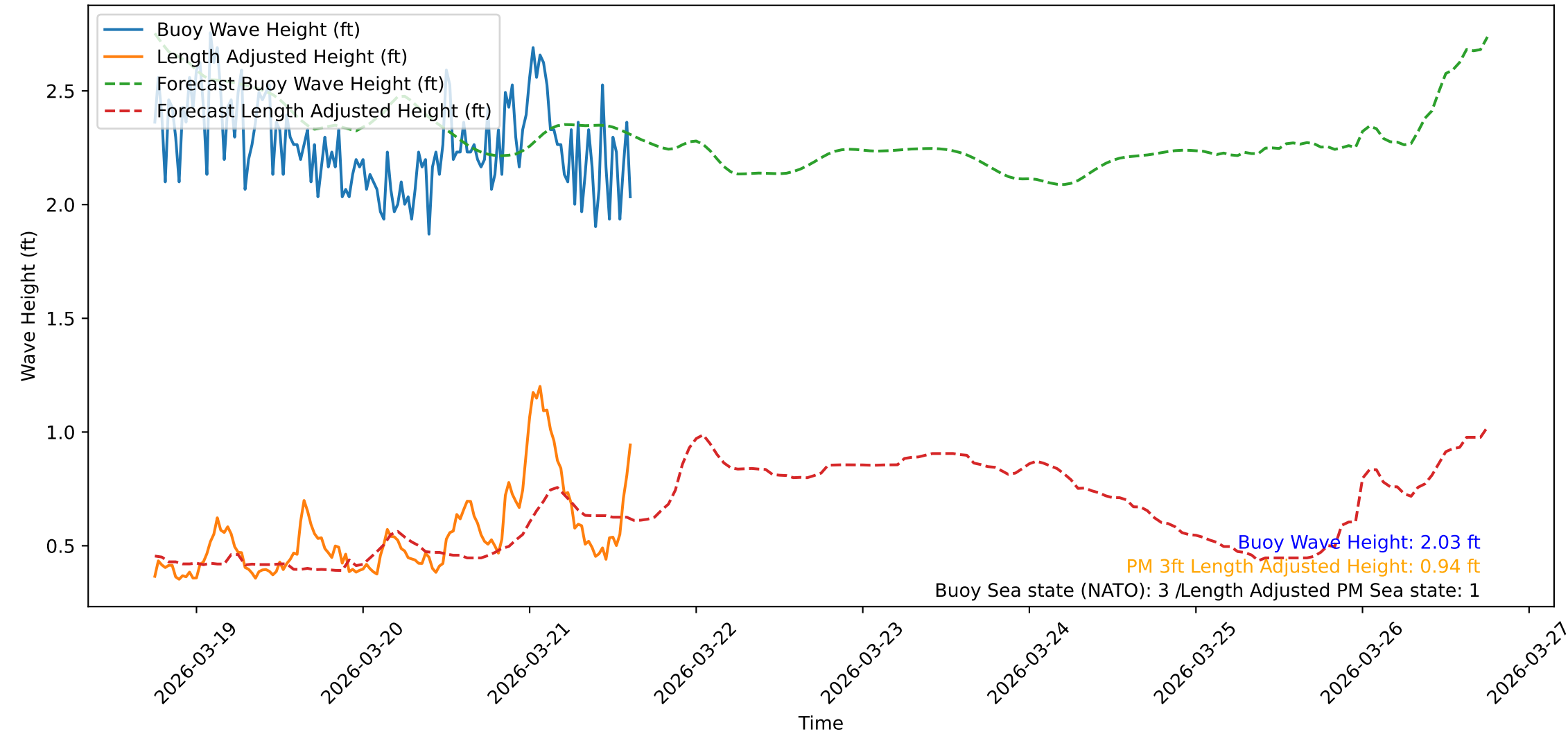
Wave Heights over Time for Red Beach at 2026-03-21 17:50:48
