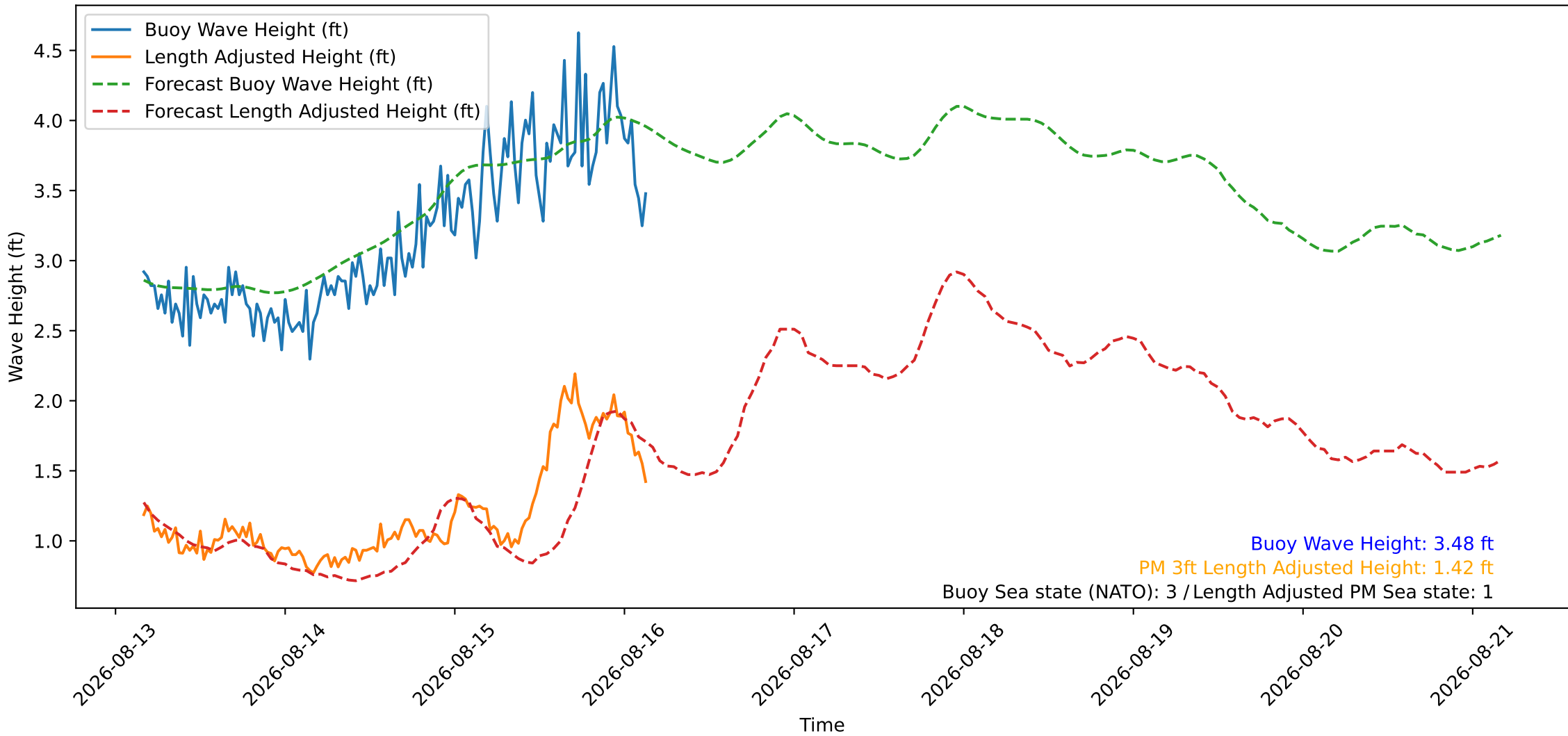
Wave Heights over Time for Oceanside Harbor at 2026-08-16 04:00:27
