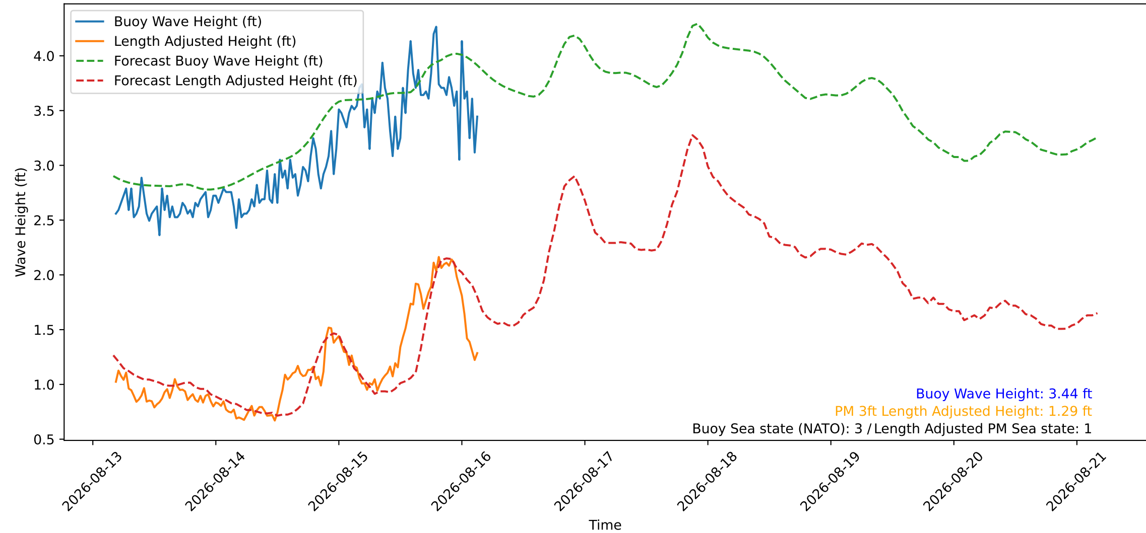
Wave Heights over Time for Green Beach at 2026-08-16 04:01:08
