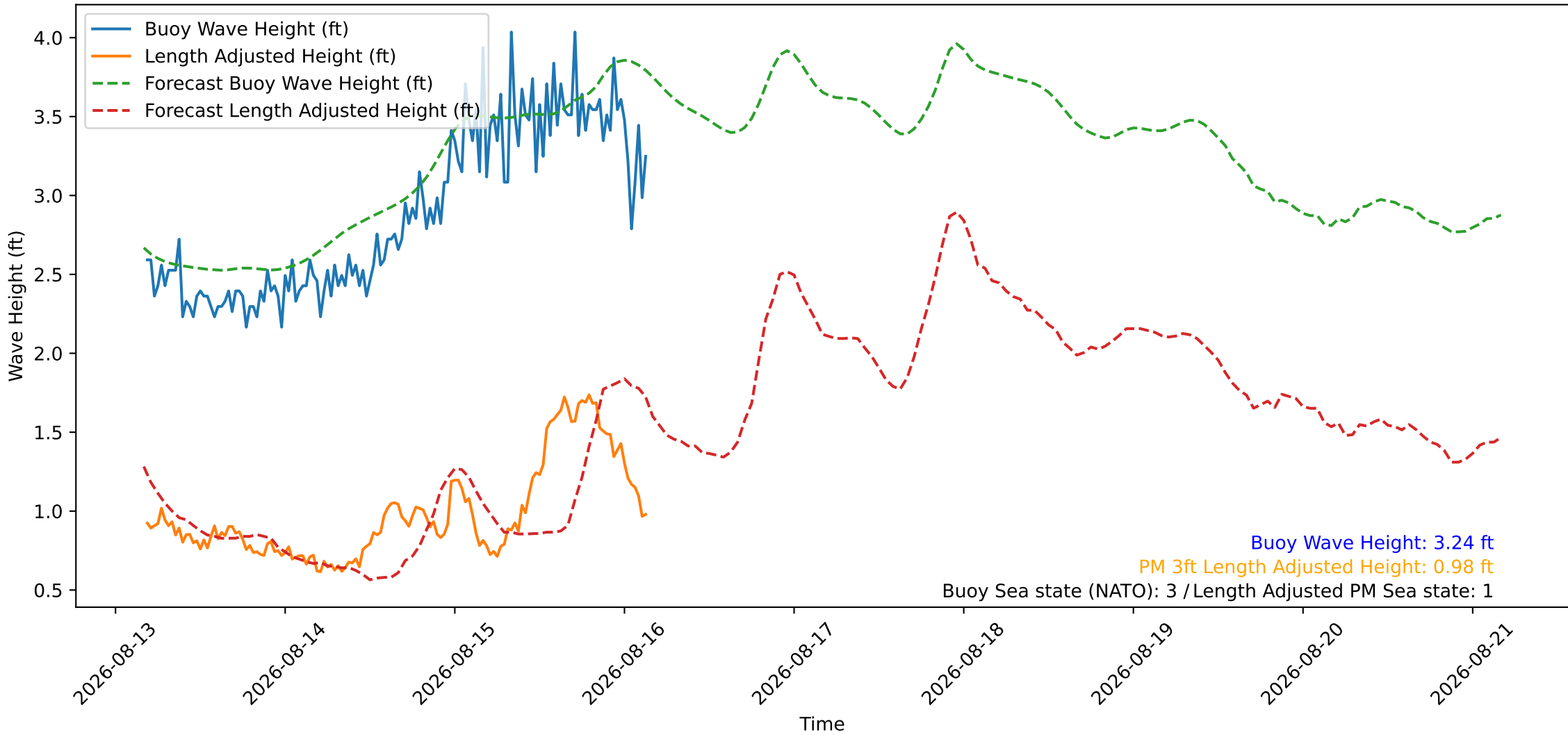
Wave Heights over Time for Red Beach at 2026-08-16 04:00:46
