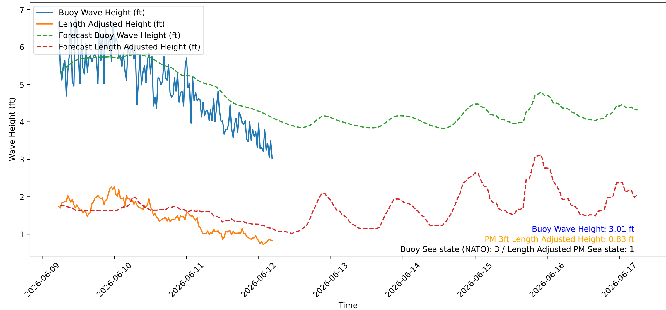
Wave Heights over Time for Green Beach at 2026-06-12 05:31:08
