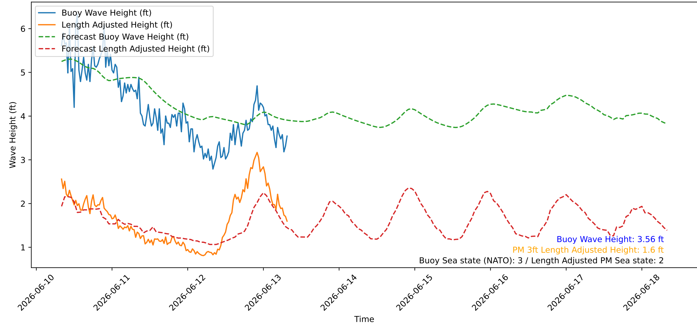
Wave Heights over Time for Oceanside Harbor at 2026-06-13 08:00:26
