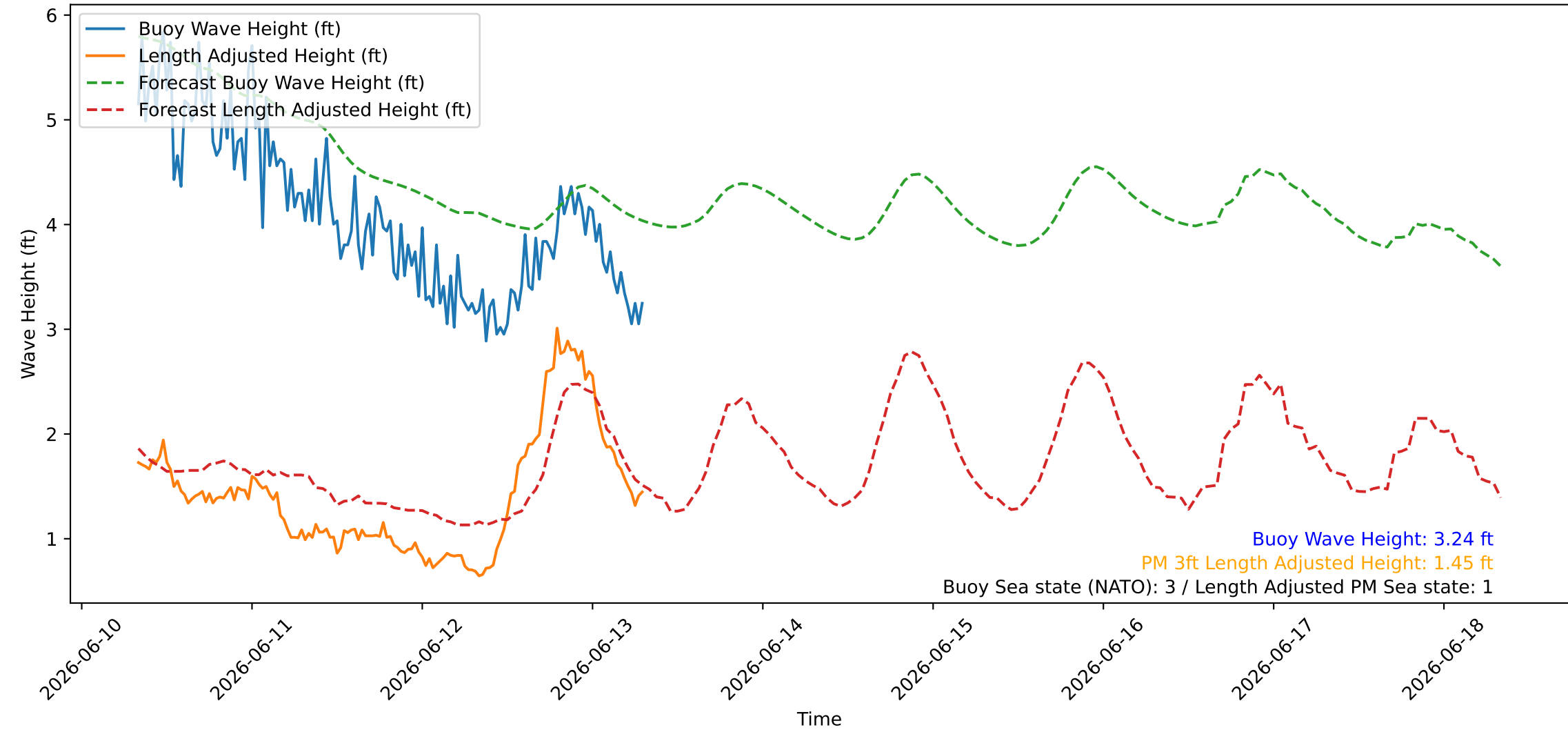
Wave Heights over Time for Green Beach at 2026-06-13 08:01:08
