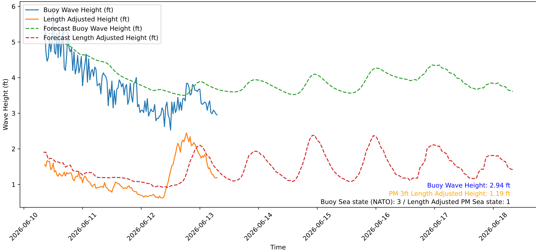
Wave Heights over Time for Red Beach at 2026-06-13 08:00:46
