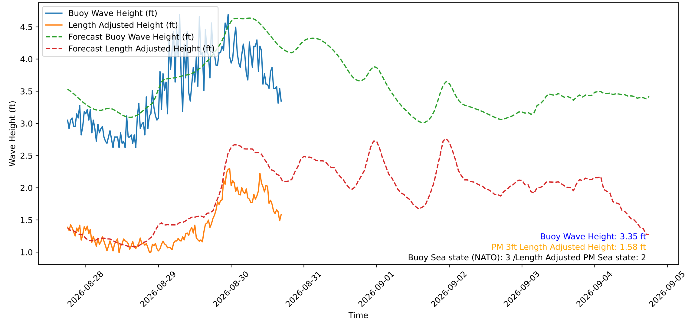
Wave Heights over Time for Red Beach at 2026-08-30 17:30:50
