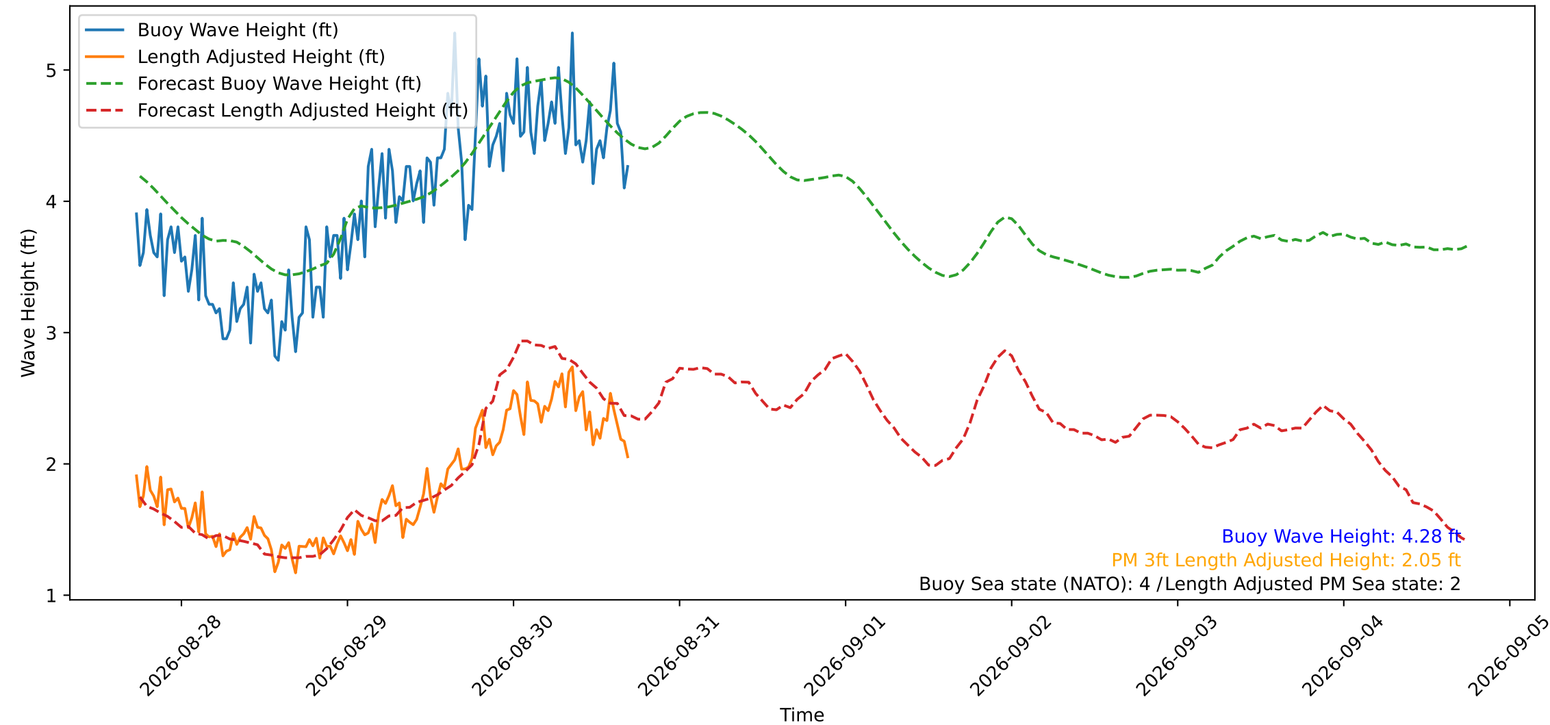
Wave Heights over Time for Oceanside Harbor at 2026-08-30 17:30:30
