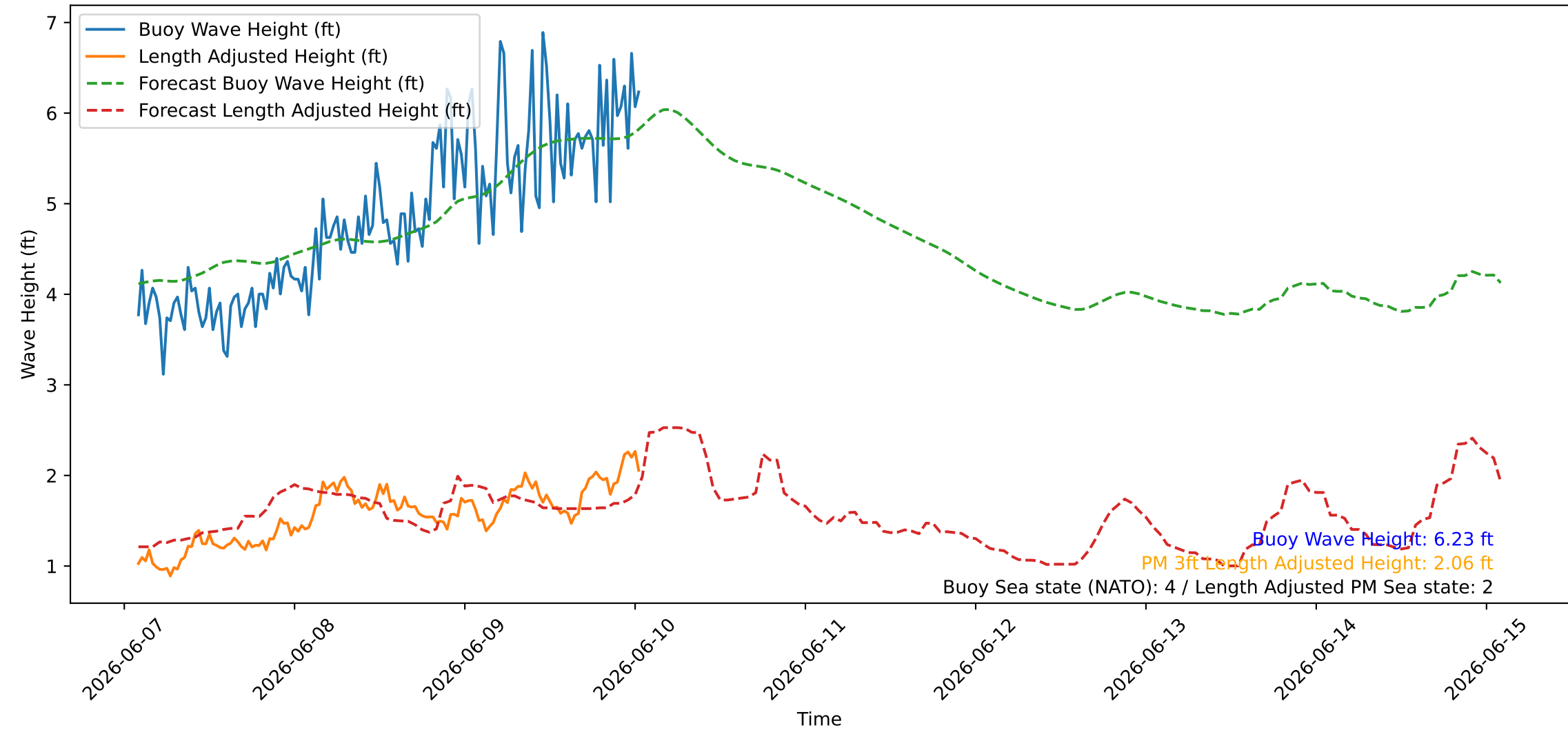
Wave Heights over Time for Green Beach at 2026-06-10 02:01:09
