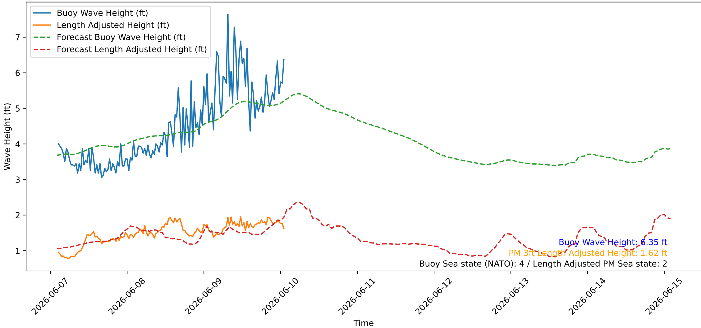
Wave Heights over Time for Red Beach at 2026-06-10 02:00:46
