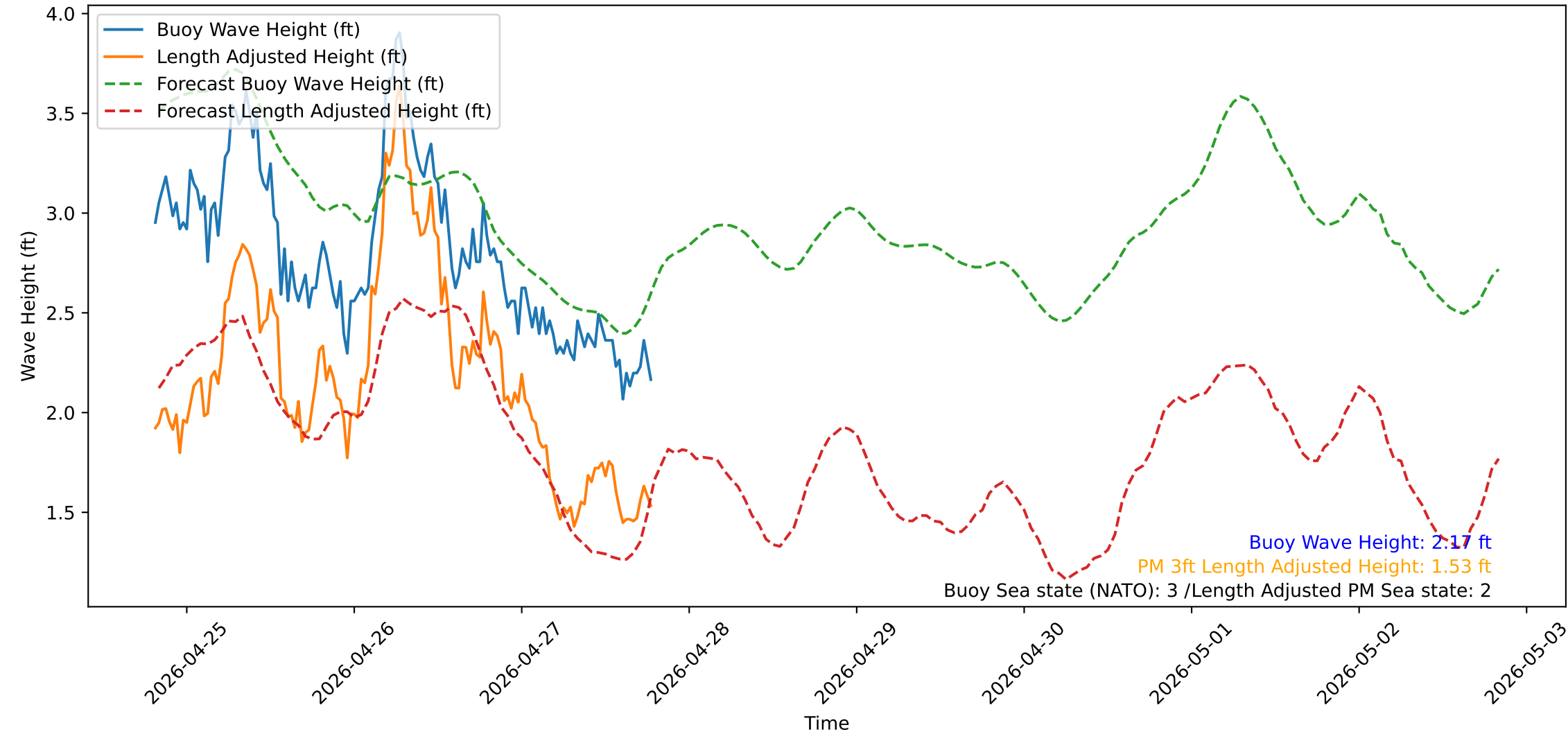
Wave Heights over Time for Oceanside Harbor at 2026-04-27 19:30:31
