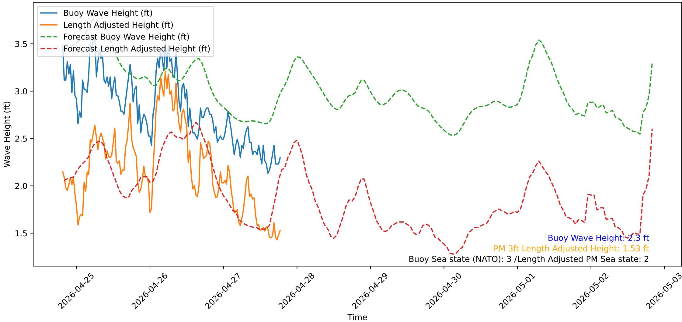
Wave Heights over Time for Green Beach at 2026-04-27 19:31:12
