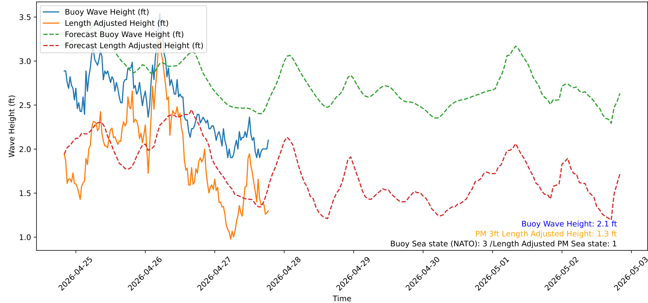
Wave Heights over Time for Red Beach at 2026-04-27 19:30:50
