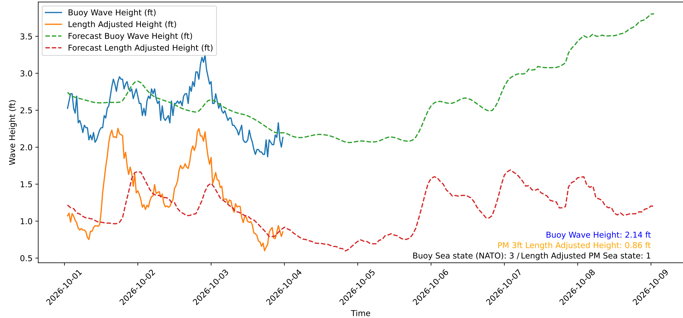
Wave Heights over Time for Red Beach at 2026-10-04 00:30:49
