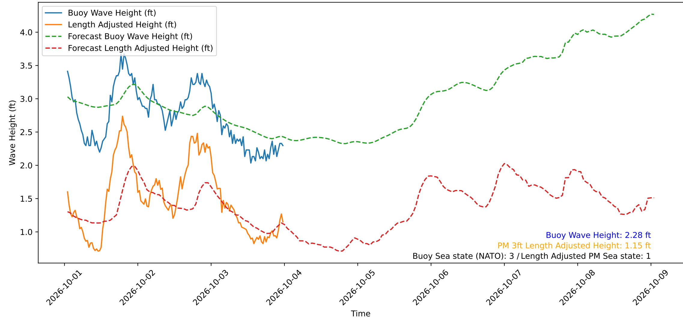
Wave Heights over Time for Green Beach at 2026-10-04 00:31:11
