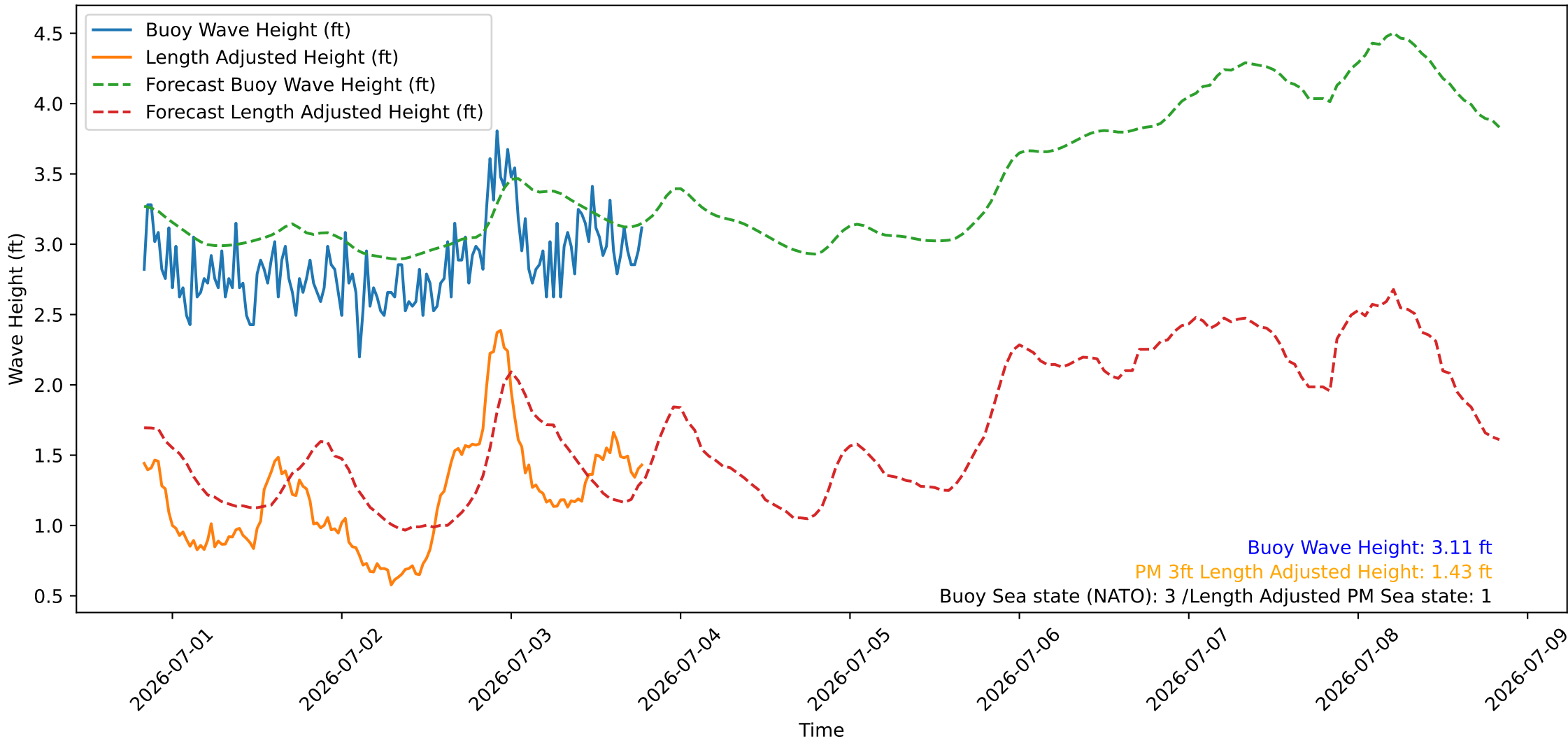
Wave Heights over Time for Red Beach at 2026-07-03 19:30:47
