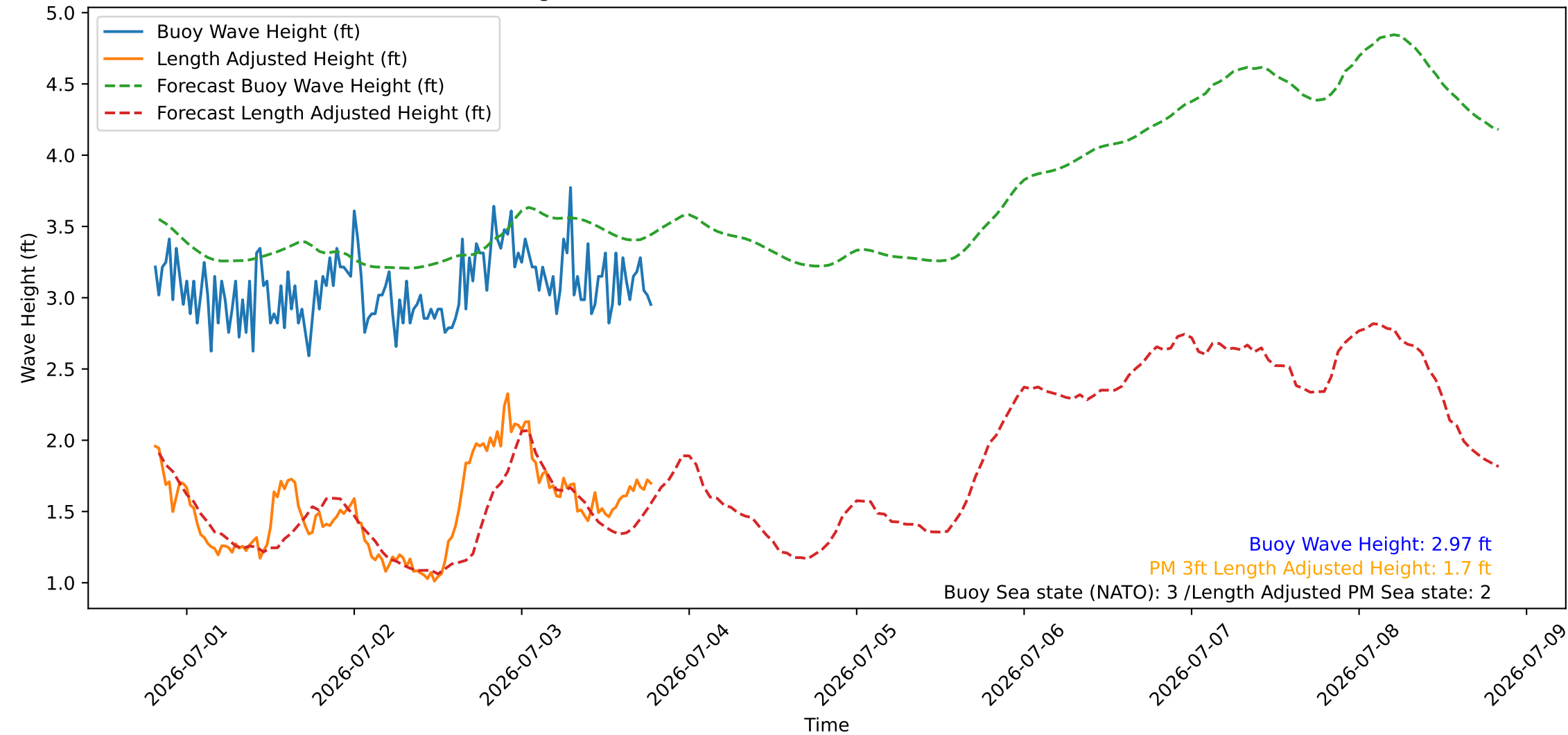
Wave Heights over Time for Oceanside Harbor at 2026-07-03 19:30:27
