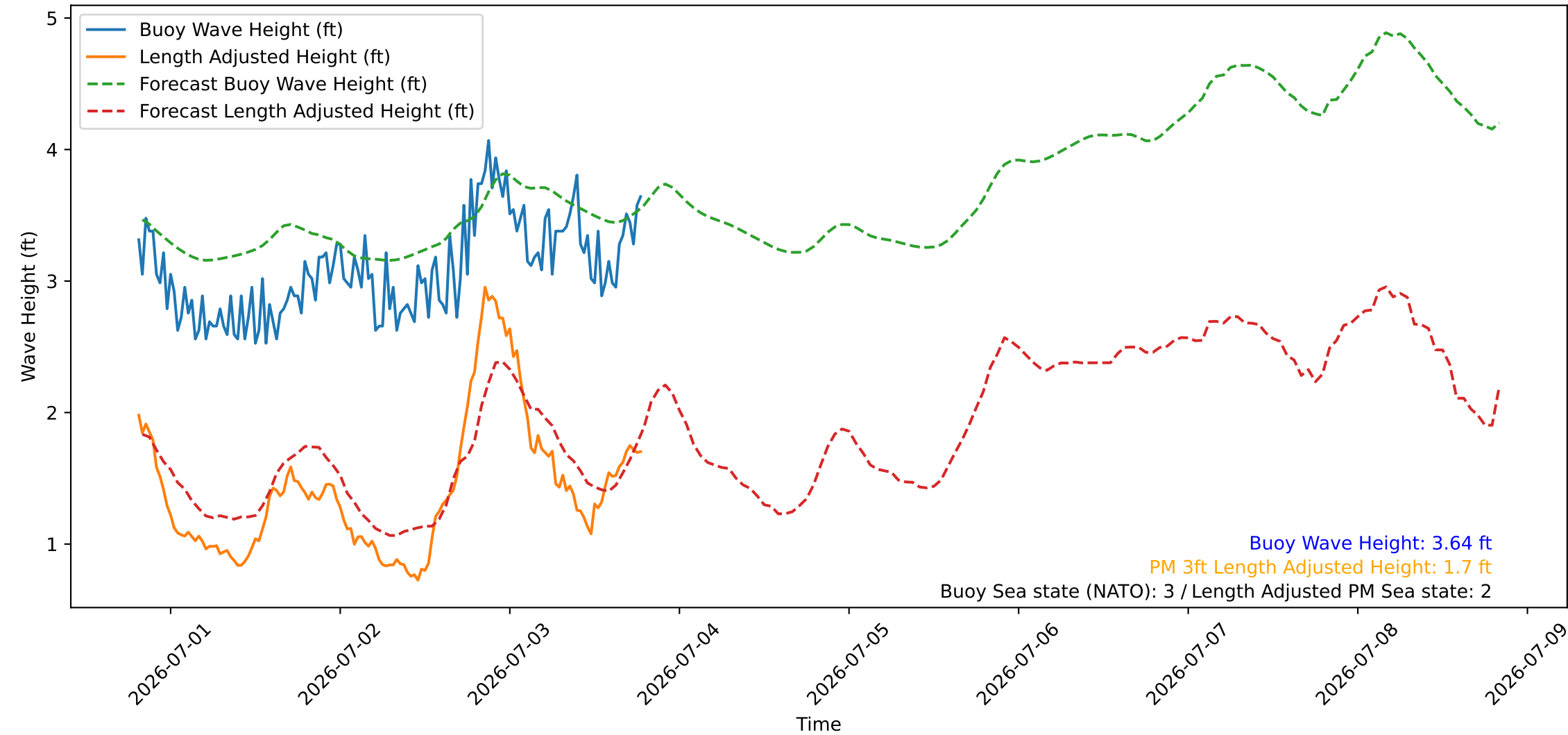
Wave Heights over Time for Green Beach at 2026-07-03 19:31:09
