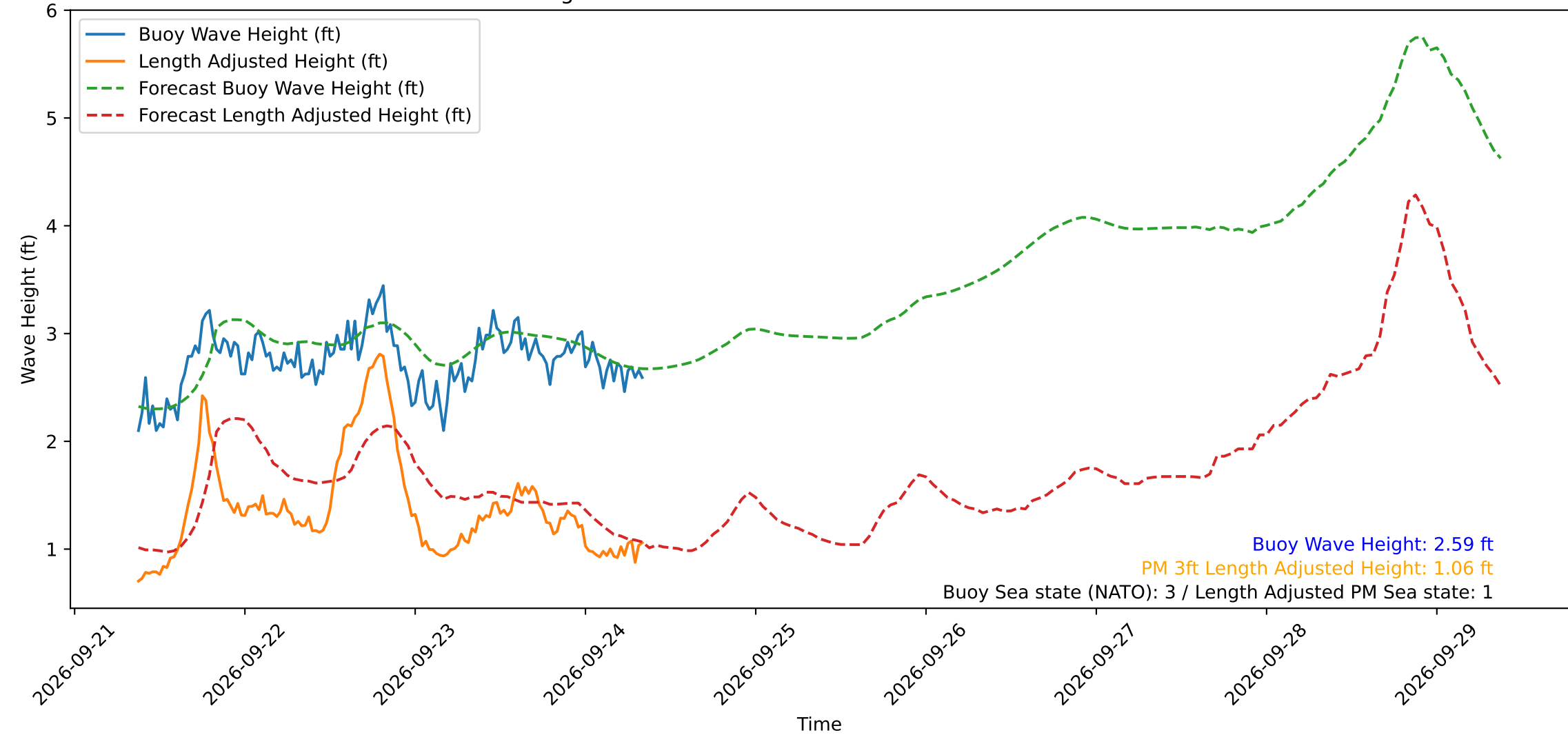
Wave Heights over Time for Green Beach at 2026-09-24 08:41:11
