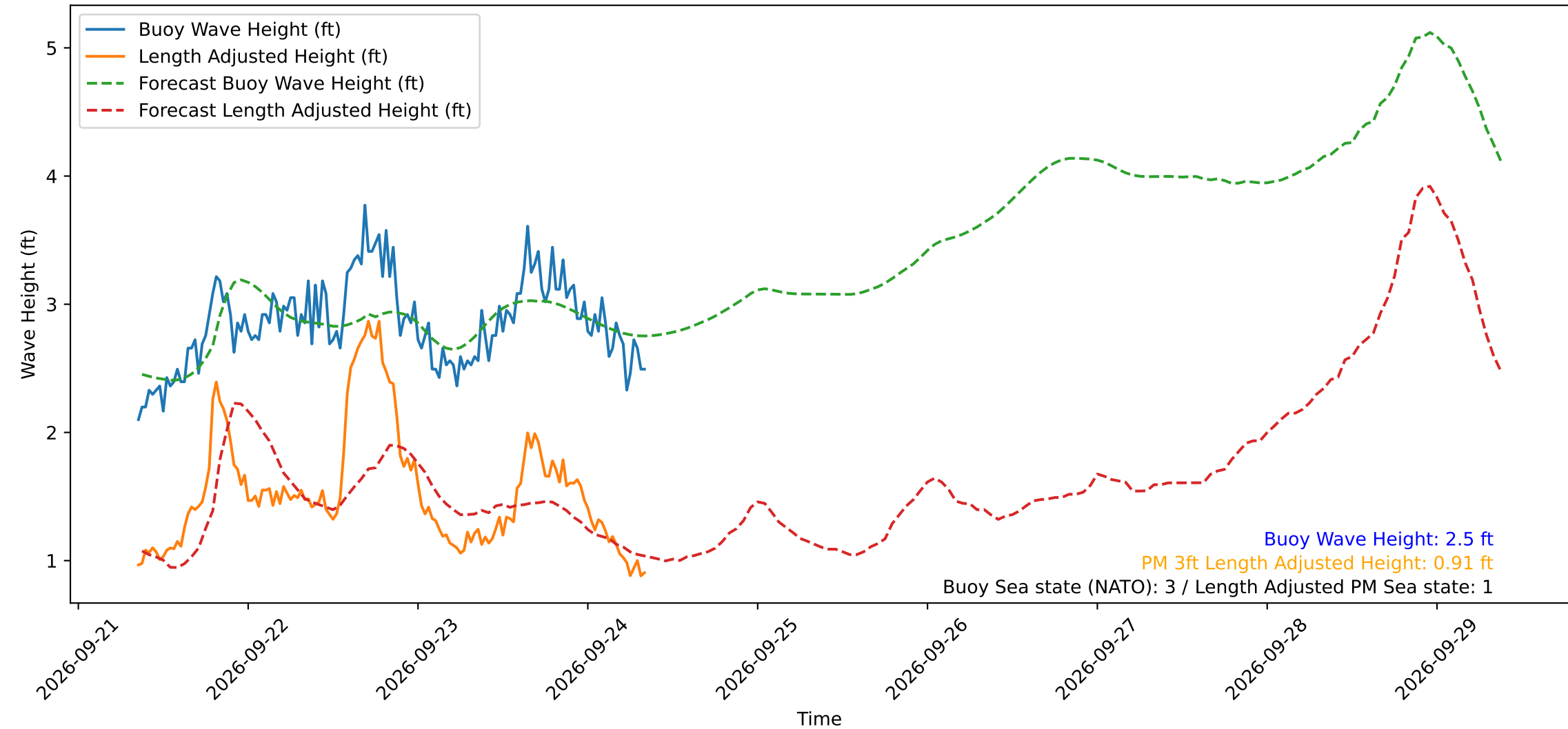
Wave Heights over Time for Oceanside Harbor at 2026-09-24 08:40:29
