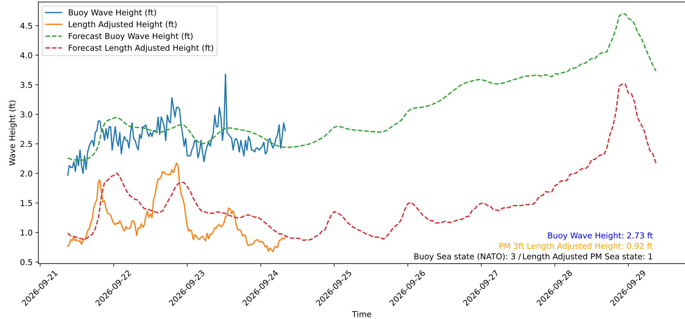
Wave Heights over Time for Red Beach at 2026-09-24 08:40:49
