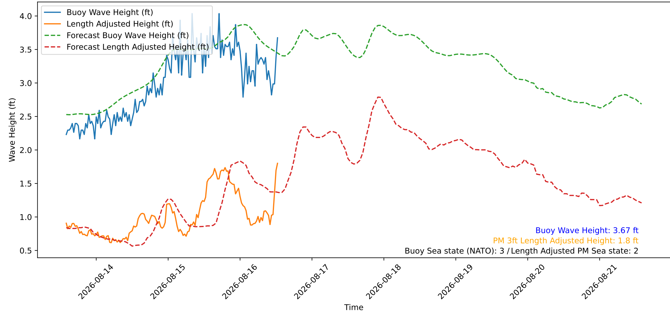
Wave Heights over Time for Red Beach at 2026-08-16 13:30:47
