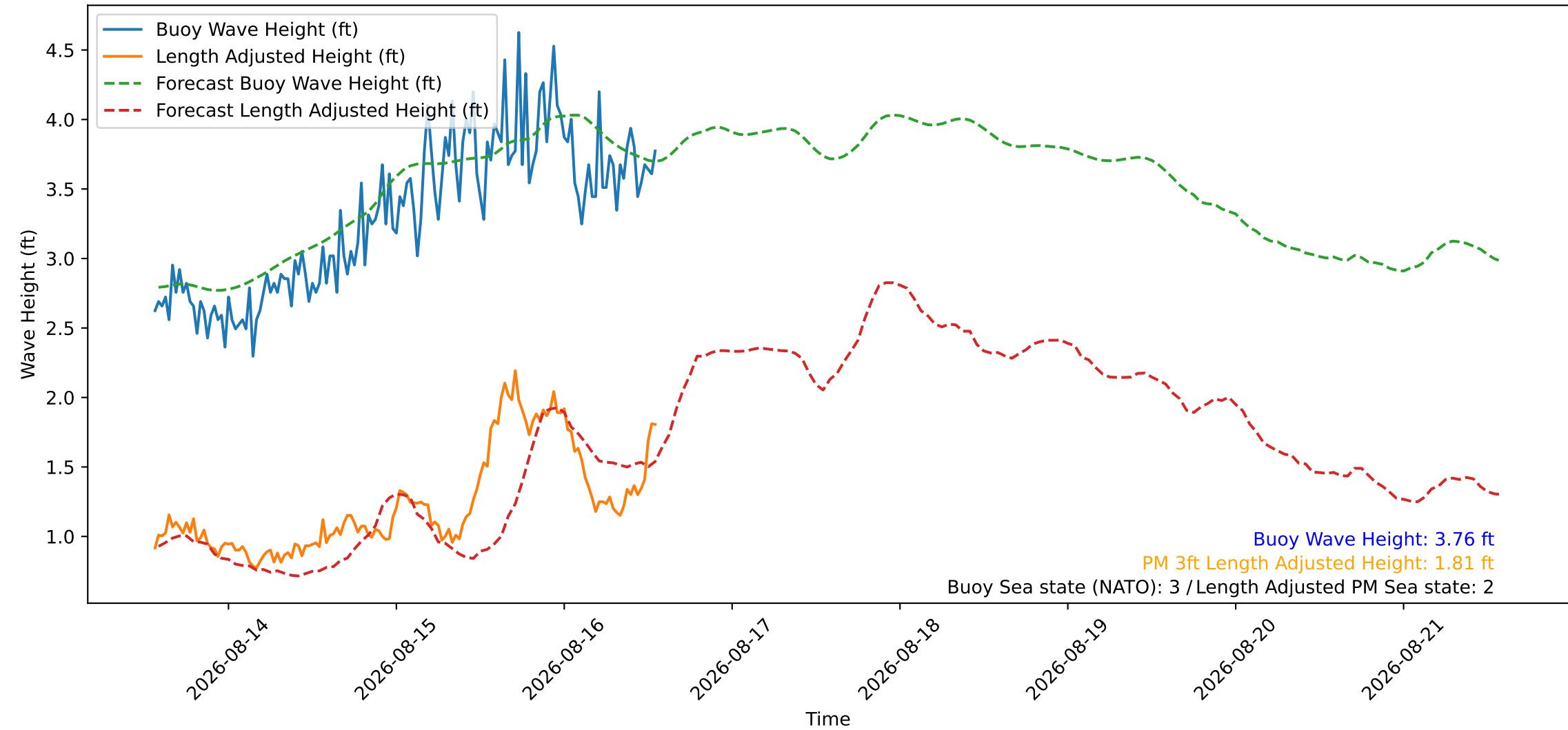
Wave Heights over Time for Oceanside Harbor at 2026-08-16 13:30:27
