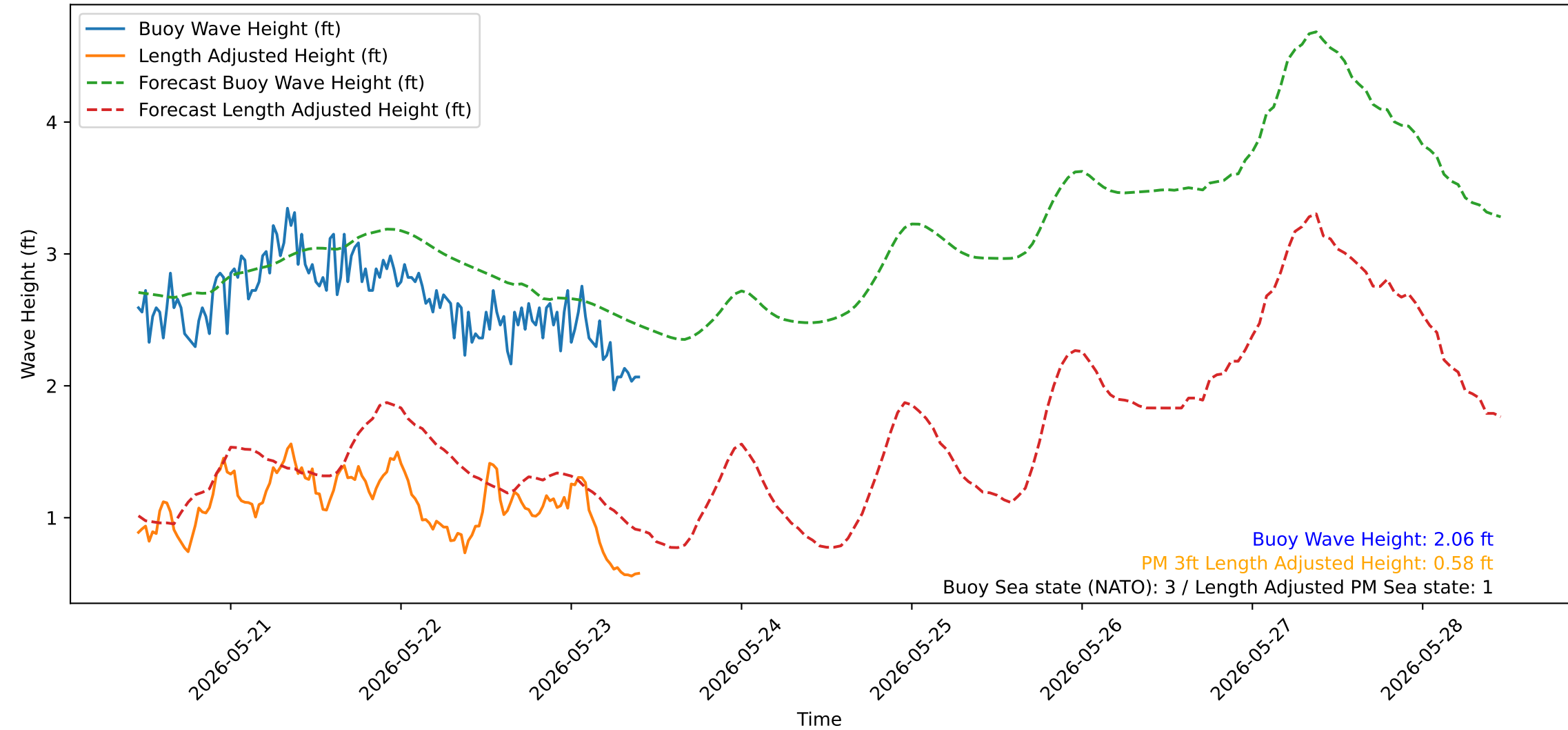
Wave Heights over Time for Red Beach at 2026-05-23 10:30:51
