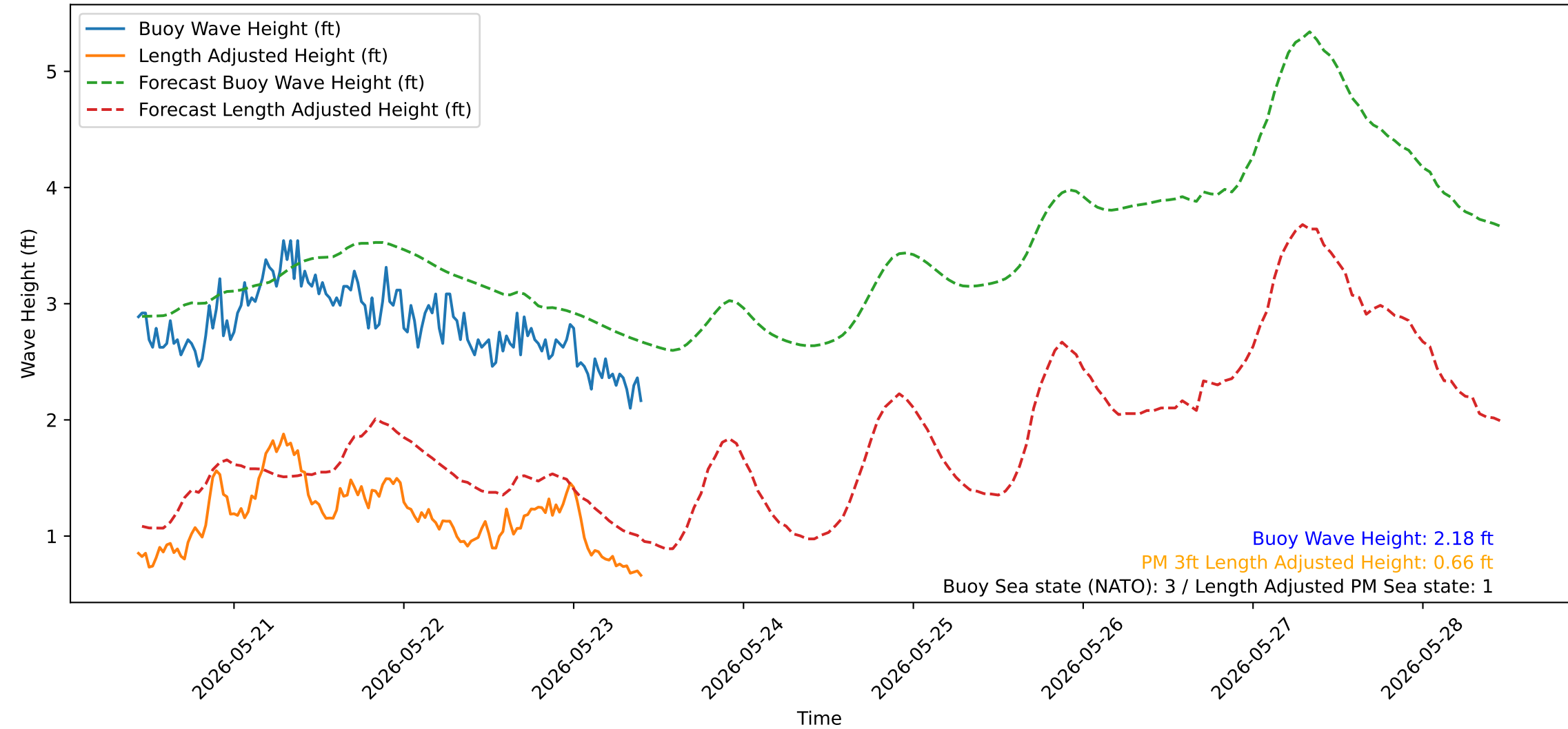
Wave Heights over Time for Green Beach at 2026-05-23 10:31:14
