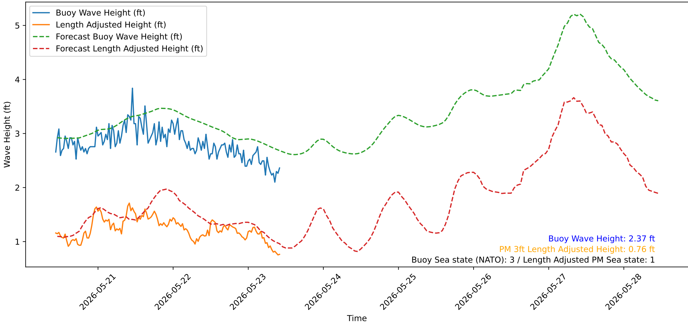
Wave Heights over Time for Oceanside Harbor at 2026-05-23 10:30:32
